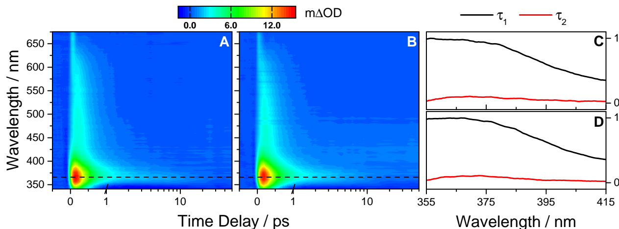
Fig. 2 (A) Raw TAS following 287 nm photoexcitation of OB-cyclohexane displaying an absorption peak at 366 nm (dashed line) and a broad absorption extending out to ~575 nm. The TAS for negative and early ( \leq 1 ps) time delays are shown on a linear scale, and longer time delays ( > 1 ps) are displayed on a logarithmic scale. The colour map indicates the change in optical density ( \Delta OD ). Similar observations are seen for OB-methanol (B). (C) and (D) The corresponding decay associated spectra for OB-cyclohexane and OB-methanol respectively from the bi-exponential global fit across the spectral range 355–415 nm returning a femtosecond lifetime \tau_1 and a picosecond lifetime \tau_2 , as summarised in Table 1.
