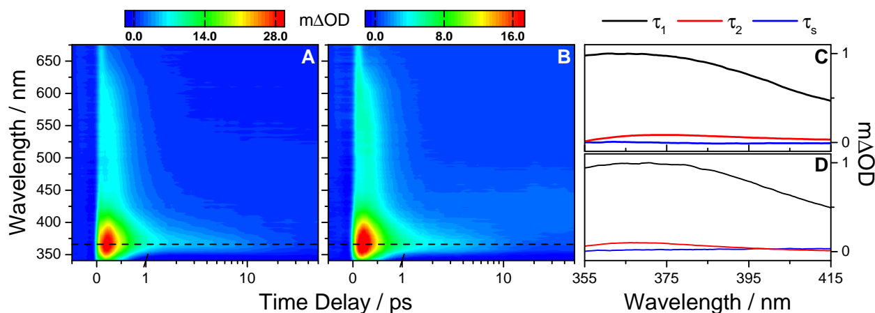
Fig. 3 (A) Raw TAS following 243 nm photoexcitation of OB-cyclohexane displaying an absorption peak at 366 nm (dashed line) and a broad absorption extending out to \sim 575 nm. The TAS for negative and early ( \leq 1 ps) time delays are shown on a linear scale, and longer time delays ( > 1 ps) are displayed on a logarithmic scale. Similar observations are seen for OB-methanol (B). (C) and (D) The corresponding decay associated spectra for OB-cyclohexane and OB-methanol respectively from the bi-exponential global fit across the spectral range 355–415 nm returning a femtosecond lifetime \tau_1 and a picosecond lifetime \tau_2 as summarised in Table 1, with a solvent dependant lifetime, \tau_s , which is \sim 400 ps for cyclohexane and \sim 3 ns for methanol. We note the small amplitude of \tau_s reflecting the minor contribution of this component to the DAS.
