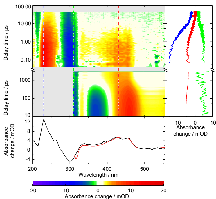
Figure 2: Spectrally and temporally resolved UV/Vis absorption spectra of photo-excited 1MP in water. The abscissa denotes the detection wavelength on a linear scale, the ordinate the time after photo-excitation on a logarithmic scale. The color table is chosen to display positive signals in a red hue and negative ones blue. White indicates zero and gray a lack of data. The femtosecond transient absorption data from time 1 ps up to 3.5 ns is taken from ref. 5 Two merged data sets from laser flash photolysis measurements complement the spectra up to 50 \mu s. The one from 40 ns to 1 \mu s with a time resolution of 20 ns, the other for longer delay times a time resolution of 100 ns. (right) Time traces for detection wavelengths of 230 nm (blue), 310 nm (green) and 430 nm (red) are given for the covered time window. (bottom) Decay associated spectra (DAS) from global data analysis of femtosecond transient absorption data (red) and laser flash photolysis (black). For direct comparison the flash photolysis data were scaled by 0.78.
