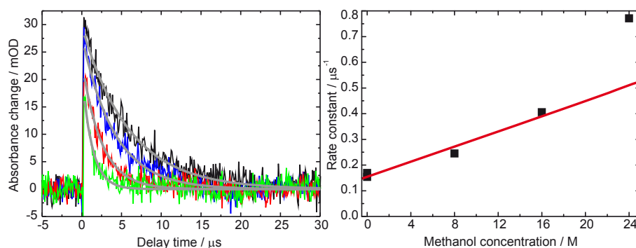
Figure 7: Impact of the MeOH concentration on the ^3\text{1MP}^* lifetime. (Left) Laser flash photolysis of 1MP in water (black), methanol (green) and methanol/water mixtures with a ratio of 1:2 (blue) and 2:1 (red). For all experiments the concentration of 1MP was around 100 \mu\text{M} . The detection wavelength was set to 430 nm. Exponential fits are given by gray lines. (Right) The rate constants derived from these fits are plotted in dependence on the methanol concentration (black squares). The red fit line illustrates the linearity. The last data point was excluded from the linear fit, see text.
