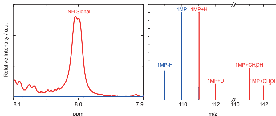
Figure 6: Determination of the chemical motifs present in the photo-product of 1MP in methanol. Measurements of 1MP are colored blue, those of the photoproduct red. (left) The product displays a broad signal around 8 ppm in the NMR spectrum. (right) The mass spectrum of the product exhibits strong peaks at \frac{m}{z} = 111 (1MP+H) and \frac{m}{z} = 141 (1MP+CH 2 OH). Slightly weaker ones at \frac{m}{z} = 112 (1MP+D) and \frac{m}{z} = 142 (1MP+CH 3 OH).
