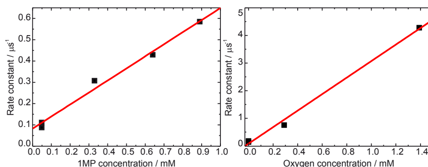
Figure 3: Rate constants for the triplet decay of 1MP. Rate constants are determined from exponential fits to time traces at a detection wavelength of 430 nm (points). A linear fit to that data (lines) yields the corresponding quenching rate constants. (left) Concentration dependence of the triplet decay in de-oxygenated solutions. (right) Quenching by molecular oxygen at a 1MP concentration of 75 \mu\text{M} .
