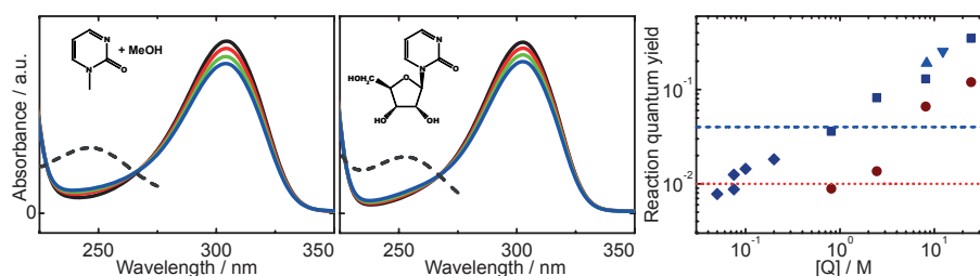
Figure 4: Representative spectral changes resulting from illumination of IMP in methanol (left) and zebularine in water (middle) as well as quantum yields derived from these changes (right). Subsequent illumination steps correspond to a light dose of \sim 1 photon per molecule. The product spectra obtained by extrapolation to complete consumption are given by dashed lines. A compilation of reaction quantum yields for different quencher concentrations is found on the right (log-log plot). Blue points depict values derived for nitrogen-purged solutions, red ones for air-saturated solutions. Values are given for methanol (squares), THF (triangles) and \beta -D-ribose (diamonds). The horizontal dashed lines specify the reaction quantum yields of zebularine in nitrogen-purged (blue) and air-saturated (red) aqueous solution.
