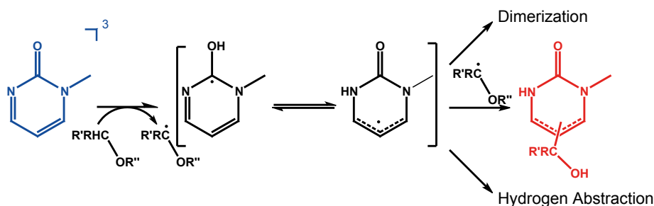
Figure 5: Scheme summarizing HA by ^3\text{1MP}^* . 1MP in the triplet state abstracts a hydrogen atom from the quencher bearing a -CRH-O- chemical motif. The so formed radical can tautomerize forming a N-H group. Recombination with the quencher radical terminates the reaction chain. For high concentrations also dimerization could occur.
