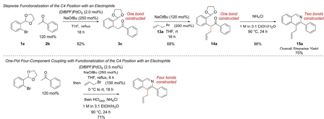
Scheme 7: Development of Four-Component One-Pot Coupling (double column)
