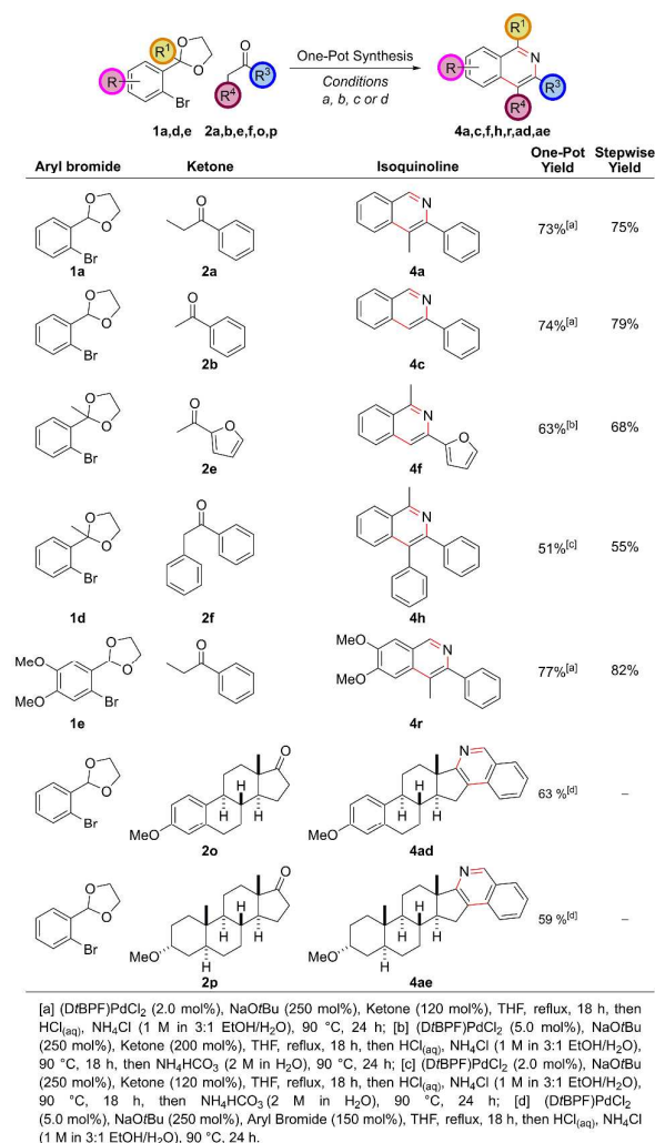
Figure 4: One-pot Synthesis of Isoquinolines (single column)
