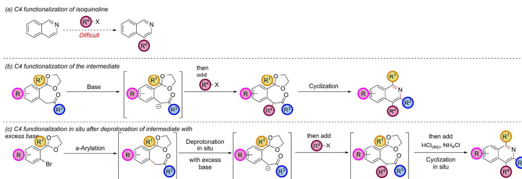
Scheme 6: Functionalization of the C4 Position (double column)
