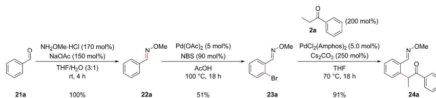
Scheme 9: C–H Functionalization Allowing Benzaldehyde Derivatives to be Incorporated into the Synthetic Route (double column)
