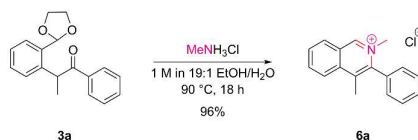
Scheme 4: Synthesis of Isoquinolinium Salt 6a (single column)
