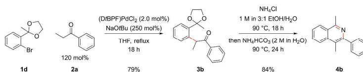
Scheme 3: Optimized \alpha -Arylation and Cyclization Conditions for R_1 \neq H (double column)
