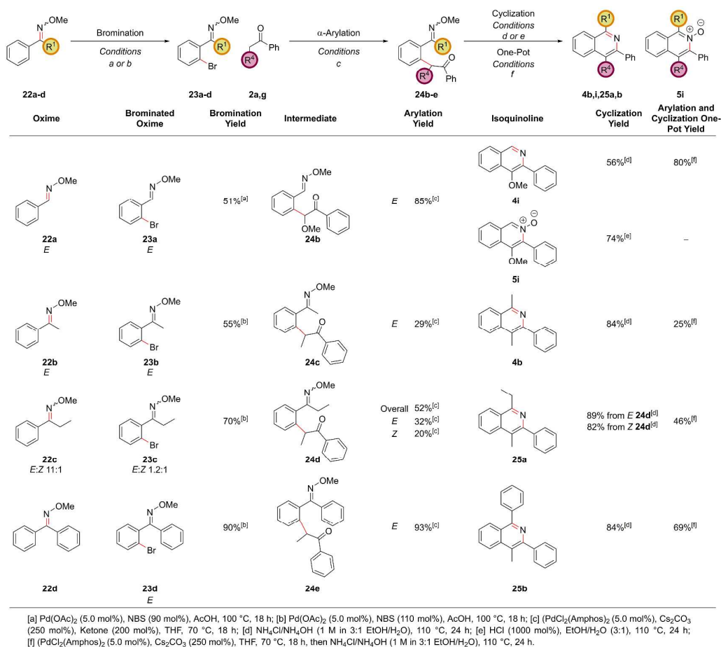
Figure 11: C–H Bromination Route to Isoquinolines (double column)
