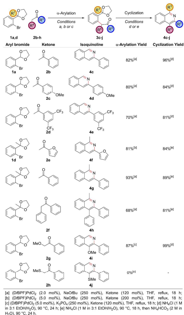
Figure 1: Exploring the Scope with Aryl Ketones (single column)
