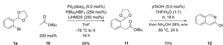
Scheme 5: \alpha -Arylation and Cyclization of Ester Enolates (double column)
