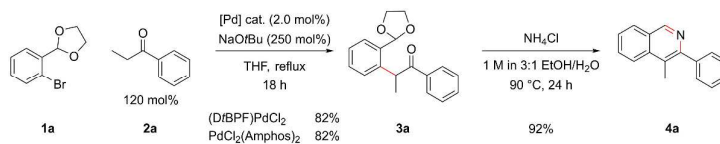
Scheme 2: Optimized \alpha -arylation and Cyclization Conditions for R_1 = H (double column)
