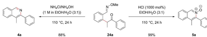
Scheme 10: Cyclization of Oxime 24a to Both Isoquinoline 4a and Isoquinoline N -oxide 5a (double column)
