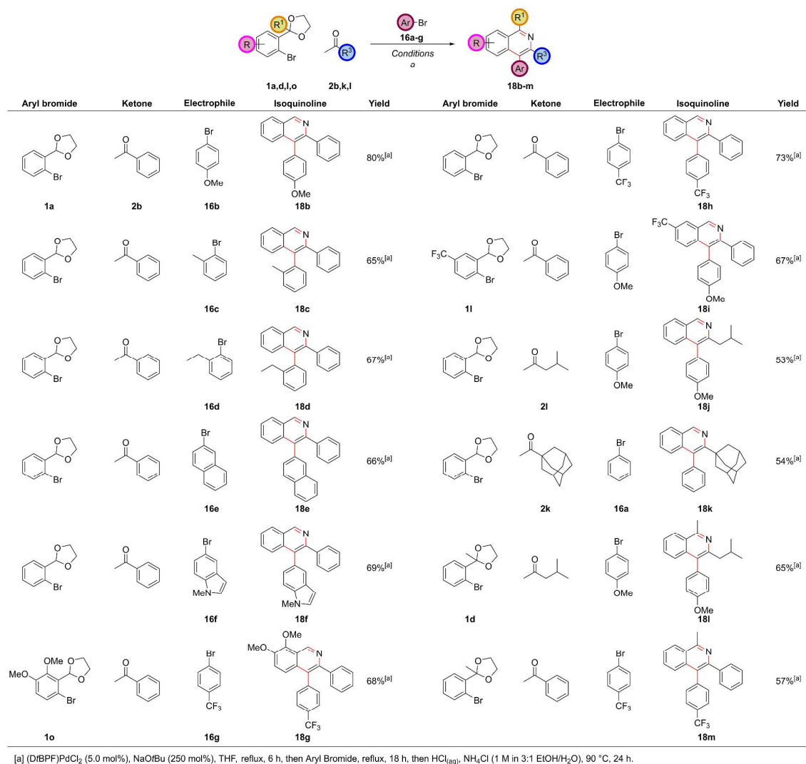
Figure 9: Scope of Four-Component Coupling Procedure with Two Aryl Bromides (double column)
