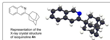
Figure 2: Exploring the Scope with Alkyl Ketones (single column)
