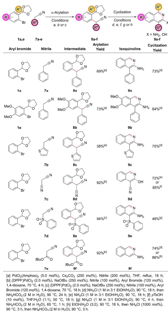
Figure 6: Access to 3-Amino and 3-Hydroxyisoquinolines (single column)
