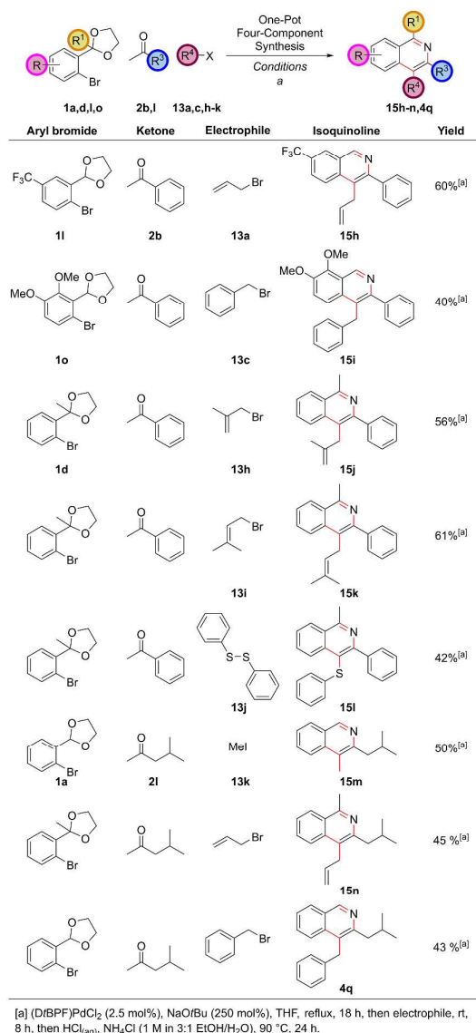
Figure 8: Further Exemplification of the One-Pot Four-Component Coupling Procedure (single column)
