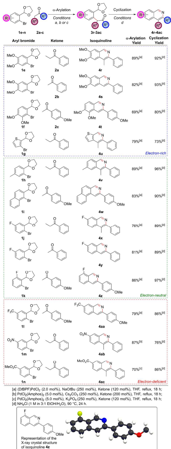
Figure 3: Exploring the Scope of the Aryl Bromide Partner (single column)
