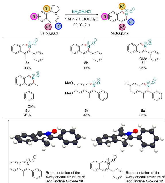
Figure 5: Synthesis of Isoquinoline N -oxides (single column)
