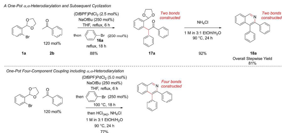
Scheme 8: Development of One-Pot Diarylation (double column)
