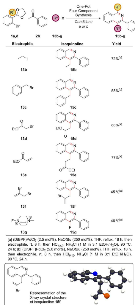
Figure 7: One-Pot Four-Component Coupling Procedure (single column)
