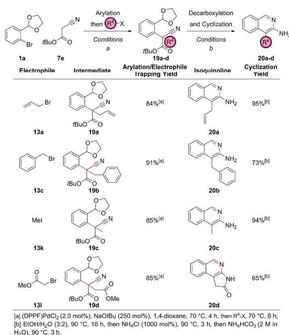
Figure 10: \alpha -Arylation and Functionalization of tert -Butyl Cyanoacetate (single column)
