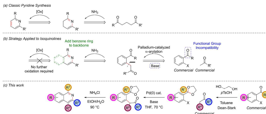
Scheme 1: Retrosynthetic Strategy for Isoquinolines (double column)
