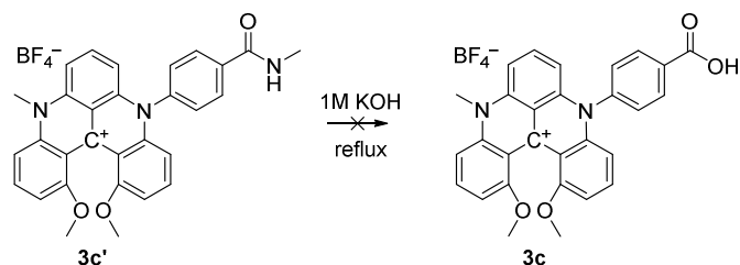
Scheme 2. Hydrolysis of DMQA amide 3c' .
