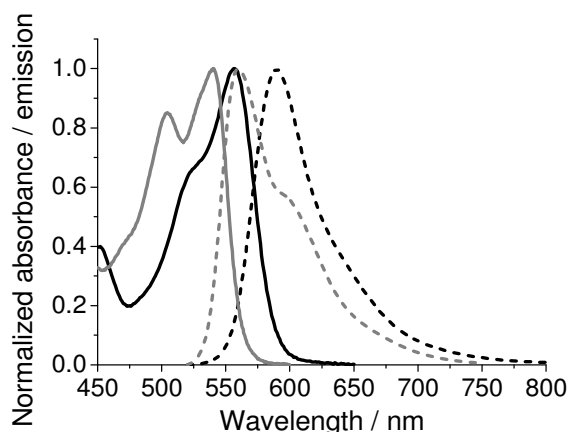
Figure 1. Absorption (full) and emission (dashed) spectra of ADOTA 4c (grey) and DAOTA 5c (black) measured in acetonitrile solution.
