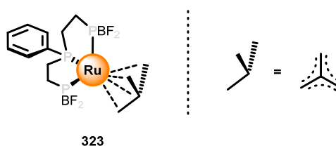
Figure 38. Molecular structure of Ru complex 323 .
