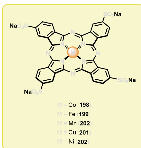
Figure 23. Water soluble metallophthalocyanines ( 198–202 ) employed for studying oxidative conversion of lignin model systems.
