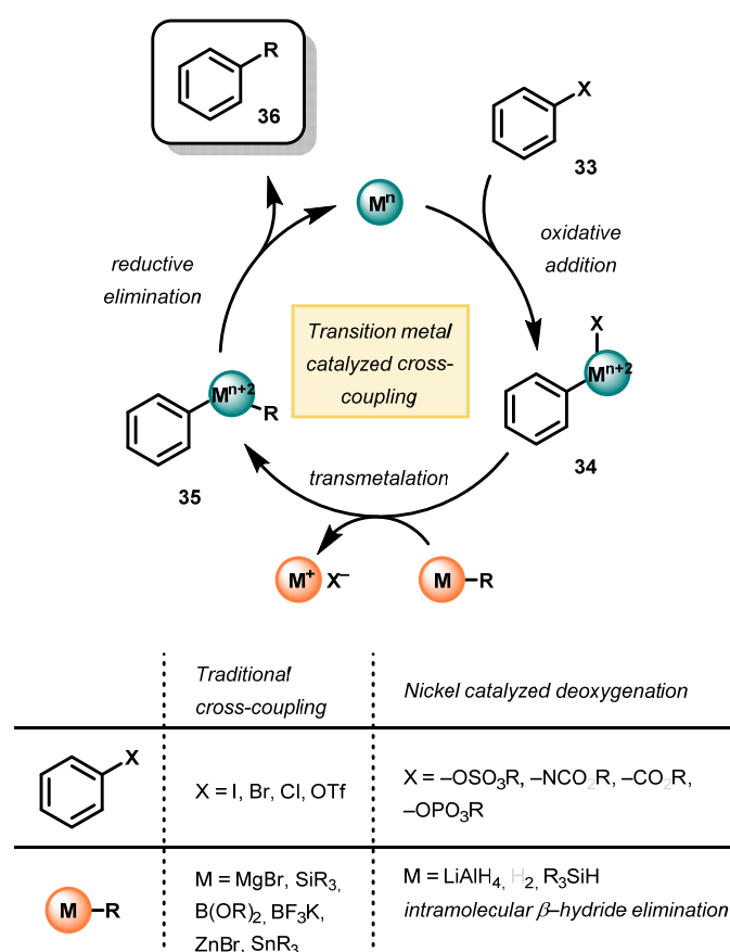
Figure 8. Comparison of traditional cross-coupling methodology and Ni-catalyzed arene deoxygenation.
