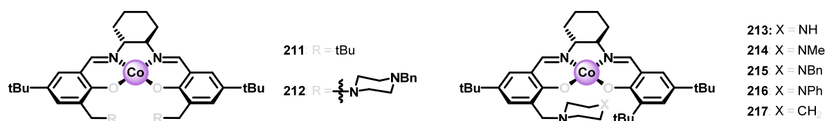
Figure 26. Symmetrical ( 211 and 212 ) and unsymmetrical ( 213–217 ) Co-Schiff base complexes developed for studying the oxidative conversion of lignin models.
