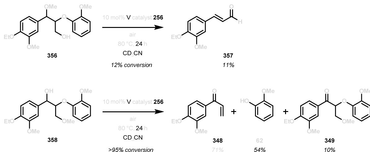
Scheme 36. Reactivity study of V complex 256 .
