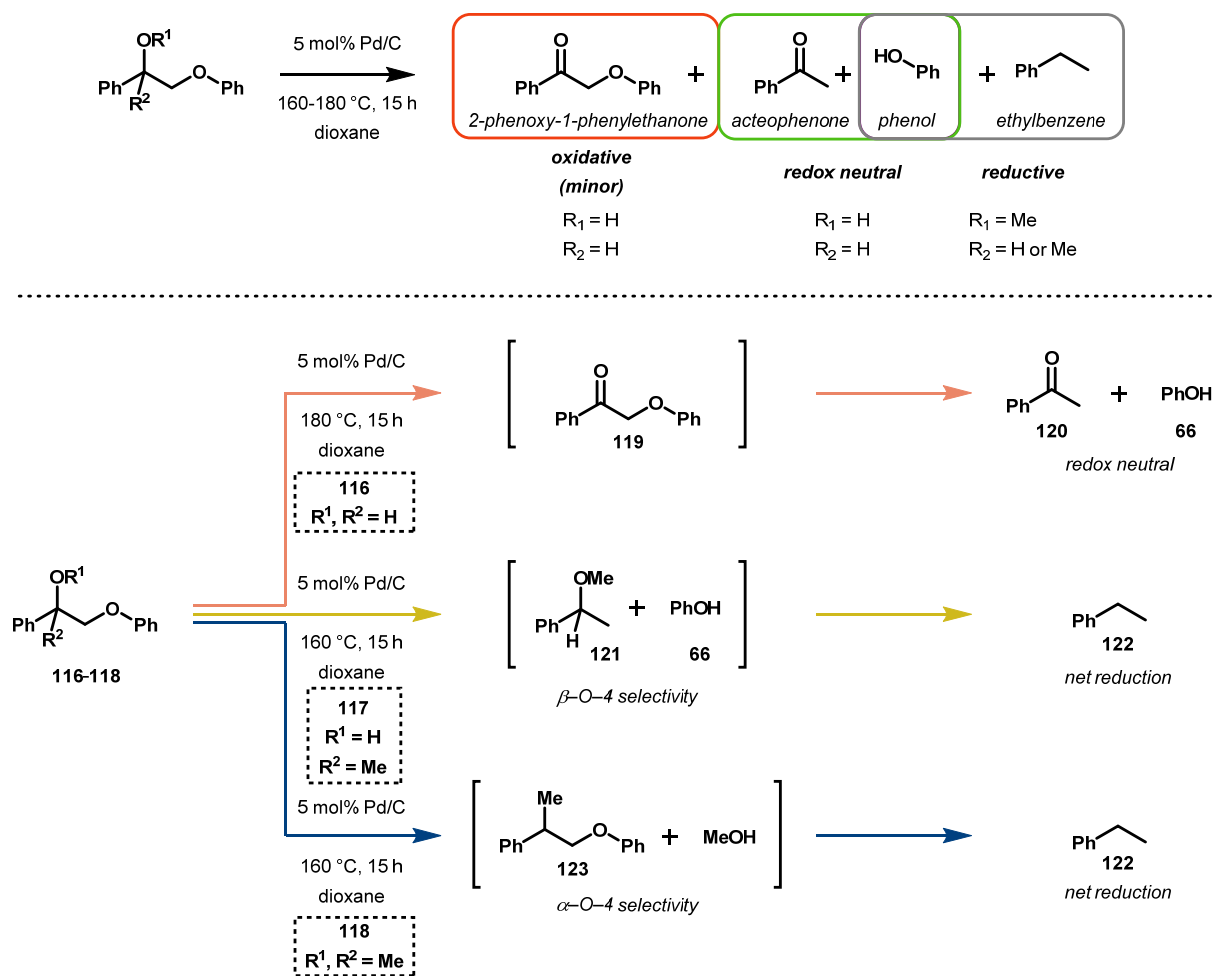
Figure 17. Pd/C catalyzed C–O bond cleavage using dioxane as hydrogen source.
