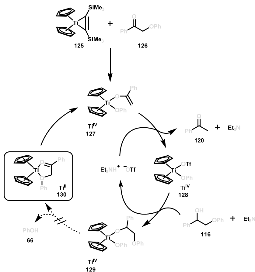
Scheme 7. Titanium catalyzed C–O bond cleavage.
