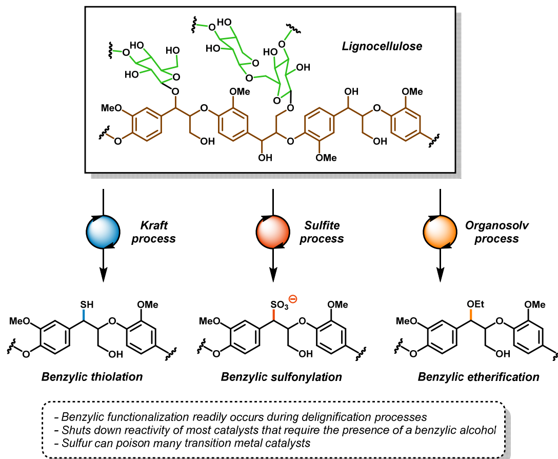
Figure 4. The lignin pulping processes.
