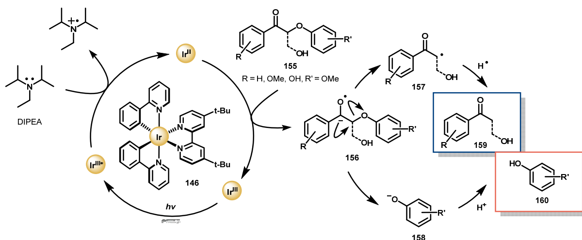
Scheme 9. Proposed mechanism for the photocatalytic reductive cleavage of oxidized lignin model systems.
