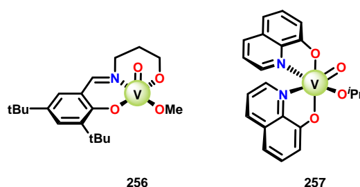
Figure 29. (a) Previously reported V catalyst 256 that mediates C–O bond cleavage of non-phenolic lignin models and (b) the previously reported 8-quinolinate-based V catalyst 257 ( V^V(HQ)_2(O)(O^iPr) ) that promotes C–H bond cleavage products of non-phenolic lignin model systems.
