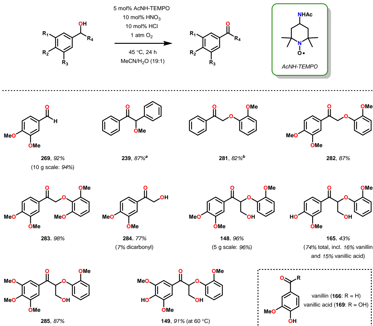
Figure 33. Metal-free aerobic oxidation of lignin models using the AcNH-TEMPO/HNO 3 /HCl catalyst system. Reaction conditions: 1 mmol of alcohol (0.2 M in MeCN/H 2 O 19:1). a 10 mol% AcNH-TEMPO, 36 h. b Yield after 36 h.
