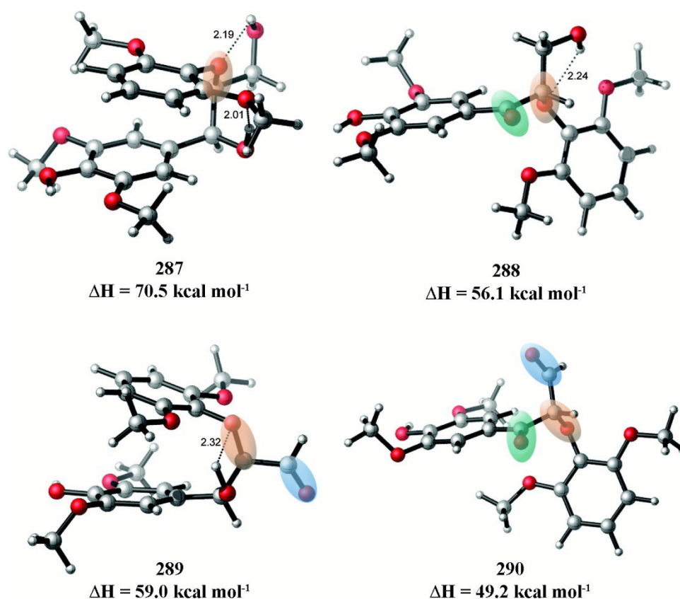
Figure 35. Comparison of \beta -O-4 in a native lignin model compound ( 287 ) and \beta -O-4 in various oxidized systems ( 288–290 ) for C–O bond cleavage at the \beta -position. Bond lengths are given in Å.
