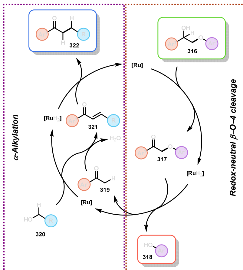
Scheme 33. Plausible mechanism for the sequential \beta\text{-O-4} cleavage/ \alpha -alkylation of lignin model compounds.
