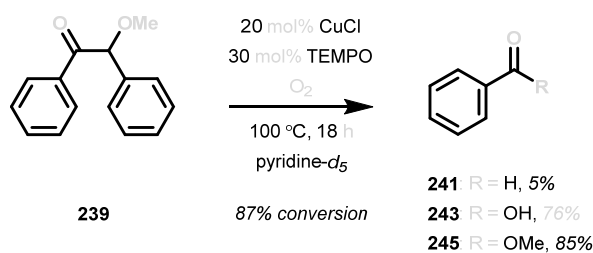
Scheme 23. CuCl/TEMPO catalyzed oxidation of benzoin methyl ether ( 239 ).
