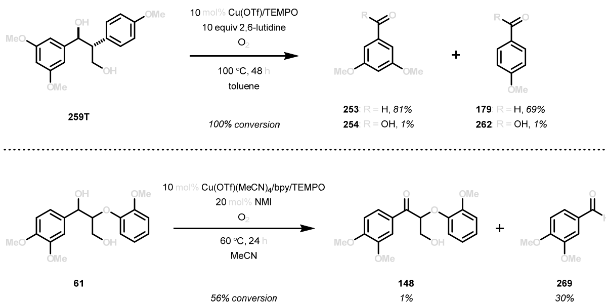
Scheme 25. (Top) Oxidation of the non-phenolic lignin model 259T with the Cu(OTf)/2,6-lutidine/TEMPO system. (Bottom) Oxidation of non-phenolic lignin model 61 with the Cu(OTf)(MeCN) 4 /bpy/TEMPO/NMI system.
