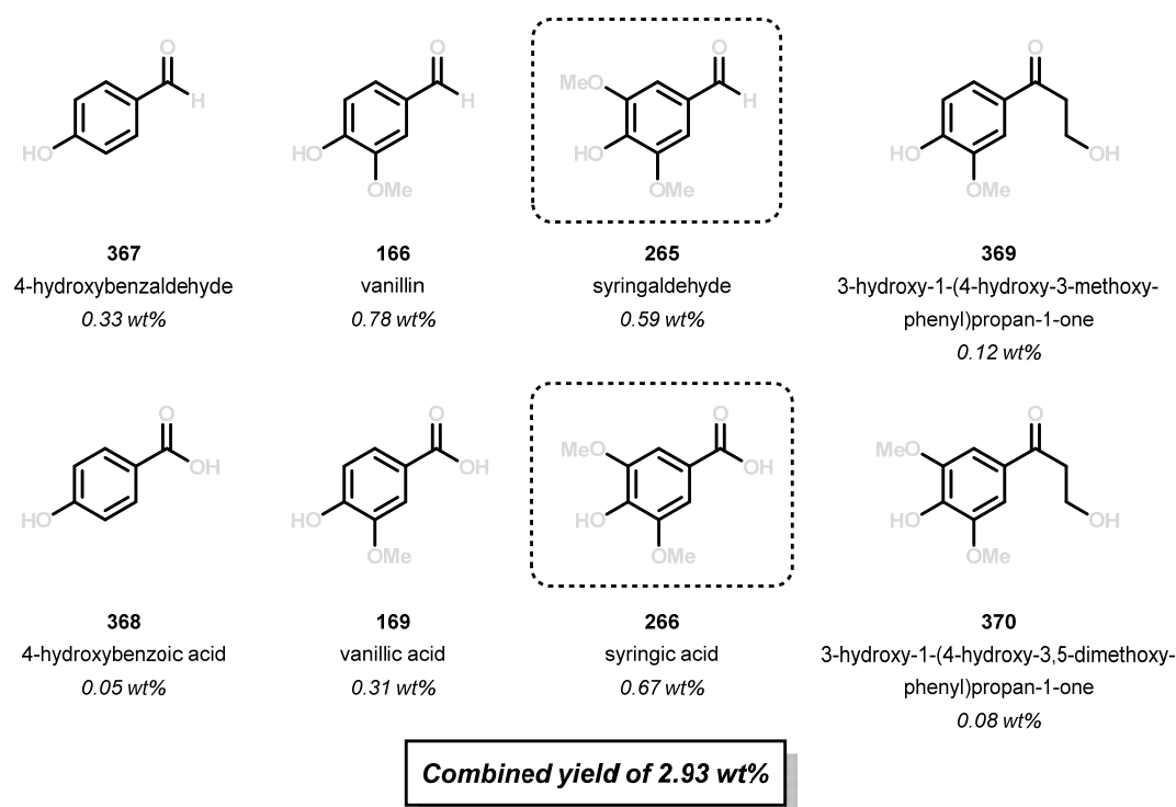
Figure 39. Identity and yield of products from V-catalyzed degradation of dioxasolv lignin derived from Miscanthus giganteus .
