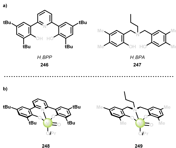
Figure 28. Structure of (a) ligands H 2 BPP ( 246 ) and H 2 BPA ( 247 ), and (b) the corresponding V complexes ( 248 and 249 ).
