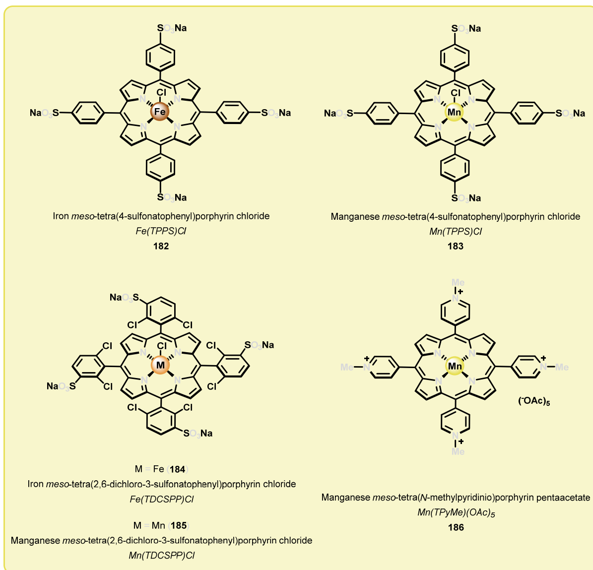
Figure 21. Water soluble porphyrin complexes 182–186 employed for degradation of lignin model systems.
