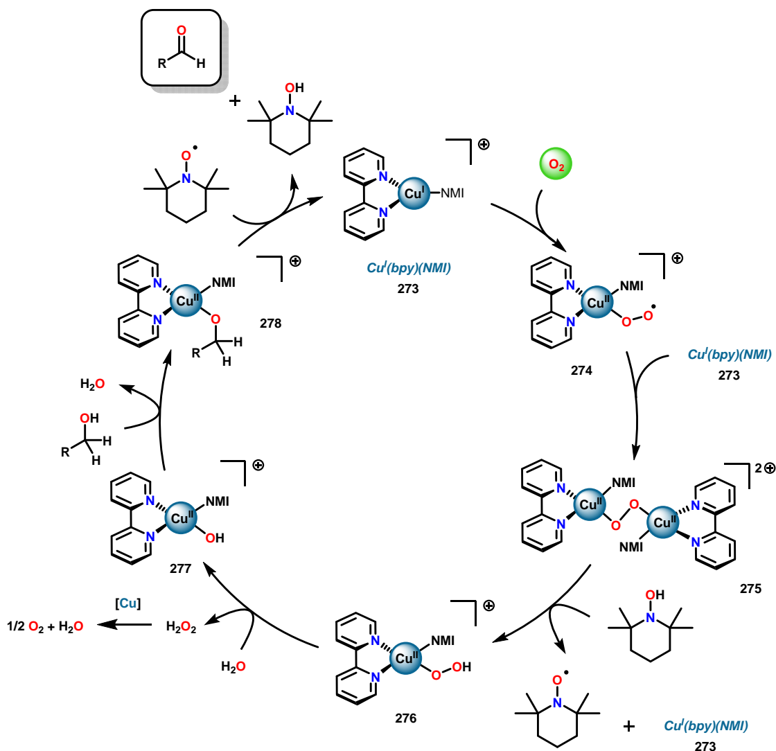
Figure 31. Proposed mechanism for catalytic \text{Cu}^{\text{I}} /TEMPO mediated oxidation of alcohols. NMI = N -methylimidazole. R = alkyl, aryl.
