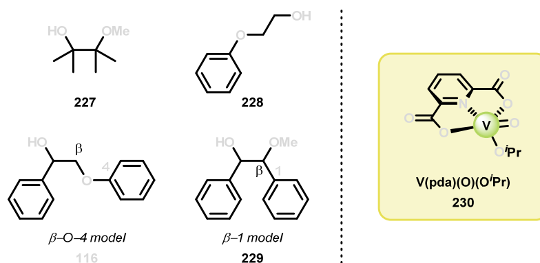
Figure 27. (Left) Model systems 116 and 227–229 and (right) V complex 230 .
