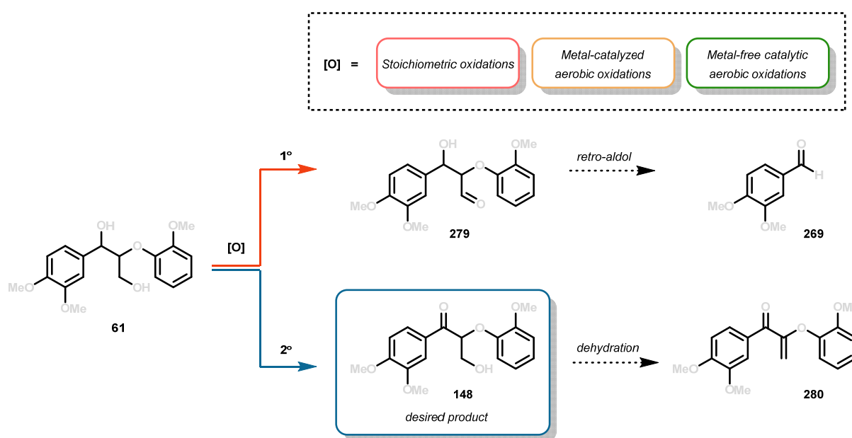
Figure 32. Possible product distribution for oxidation of lignin model system 61 by TEMPO-based catalytic protocols.
