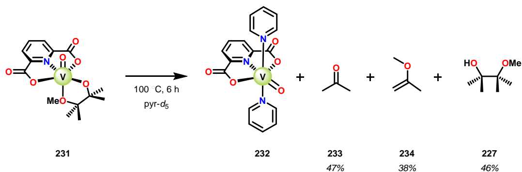
Scheme 16. Stoichiometric C–C bond cleavage by V complex 231 .
