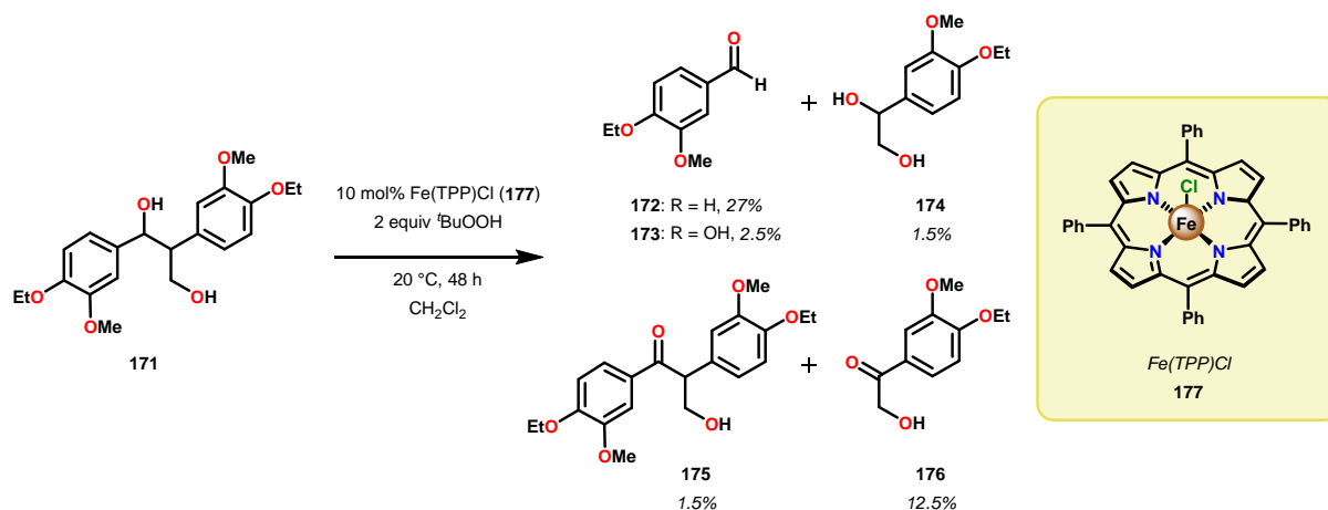
Scheme 11. Oxidation of lignin model system 171 by \text{Fe(TPP)Cl} ( 177 ).
