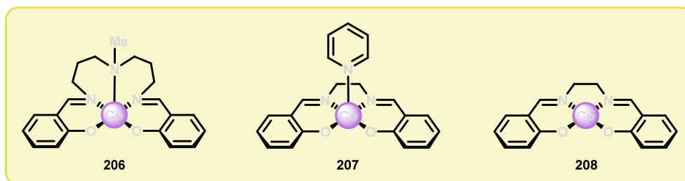
Figure 25. Co-Schiff base complexes used for oxidative degradation of lignin model systems.
