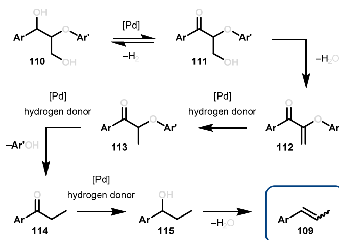
Figure 16. (Top) Pd/C catalyzed tandem organosolv transfer hydrogenolysis (TOH) of birch wood and (bottom) proposed mechanism of aryl propene formation.
