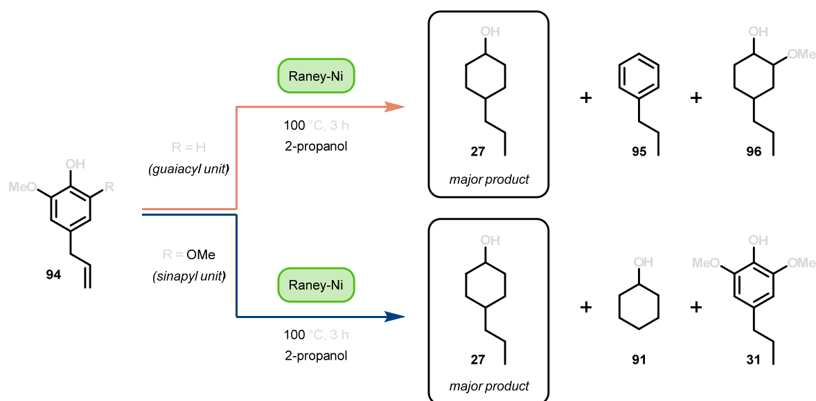
Figure 14. Raney-Ni catalyzed transfer hydrogenation of lignin model substrates.
