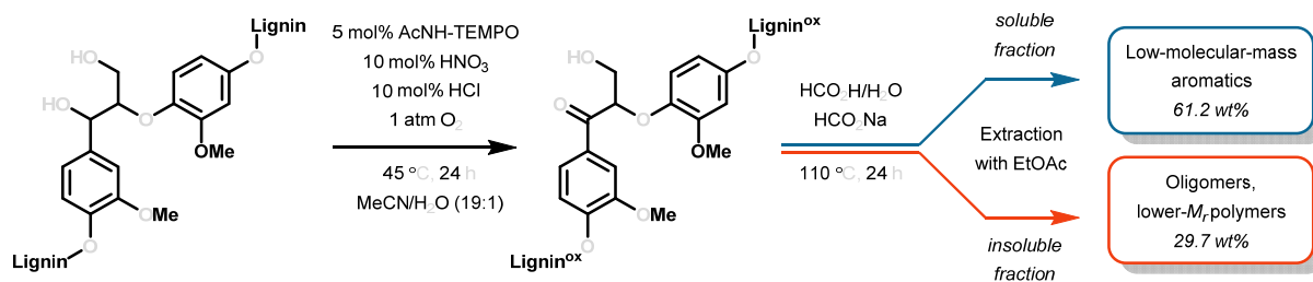
Scheme 29. Two-step approach for depolymerization of aspen lignin.
