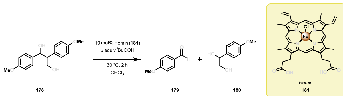
Scheme 12. Oxidative \text{C}_\alpha\text{-C}_\beta bond cleavage of lignin model system 178 by hemin 181 .
