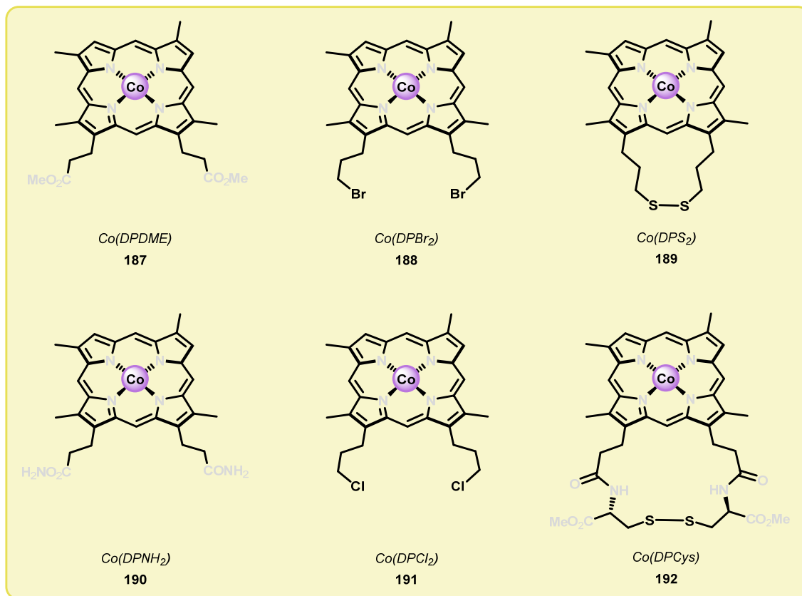
Figure 22. Structure of Co deuteroporphyrins 187–192 .
