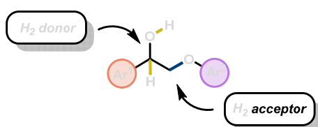
Figure 34. Principle for redox-neutral conversion of lignin and lignin model systems.
