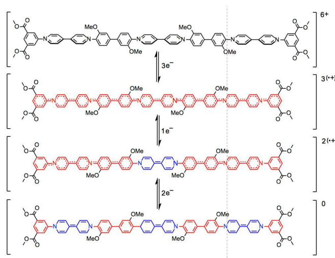
Scheme 3 The structures of the stable intermediates observed during the electrochemical interconversions of trimer 3 : tris(dicationic), tris(radical cationic), di(radical cationic) and neutral, quinoidal forms (top to bottom respectively).
