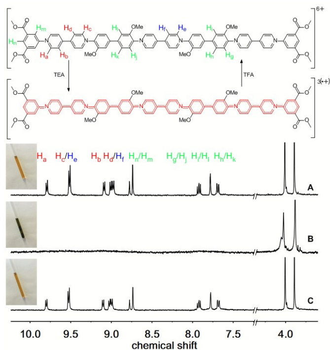
Fig. 2 Chemical reduction (3 × one-electron) and reoxidation of trimer 3 using TEA and TFA, respectively. The aromatic and heterocyclic rings highlighted in red indicate the region of unpaired spin density (not bond order). ^1\text{H} NMR spectra and photographs of the samples: (A) trimer 3 in acetone- d_6 , (B) after addition of 20 equivs of TEA and (C) subsequent to addition of an excess of TFA to B.
