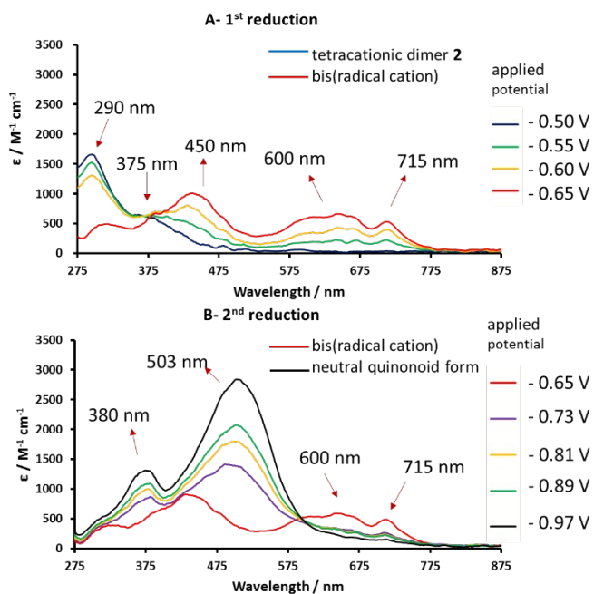
Fig. 6 Reversible UV-vis spectral changes accompanying the stepwise 1e - reduction of tetracationic dimer 2 to the corresponding bis(radical cation) (spectrum A) and the neutral quinonoid form (spectrum B). Spectra recorded in anhydrous DMF/0.1M TBAPF 6 , using an OTTLE cell. 67
