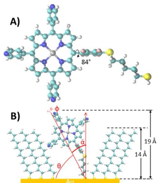
Figure 27 A. Porphyrin molecule with thiol tether (optimized structure from DFT calculations) (Zn or H 2 is grey, carbon is aqua blue, hydrogen is white, nitrogen is blue, fluorine is pink, and sulphur is yellow). B. Scheme showing geometry of thioalkyl substituted porphyrin inserting between alkanethiols. see ref. 50, 177. Reproduced with permission from ref 50. Copyright 2015 American Chemical Society
