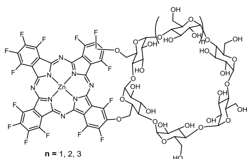
Figure 19 Amphiphilic cyclodextrin-Pc conjugates, see ref. 116.
