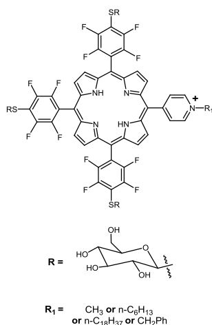
Figure 3 Thioglycosylated cationic porphyrin, see ref. 75
