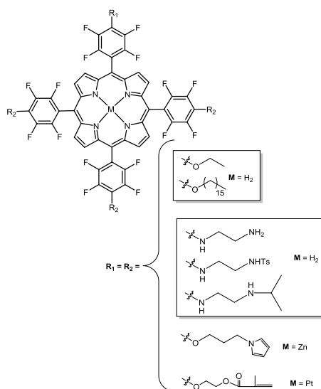
Figure 23 Symmetric metallated and free base oxy and amino substituted porphyrin for applications as sensors, see ref. 35, 38, 128, 152.
