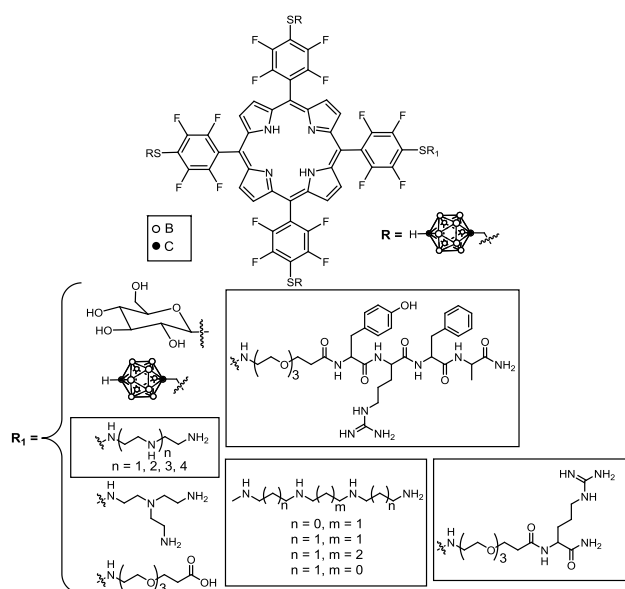
Figure 12 Asymmetrical carborane-porphyrin conjugates for BNCT, see ref. 41, 46.
