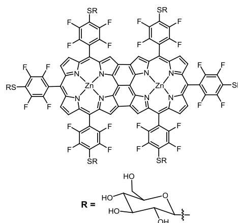
Figure 20 Hexathioglucose triply bridged fused porphyrin, see ref. 47.
