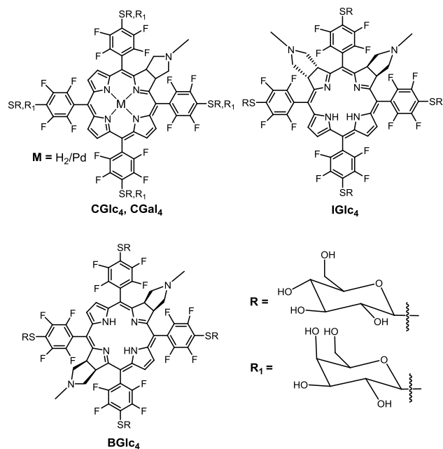
Figure 14 Pd and free base CGlc 4 , free base CGal 4 , free base IGlc 4 , and free base BGlc 4 . See ref. 91, 92, 94.
