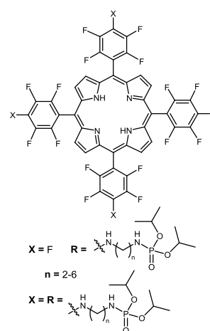
Figure 10 Porphyrin-phosphoramidateconjugates, see ref. 83.
