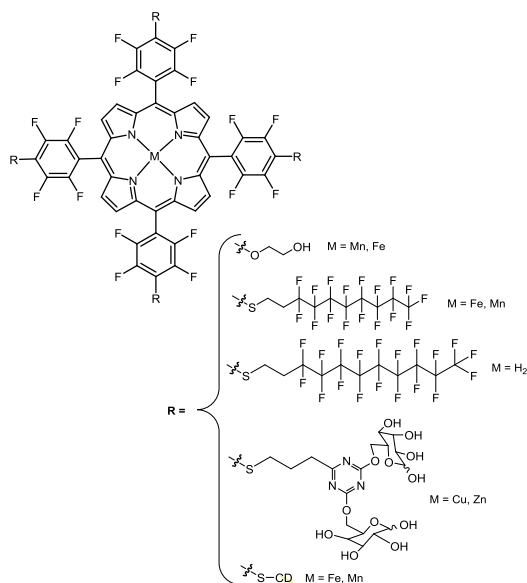
Figure 21 Tetra substituted metallated and non-metallated porphyrin thio and oxy derivatives, see ref. 52, 53, 120, 121, 122, 124, 125.
