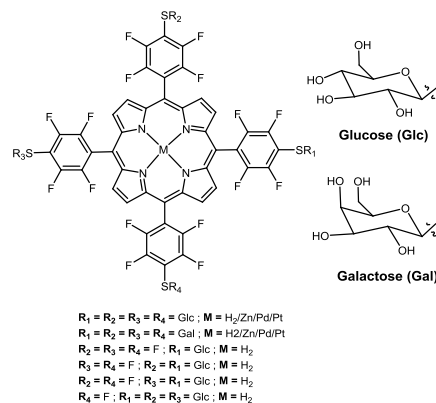
Figure 4 Metallated and non-metallated S-sugar-porphyrins, see ref. 33, 76, 77.
