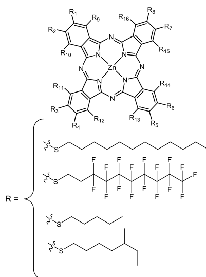
Figure 24 Thio substituted phthalocyanines, see ref. 48, 49, 126.
