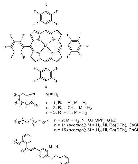
Figure 7 Symmetricmetallated and metal free glycol porphyrins and free base chalcone porphyrin derivatives, see ref. 45, 80, 81.
