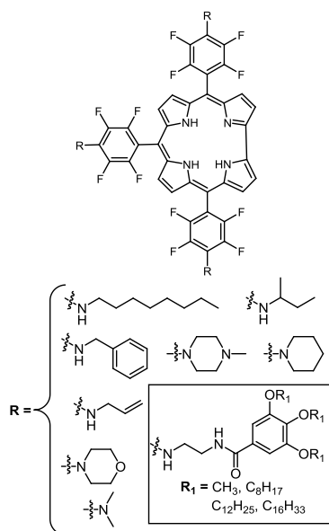
Figure 16 Mono and tri amino substituted corrole derivatives, see ref. 106.
