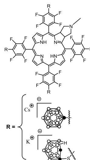
Figure 13: Symmetrical tetra substituted carborane-chlorin conjugates, see ref. 68, 89.
