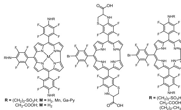
Figure 17 Mono and di substituted amino acid-corrole derivatives, see ref. 107.
