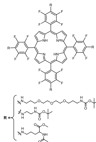
Figure 6 Symmetric tetra amino substituted porphyrin, see ref. 79
