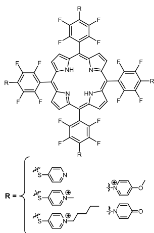
Figure 11 Tetra cationic pyridyl porphyrins, see ref. 84, 85.
