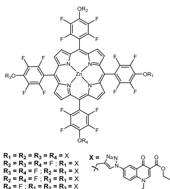
Figure 8 Zinc metallated porphyrin-quinolone conjugates, see ref. 36.
