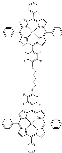
Figure 26 Zn porphyrin dimer connected via thio alkyl tether, see ref. 51.
