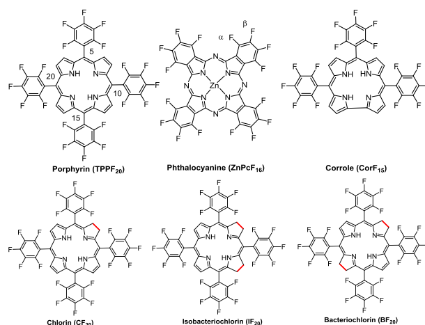
Figure 1 Fluorinated porphyrinoid platforms.
