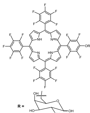
Figure 5 Mono substituted O-galactosyl porphyrin, see ref. 78
