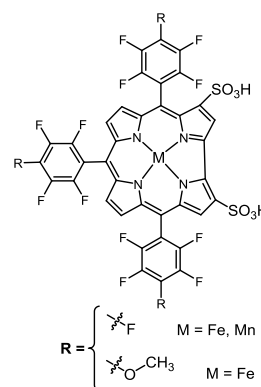
Figure 22 Tri methoxy-substituted bis-sulfonated corroles. See ref 134.
