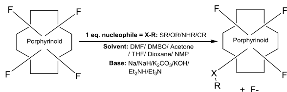
Figure 2 Scheme of nucleophilic substitution on fluorinated porphyrinoids (substitution in the order of softness S>N>O).
