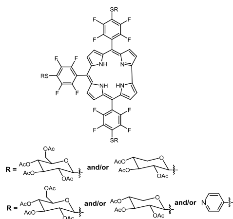
Figure 15 Combinatorial library of sugars and pyridyl substituted corroles, see ref. 39, 105.
