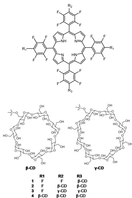
Figure 9: Porphyrin-CD conjugates, see ref. 82.
