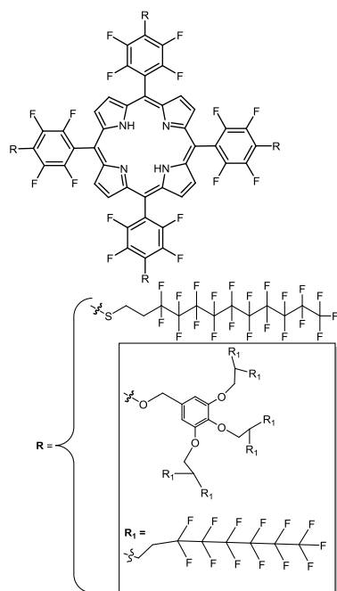
Figure 25 Highly fluorinated symmetric porphyrin, see ref. 42, 176.
