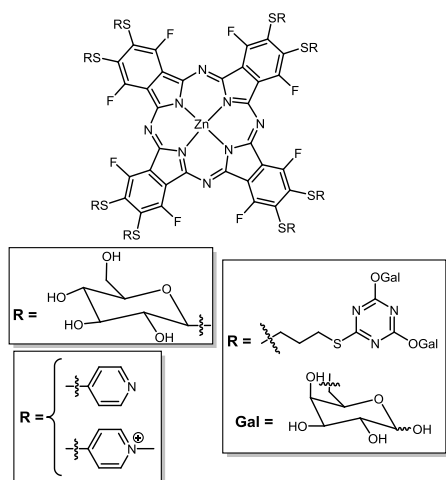
Figure 18 Symmetrical octa and hexadecaglycosyl-ZnPc, see ref. 112, 113, 115.
