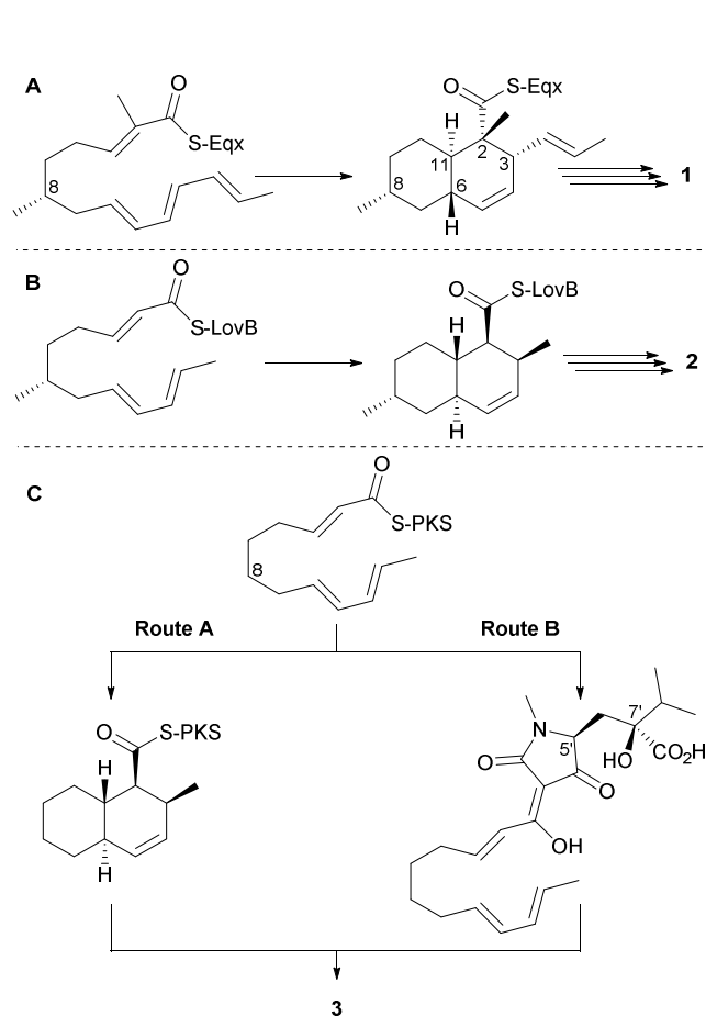
Scheme 1 (A) Proposed biosynthesis of equisetin ( 1 ) involving an early stage enzyme-catalysed Diels-Alder (DA) cycloaddition. 4b (B) Proposed biosynthesis of Lovastatin ( 2 ) involving the Diels-Alderase LovB. 2b (C) Two possible biosynthetic routes to JBIR-22 ( 3 ). Route A: Early stage DA cycloaddition which would require enzyme catalysis to control the stereochemical outcome. Route B: Late stage DA cycloaddition which could occur spontaneously under substrate control or occur via enzyme catalysis. For clarity the numbering system used reflects that reported for equisetin ( 1 ) in reference 4d. PKS = polyketide synthase.
