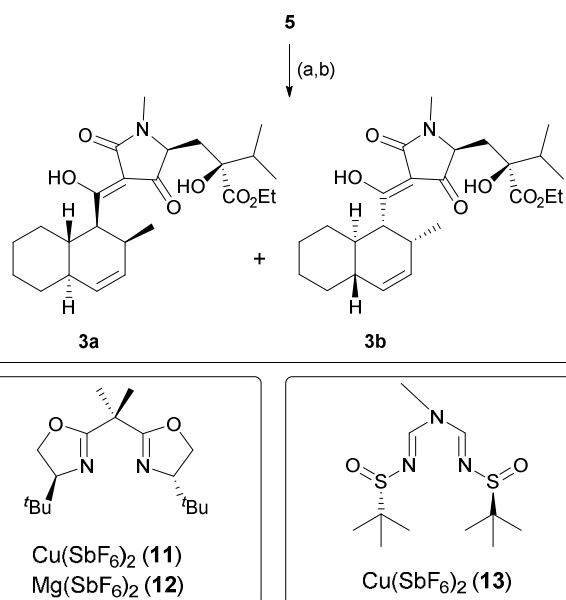
Scheme 3 IMDA cyclisation of 5 followed by hydrolysis to yield diastereomeric mixture of 3a and 3b . (a) See text and Table 1 for conditions of thermal and Lewis acid catalysed IMDA; (b) NaOH (2N), EtOH, 110 °C (MW), 20 minutes, (71% for Table 1, entry 3). Crude reaction mixtures analysed by 1 H NMR and UPLC.
