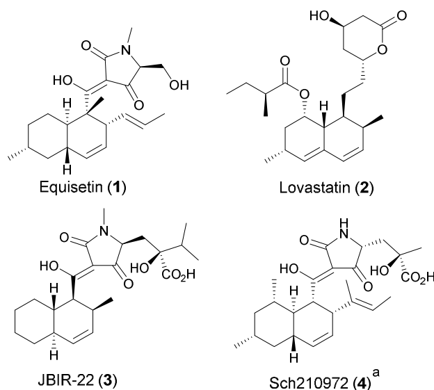
Figure 1 Examples of natural products that contain an unsaturated decalin ring system that may be formed by a Diels-Alderase catalysed reaction. a To date only the relative stereochemistry of 4 has been reported.
