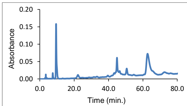
Figure 3. Reverse phase HPLC from cross-linking \alpha 99 -fumaryl- \alpha 99 , \beta_2 with 15 eq. of azide 2 . Peaks: heme (10 min.), \beta\beta -cross-linked subunits (45 min.), over-modified \beta\beta -cross-linked subunits (52 min.) and \alpha\alpha -cross-linked subunits (62 min.).
