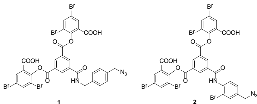
Figure 2. Azido-containing cross-linking reagents for modification of fumaryl cross-linked Hb.
