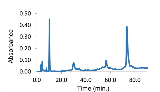
Figure 4. Reverse phase HPLC from cross-linking \alpha 99 -fumaryl- \alpha 99 , \beta_2 with 8.5 eq. of azide 2 . Peaks: heme (10 min.), \beta subunits (30 min.), \beta\beta cross-linked subunits (56 min.) and \alpha\alpha cross-linked subunits (73 min.).
