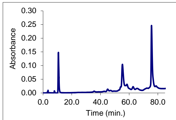
Figure 1. Reverse phase HPLC trace under dissociating conditions of \alpha 99-fumaryl- \alpha 99, \beta 82-trimesyl- \beta 82 Hb. A minor peak from elution of free heme appears at 11 min., while the major peaks are the \beta cross-linked subunits occurring at 56 min. and \alpha cross-linked subunits at 76 min.
