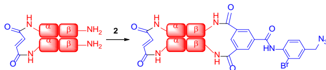
Scheme 2. Addition of azide 2 to \alpha 99 -fumaryl- \alpha 99 , \beta_2 in sodium borate buffer (0.05 M, pH 9.0) to yield \alpha 99 -fumaryl- \alpha 99 , \beta_{82} -azido- \beta_{82} by selective modification of the \beta -Lys-82 residues.
