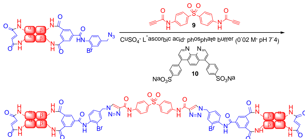
Scheme 3. Reaction of \alpha 99-fumaryl- \alpha 99, \beta 82-azido- \beta 82 with bis-alkyne 9 produces a cross-linked bis-tetramer.
