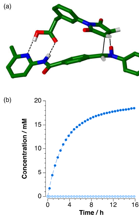
Fig. 2 (a) Stick representation of the calculated transition state (B3LYP/6-31G+(d,p)) for the recognition mediated reaction between nitrone 4 and maleimide 5b to afford cis - 7b . Carbon atoms are coloured green, oxygen atoms red, nitrogen atoms blue, the fluorine atom yellow-green and hydrogen atoms grey. Most hydrogen atoms are omitted for clarity. Dashed lines represent hydrogen bonds and solid lines represent the location of covalent bonds formed during the reaction. (b) Kinetic data for the reaction between nitrone 4 and maleimide 5b . Starting conditions: [\mathbf{4}] = [\mathbf{5b}] = 20 mM; \text{CD}_2\text{Cl}_2 saturated with p -toluenesulfonic acid monohydrate; 273 K. Concentrations determined by 470.4 MHz ^{19}\text{F} NMR spectroscopy. Dark blue circles represent cis - 7b and light blue circles represent trans - 7b . The dashed line represents the best fit of the data to the appropriate kinetic model (See Electronic Supplementary Information).
