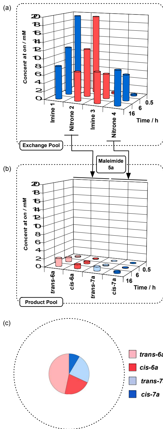
Fig. 3 Distribution of compounds present in (a) the Exchange Pool and (b) the Product Pool at 0.5 h, 6 h and 16 h in the recognition-disabled experiment (Initial conditions: \text{CD}_2\text{Cl}_2 / saturated with PTSA / [\mathbf{1}] = [\mathbf{2}] = [\mathbf{5a}] = 20 mM). Species bearing a recognition site are coloured blue and those having no recognition site are coloured red. (c) Composition of the Product Pool after 16 h. The area of the dashed circle represents 100% conversion of maleimide 5a to cycloadducts. The inset pie chart shows the composition of the Product Pool and its area is scaled to match the conversion of maleimide 5a to cycloadducts (22%) at 16 h.
