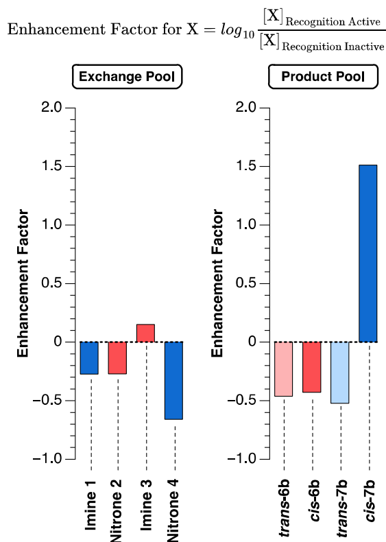
Fig. 7 Calculated Enhancement Factors (EFs) for each member of the exchange and Product Pools after 16 h in the experiment where recognition is active (data shown in Figure 4).
