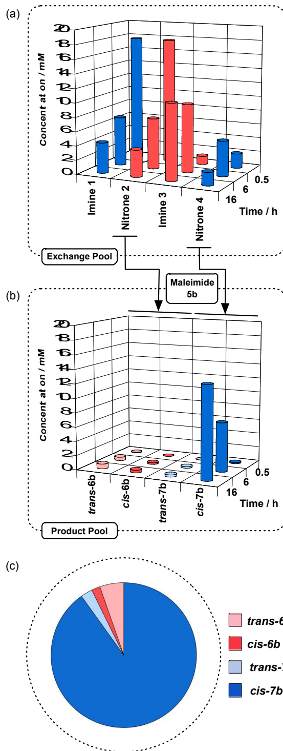
Fig. 4 Distribution of compounds present in (a) the Exchange Pool and (b) the Product Pool at 0.5 h, 6 h and 16 h in the recognition-enabled experiment (Initial conditions: \text{CD}_2\text{Cl}_2 / saturated with PTSA / [\mathbf{1}] = [\mathbf{2}] = [\mathbf{5b}] = 20 mM). Species bearing a recognition site are coloured blue and those having no recognition site are coloured red. (c) Composition of the Product Pool after 16 h. The area of the dashed circle represents 100% conversion of maleimide 5b to cycloadducts. The inset pie chart shows the composition of the Product Pool and its area is scaled to match the conversion of maleimide 5b to cycloadducts (72%) at 16 h.
