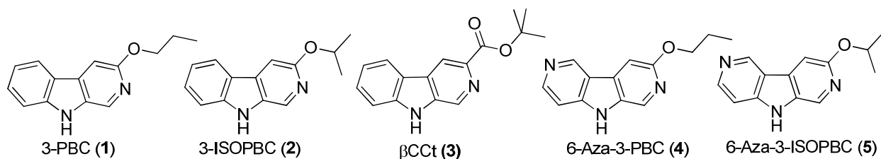
Figure 1. Structures of 3-PBC (1), 3-ISOPBC (2), \beta CCt (3), 6-Aza-3-PBC (4) and 6-Aza-3-ISOPBC (5)
