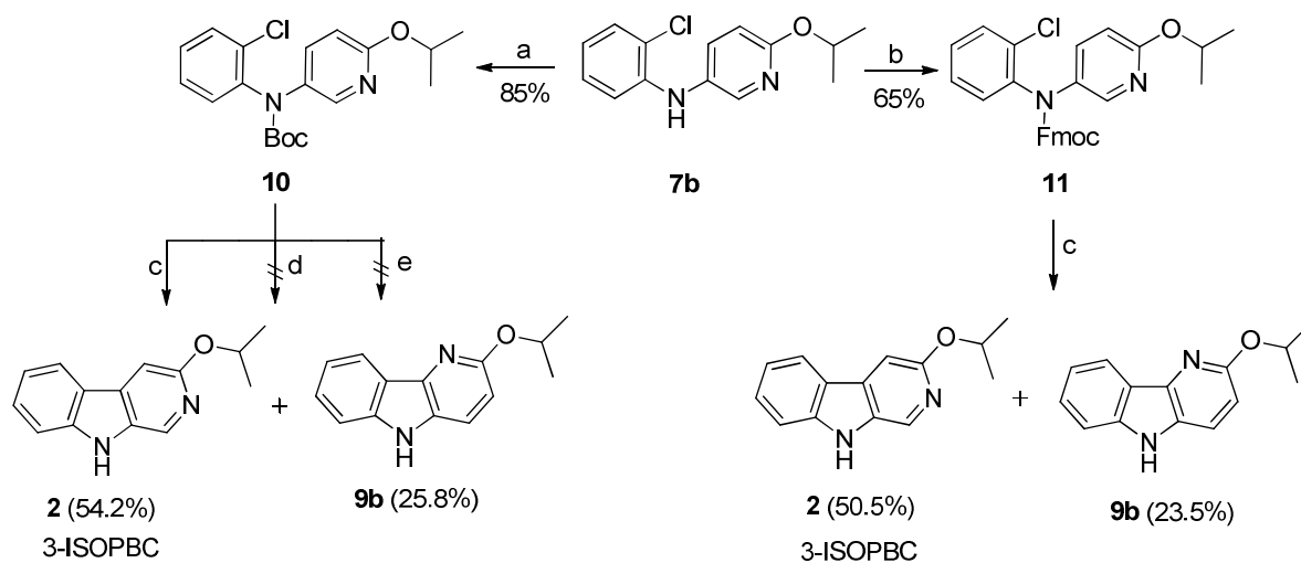
Scheme 2. Synthesis of the Carbamate Protected Analogs from Intermediate 7b
