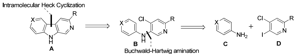
Scheme 3. Retrosynthetic Analysis of 3,6-Disubstituted β-carbolines
