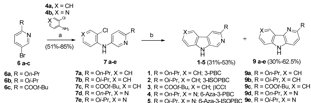
Scheme 1. Synthesis of Substituted Carboline Analogues
