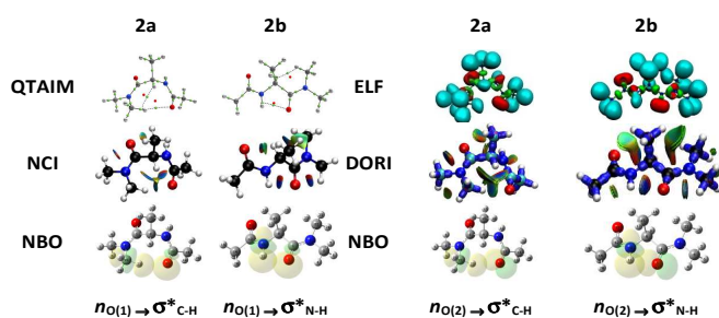
Figure 4: QTAIM, ELF, NCI, DORI and NBO graphical representations for conformers 2a and 2b . QTAIM green points and red points represent bond critical points and cage critical points, respectively. NCI figures were obtained with a blue-green-red scale ranging from -0.02 < \text{sign}\lambda_2 < 0.02 au and with a RDG cutoff of 0.5 au. ELF localization domains were built with a 0.8 au isodensity value. DORI were also obtained with a blue-green-red scale ranging from -0.02 < \text{sign}\lambda_2 < 0.02 au. NBO plots of orbitals in n \rightarrow \sigma^*_{\text{NH}} interactions were obtained with an isovalue of 0.04 au. All figures obtained from B3LYP/aug-cc-pVDZ electron densities at B3LYP-D3/aug-cc-pVDZ optimised geometries.
