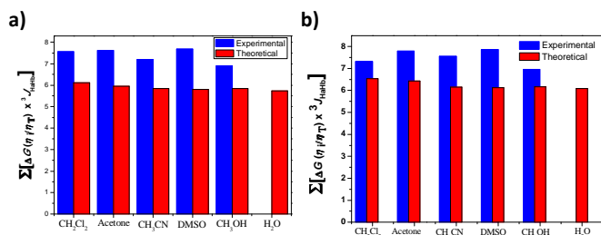
Figure 2: Comparison between experimental and theoretical obtained ^3J_{\text{HaHb}} SSCCs for compounds 1 (left) and 2 (right). Theoretical values were obtained by averaging all conformer contributions for the ^3J_{\text{HaHb}} values.
