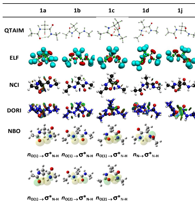
Figure 3: QTAIM, ELF, NCI, DORI and NBO graphical representations for conformers 1a-1d and 1j . QTAIM green points and red points represent bond critical points and ring critical points, respectively. NCI figures were obtained with a blue-green-red scale ranging from -0.02 < \text{sign}\lambda_2 < 0.02 au and with a RDG cutoff of 0.5 au. ELF localization domains were built with a 0.8 au isodensity value. DORI were also obtained with a blue-green-red scale ranging from -0.02 < \text{sign}\lambda_2 < 0.02 au. NBO plots of orbitals involved in n \rightarrow \sigma^*_{\text{NH}} interactions were obtained with an isovalue of 0.04 au. All figures were obtained from B3LYP/aug-cc-pVDZ electron densities at B3LYP-D3/aug-cc-pVDZ optimised geometries.
