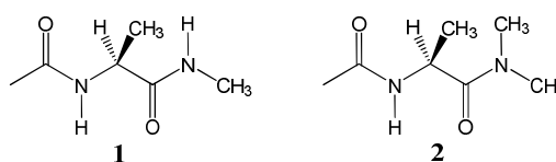
Scheme 1: Ac-Ala-NHMe ( 1 ) and Ac-Ala-N(Me) 2 ( 2 ) structure representations.
