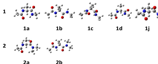
Figure 1: B3LYP-D3/aug-cc-pVDZ optimised geometries of the most stable conformers of compounds 1 and 2 .
