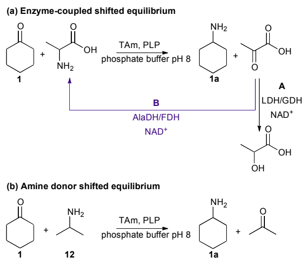
Scheme 1. Methods used to shift the TAM reaction equilibrium toward the desired amine product, using 1 as the ketone acceptor. (a) Enzyme-coupled shifted equilibrium; (b) amine donor shifted equilibrium
