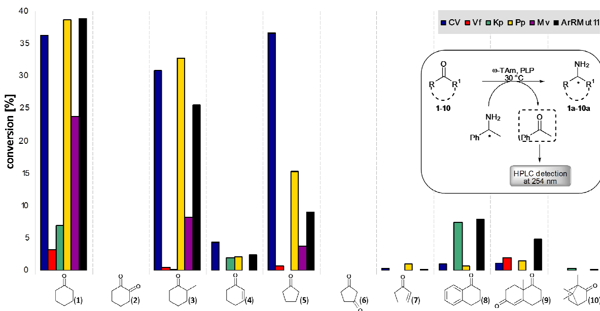
Figure 1. Initial screening results giving conversions for a range of cyclic ketone substrates employing the selected \omega -TAMs. ( R )- or ( S )-MBA 11 were used as amine donors and the product acetophenone was detected by HPLC analysis (see Scheme). All reactions were performed in triplicate and standard deviations were less than 10%.
