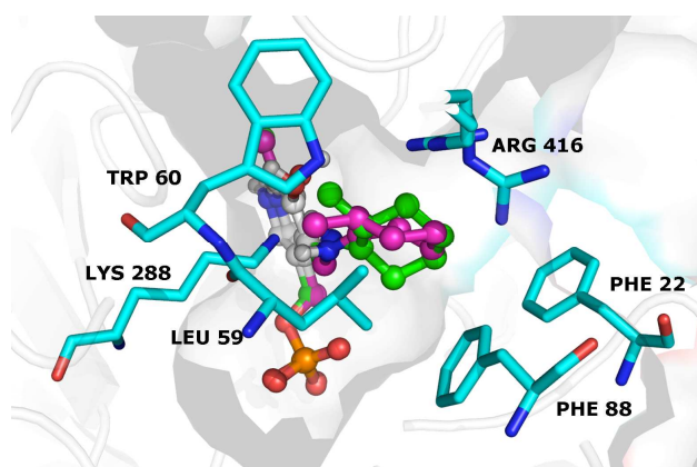
Figure 2. Docking of (2 S ) (pink) and (2 R ) (green) quinonoid intermediate into the active site of CV-TAm (4AH3). The binding pocket is indicated as grey shadow, and amino acids involved in the transamination reaction are labelled.
