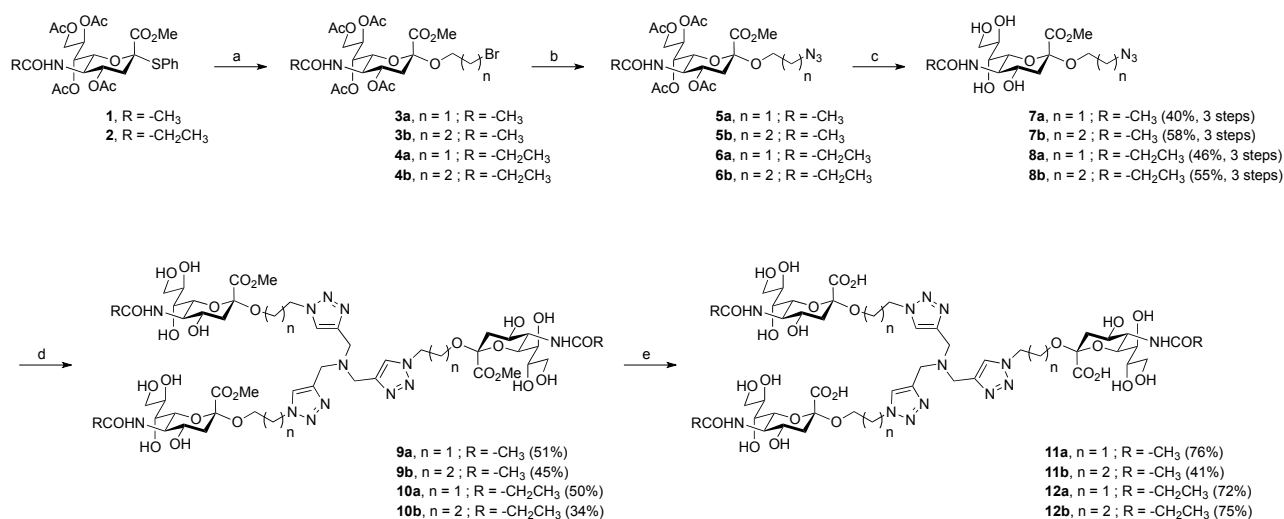
Scheme 1. Synthesis of 11a , 11b , 12a and 12b . Reagents and conditions: (a) i: molecular sieves 3Å, 2-bromoethanol or 3-bromopropan-1-ol, CH 3 CN/CH 2 Cl 2 (3:2), rt, 2 h, ii: AgOTf, IBr, -73 °C, 4.5 h, iii: DIPEA, -73 °C, 30 min. (b) NaN 3 , TBAI, DMSO, rt, 6 h. (c) i: NaOMe, MeOH, rt, 3 h, ii: H + ion exchange resin. (d) Tripropargylamine, CuSO 4 , sodium ascorbate, THF/H 2 O (1:1), 50 °C, 3 h then rt, 18 h. (e) i: LiOH, MeOH, rt, 9 h, ii: H + ion exchange resin.
