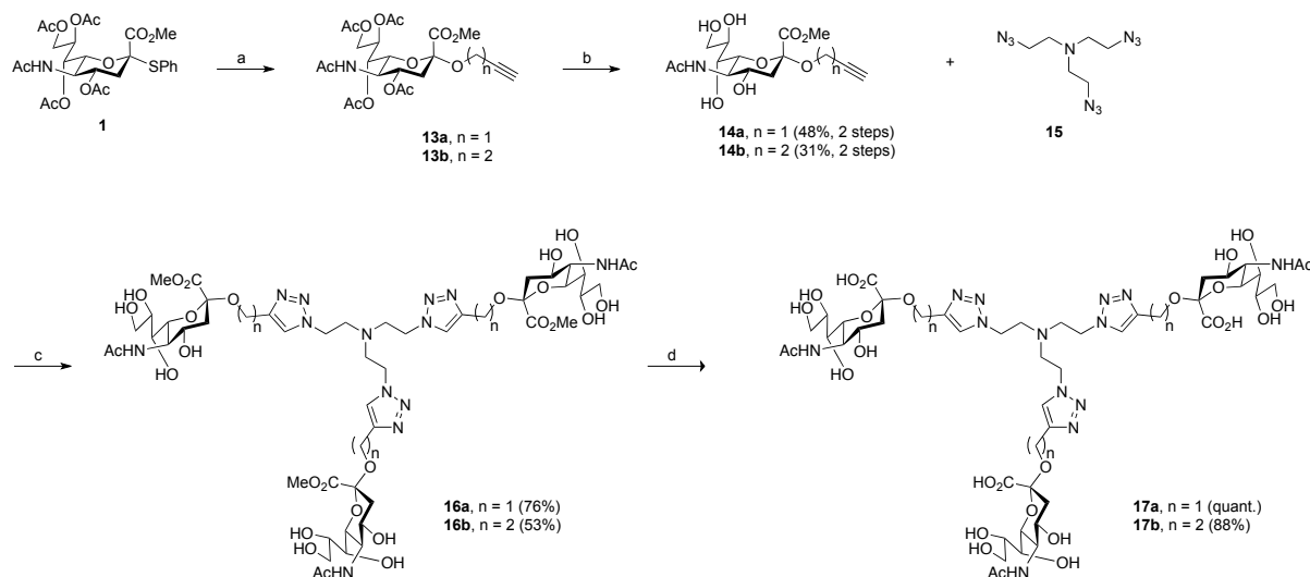
Scheme 2. Synthesis of 17a and 17b . Reagents and conditions: (a) i : molecular sieves 3Å, propargyl alcohol or 3-butyn-1-ol, CH 3 CN/CH 2 Cl 2 (3:2), rt, 2 h, ii : AgOTf, 1Br, -73 °C, 4.5 h, iii : DIPEA, -73 °C, 30 min. (b) i : NaOMe, MeOH, rt, 3 h, ii : H + ion exchange resin. (c) CuSO 4 , sodium ascorbate, THF/H 2 O (1:1), 50 °C, 3 h then rt, 18 h. (d) i : LiOH, MeOH, rt, 9 h, ii : H + ion exchange resin.
