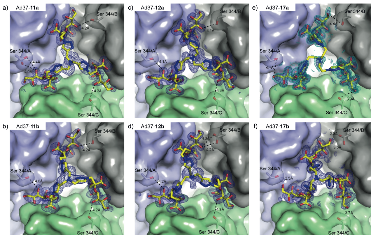
Figure 4. Binding of 11a , 11b , 12a , 12b , 17a and 17b to the Ad37 fiber knob (top view, a-f). Simulated annealing omit difference electron density maps for 11a (a, 2.0 Å resolution, PDB ID 4K6T), 11b (b, 1.9 Å resolution, PDB ID 4K6U), 12a (c, 1.5 Å resolution, PDB ID 4K6W), 12b (d, 1.5 Å resolution, PDB ID 4K6V), 17a (e, 1.4 Å resolution, 4XQA) and 17b (f, 1.6 Å resolution, 4XQB) were contoured at 3 \sigma and shown with a radius of 2.4 Å around the ligand (dark blue). For 17a (e), an additional map at 2 \sigma shows an ordered density for the ligand base (cyan). One inhibitor molecule is simultaneously bound with its three terminal sialic acid residues. Serine 344 (Ser344) is within the van-der-Waals radius of the sialic acid moieties and only 17b (f) is capable of forming hydrogen bonds with this residue. Black dashed lines in a-e indicate distances to Ser344.
