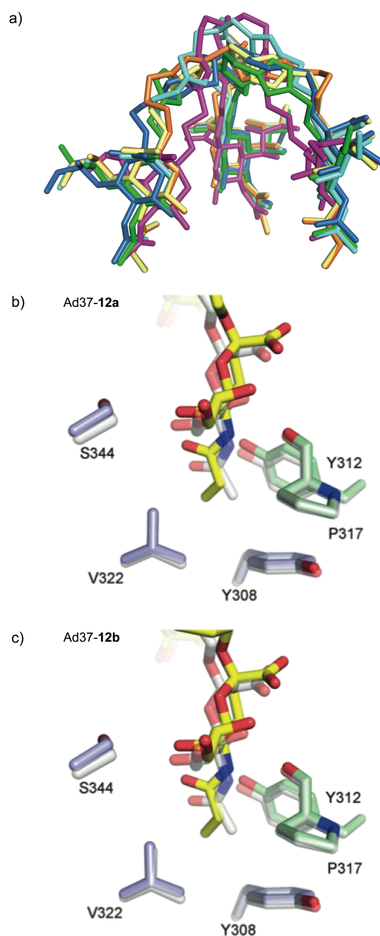
Figure 5. a) Superposition of the inhibitor compounds ( 11a = blue, 11b = cyan, 12a = yellow, 12b = orange, 17a = green, 17b = magenta). The corresponding protein chains were aligned in PyMOL. 17b possesses additional internal order, its sialic acid moieties are rotated sideward and its linker forms a bell-like structure; b) and c) Hydrophobic interactions of 12a (b) and 12b (c). For the two compounds, the additional methyl group of the propionic acid group is facing away from Y308 and V322, pushing the whole ligand up.
