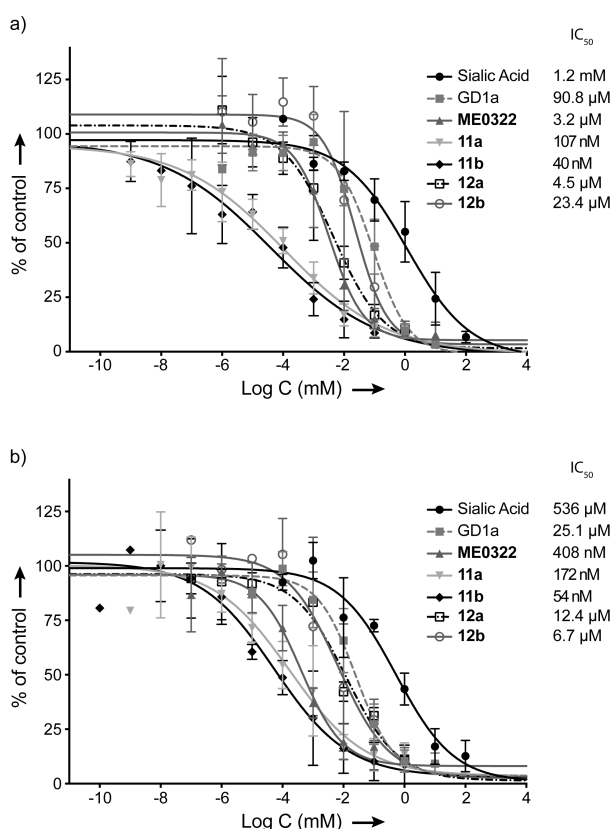
Figure 2. Effect of the set of trivalent sialic acid derivatives 11a-b and 12a-b on Ad37 binding to and infection of HCE cells. a) Virion binding in the presence of inhibitors at different concentrations. b) Infection at different concentrations of the inhibitors. Data are presented as % of control that is the value obtained in the absence of inhibitor.
