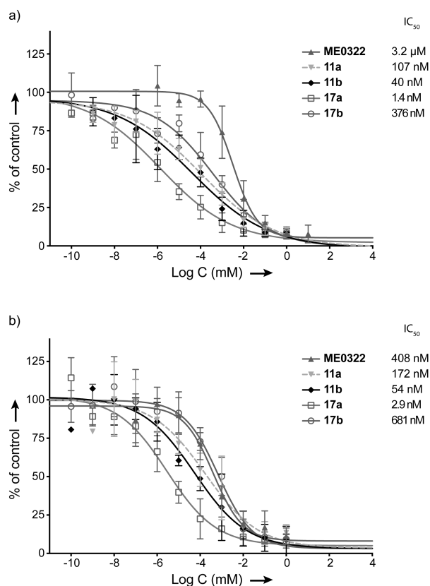
Figure 3. Effect of the set of trivalent sialic acid derivatives ( 17a-b ) on Ad37 binding to and infection of HCE cells. a) Virion binding in the presence of inhibitors at different concentrations. b) Infection at different concentrations of the inhibitors. Data are presented as % of control that is the value obtained in the absence of inhibitor.
