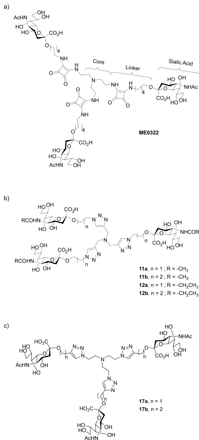
Figure 1. Structure of a) trivalent sialic acid ME0322 , 21 a potent inhibitor of Ad37, b) the first-generation triazole linker-based trivalent sialic acid derivatives and c) the second-generation triazole linker-based trivalent sialic acid derivatives.
