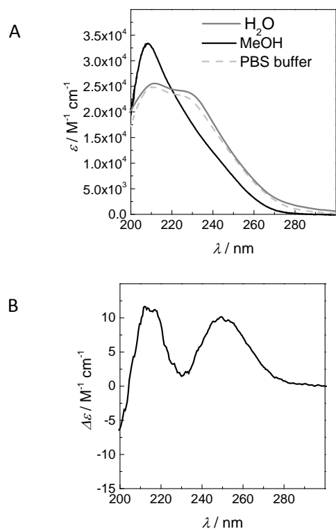
Figure 1 (A) UV-Vis absorption spectra of 1 in MeOH (black line), water (dark grey line) and PBS buffer (grey dashed line). c = 10 \mu\text{M} in PBS buffer and 50 \mu\text{M} in water and MeOH; (B) CD spectrum of 1 in water. c = 50 \mu\text{M}
