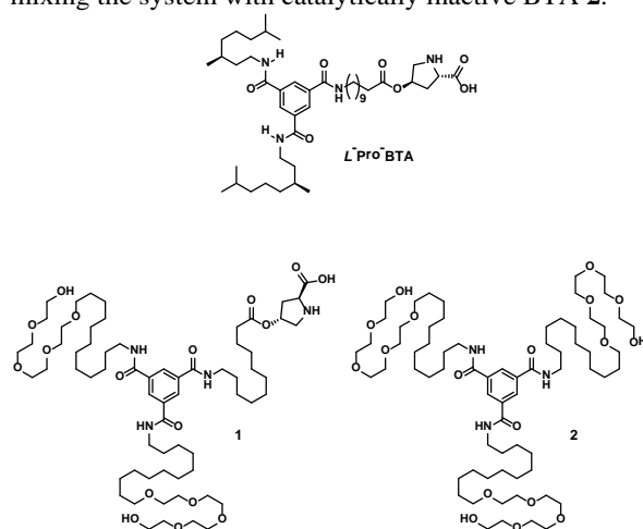
Scheme 1. Molecular structures of BTA derivatives L -pro-BTA, 1 and 2 .
