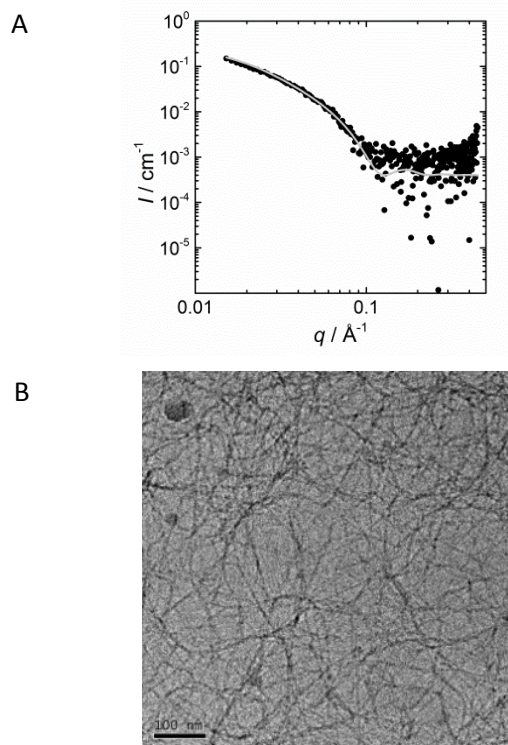
Figure 2 (A) Experimental SAXS profile of BTA 1 , ( c = 3.7 \text{ mM} in \text{H}_2\text{O} ). The solid grey line is the fit with a form factor model for flexible cylinders (i.e., the Schurtenberger-Pedersen form factor for worm-like, self-avoiding chains). 19 (B) Cryo-TEM image of BTA 1 showing the presence of high aspect ratio fibres ( c = 0.4 \text{ mM} ). The dark circular objects in the image are non-vitrified water. The scale bar represents 100 nm.
