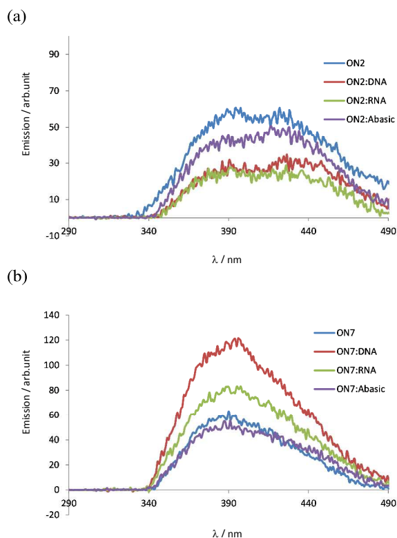
Figure 2. Selected fluorescence emission spectra for ON's containing monomer X . (a) ON2, and (b) ON7. Excitation wavelength = 255 nm
