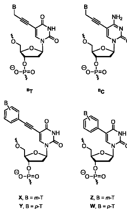
Figure 1. Double-headed nucleotides. B = nucleobase. T = thymine-1-yl.
