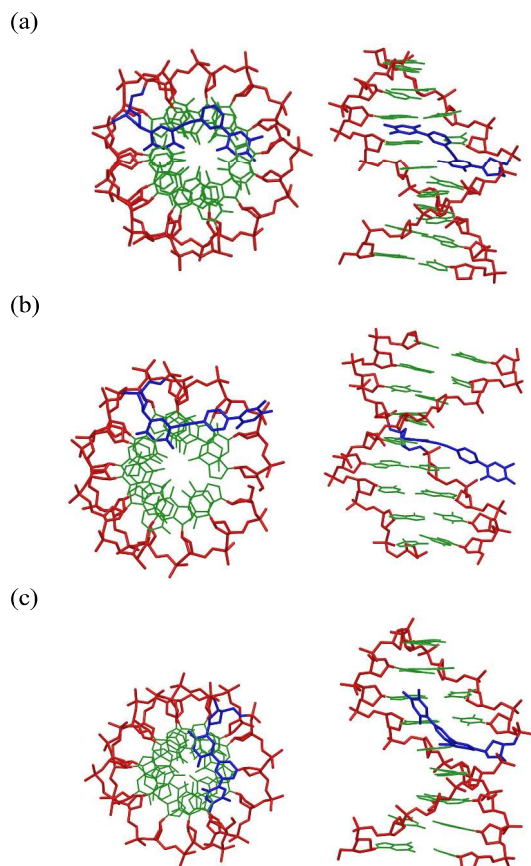
Figure 3. Minimized structures from selected molecular dynamics simulations. Top views and side views of (a) ON2:DNA, (b) ON3:DNA and (c) ON4:DNA. The sugar-phosphate backbone is colored red, Watson-Crick nucleobases green and modified monomers blue.
