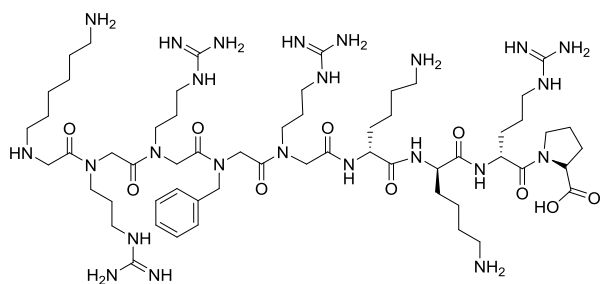
Figure 3. Peptoid/peptide hybrid CGP64222.
