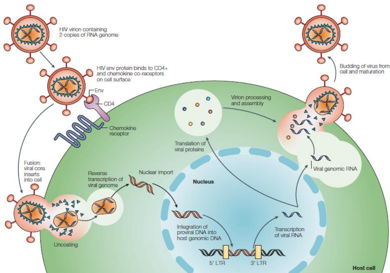
Figure 2. HIV replication cycle. Reprinted from ref 3 with permission from Nature.
