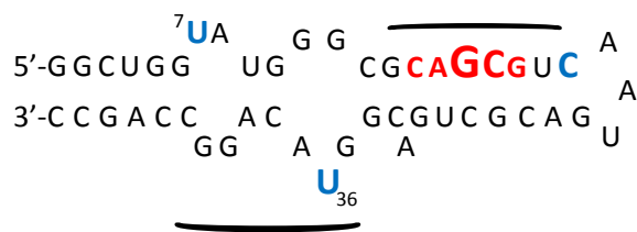
Figure 6. Summary of RNase protection of RRE IIB in the presence of increasing concentrations of BPBA1. Font size reflects level of protection from RNase A (blue) and RNase VI (red). Curved lines indicate regions of peptide:RNA contact.
