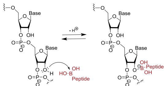
Figure 9. Suggested reversible covalent bond formation between boronic acid on branched peptide and 2'-OH on RNA.
