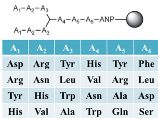
Figure 6. 3.3.3 Branched peptide library.
