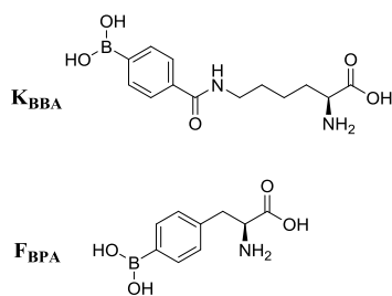
Figure 8. Structures of boronic acid monomers K_{BBA} and F_{BPA} .
