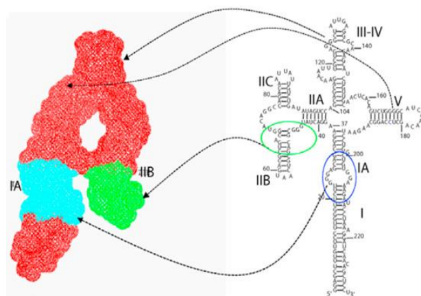
Figure 5. Right: Secondary structure of full-length RRE RNA with domain locations; Left: SAXS topological structure, with the high affinity binding site IIB in green and oligomerization site between IIB and IA (cyan legs). Reprinted from ref 40 with permission from Elsevier.
