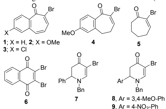
Fig. 3 Selected enone derivatives employed in these studies
