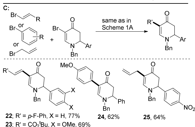
Scheme 1 Co-catalyzed reductive cross-coupling of \alpha -bromo enones with organic bromides
