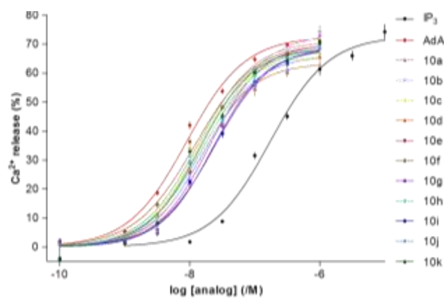
Fig. 3 Concentration-dependent release of Ca 2+ (%) by IP 3 , AdA and triazolophostins from the intracellular stores of cells expressing IP 3 R1. Results show means ± SEM from at least 3 experiments.
