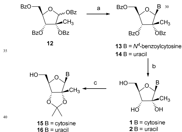
Scheme 2 Synthesis of 2'-C-Me-cytidine ( 1 ) and 2'-C-Me-uridine ( 2 ) nucleosides and their corresponding 2',3'-O-isopropylidene protected analogues 15 and 16 . Reagents and conditions: a) N 4 -benzoylcytosine/uracil, N,O -bis(trimethylsilyl)acetamide, MeCN, 80 °C, 1 h, then 12 , \text{SnCl}_4 , reflux, 3 h, 80% for 13 , 90% for 14 ; b) sat. \text{NH}_3 in MeOH, rt, overnight, 80% for 1 , 91% for 2 ; c) p -TSA, acetone, 2,2-dimethoxypropane, rt, overnight, 90% for 15 , 80% for 16 .
