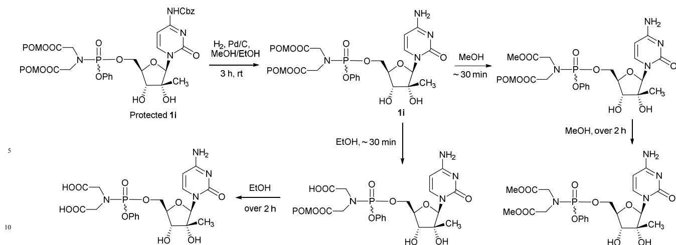
15 Scheme 4 Decomposition of pivaloyloxymethyl (POM) group of compound 1i under hydrogenation condition.
