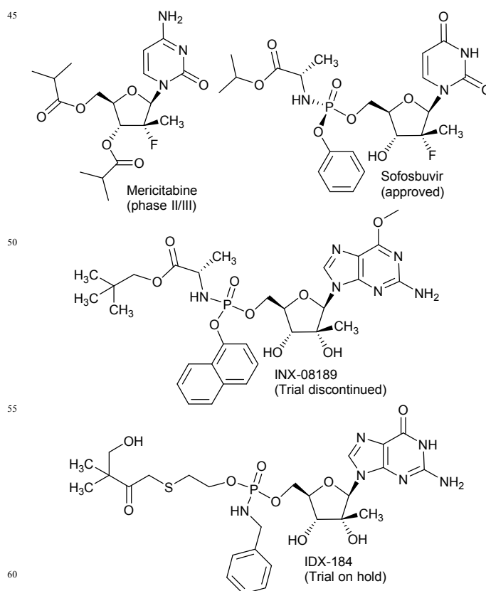
Fig. 1 Chemical structures of clinically advanced and approved anti-HCV drugs.
