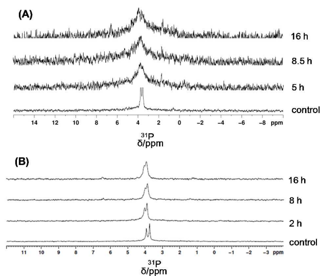
Fig. 3 Stack plot of 31 P NMR spectra depicting the stability of ProTides (A) 1g and (B) 2c in human serum at different time intervals. Control: no serum is added.
