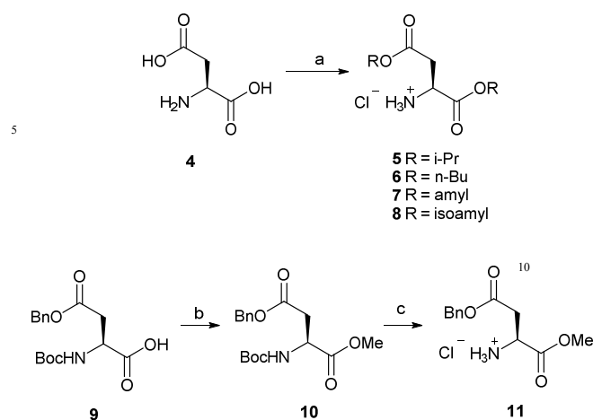
Scheme 1 Synthesis of aspartic acid esters used in the synthesis of phosphoramidate analogues. Reagents and conditions: a) \text{SOCl}_2 , i -PrOH/ n -BuOH/amyl alcohol/isoamyl alcohol, 0 °C to rt, 12 h, then reflux, 3 h/heat to 50 °C for 8 , 40-94%; b) EDC.HCl, \text{Et}_3\text{N} , MeOH, \text{CH}_2\text{Cl}_2 , 0 °C to rt, 24 h, 72%; c) 5-6N HCl in i -PrOH, \text{CH}_2\text{Cl}_2 , rt, 3-4 h, 75%.
