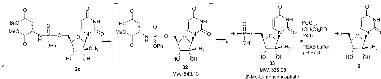
Fig. 4 Metabolism of ProTide 2c in human liver S9 fraction leading to the formation of 2'-Me-U monophosphate and its chemical synthesis from nucleoside 2 .
