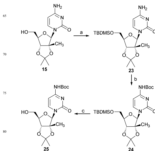
Scheme 5 a) Imidazole, TBDMSO, anhydrous pyridine, 0 °C to rt, overnight, 95%; b) di- tert -butyldicarbonate, THF:dioxane (1:1), reflux, 5 h, 77%; c) Et 3 N.3HF, dry THF:pyridine (1:1), 0 °C to rt, 4 h, 92%.
