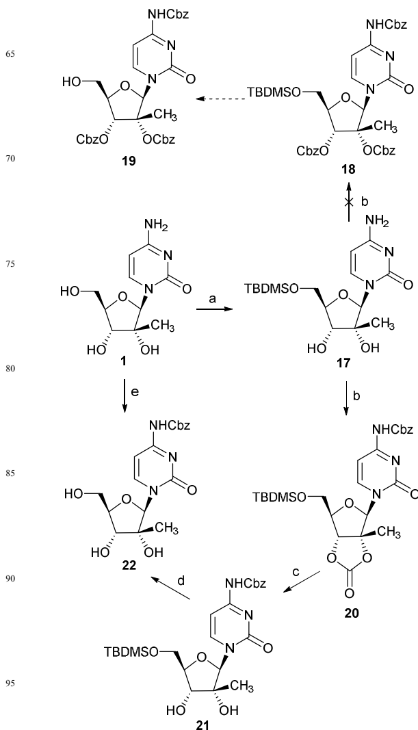
Scheme 3 a) Imidazole, \text{TBDMSCl} , anh. pyridine, 0 °C to rt, overnight, 97%; b) benzyl chloroformate, DMAP, dry \text{CH}_2\text{Cl}_2 , 0 °C to rt, 24 h, 80%; c) pyridine: \text{H}_2\text{O} (1:1), reflux, 2 h; d) \text{Et}_3\text{N} \cdot 3\text{HF} , dry THF, rt, overnight, 85%; e) \text{TMSCl} , anh. pyridine, 0 °C to rt, 1.5 h, then benzyl chloroformate, 0 °C to rt, 2 h, 90%.
