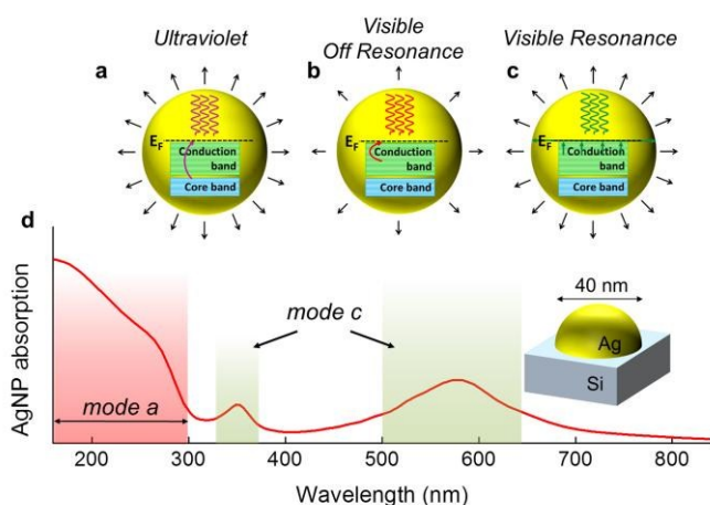
Fig. 1. (a-c) Schematic representation of the main physical mechanisms of absorption we exploit in the current work and their corresponding thermal effect on metallic nanostructures. (d) Calculated absorption spectrum of a 40nm diameter Ag nanoparticle (Ag NP) on top of a Si substrate, as shown in the inset schematic. Interband absorption (mode a) dominates the red shaded region, while intraband absorption (LSPR driven, mode c) is dominating the green shaded regions (at \sim 350nm the quadrupole and \sim 580nm the dipole LSPR contributions respectively).
