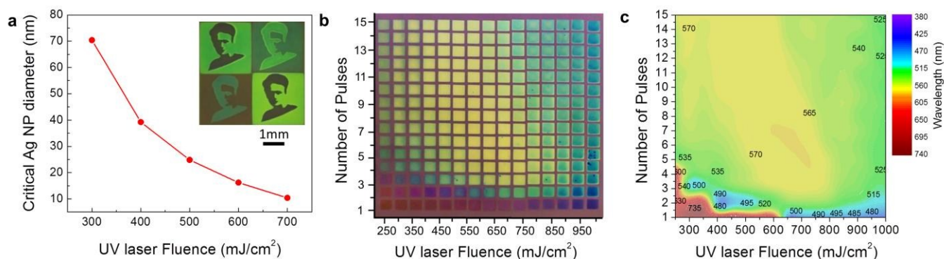
Fig. 4. (a) Critical nanoparticle diameter (the diameter value under which every particle remains practically cold during the UV LA process; hence these particles cannot be further manipulated upon irradiation) as a function of applied laser fluence. The inset shows an optical microscopy image of the “Marie Curie Actions” logo produced by projection mask under LISA / UV MONA-LISA. Each colour represents a different UV LA fluence. (b) A digital photo of a grid of LISA / UV MONA-LISA spots (2.5×2.5 mm 2 each) of varying fluence (x-axis) and number of pulses (y-axis) produced on a 10nm Ag thin film. (c) Contour plot of the dominant LSPR maximum acquired from optical reflectivity spectra from each spot of (b) (in the case of bimodal responses, the spectral value of the stronger reflectivity peak is reported).
