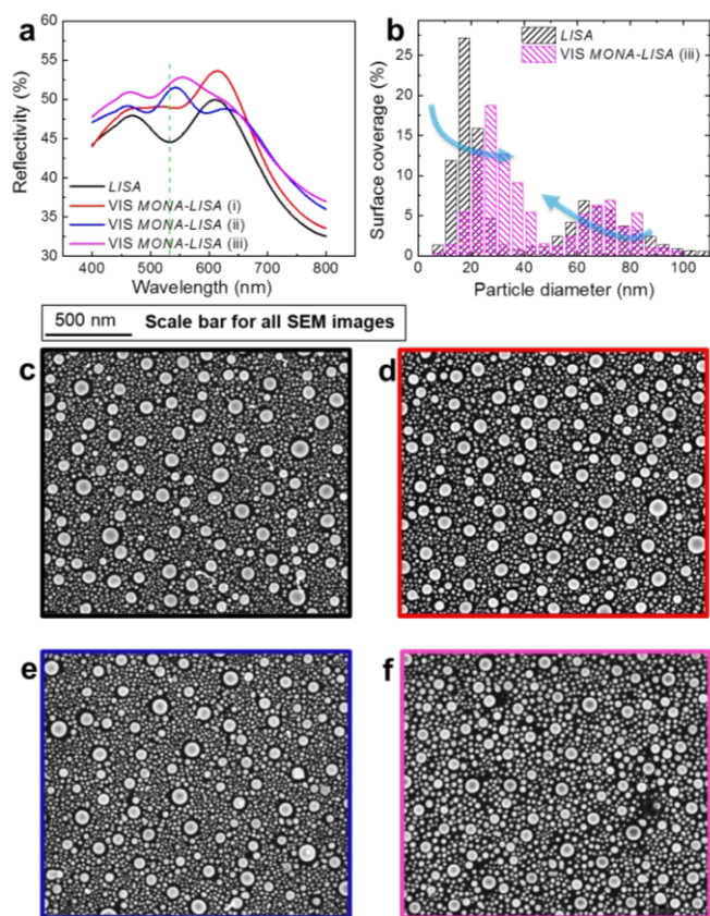
Fig. 6. (a) Optical reflectivity spectra of UV MONA-LISA (2 pulses, 248 nm at 350 mJ/cm 2 - black line), used as a template for the subsequent VIS MONA-LISA (532 nm at 125 mJ/cm 2 ) with 500 pulses (red line), 2000 pulses (blue line) and 4000 pulses (magenta line). The green dashed line sets the 532 nm mark. (b) Surface coverage of the nanoparticles in relation to the particle diameter for all the cases of (a). (c) SEM image of the UV MONA-LISA processed sample. (d) SEM image of the VIS MONA-LISA (i) sample (500 pulses). (e) SEM image of the VIS MONA-LISA (ii) sample (2000 pulses) and (f) SEM image of the VIS MONA-LISA (iii) sample (4000 pulses).
