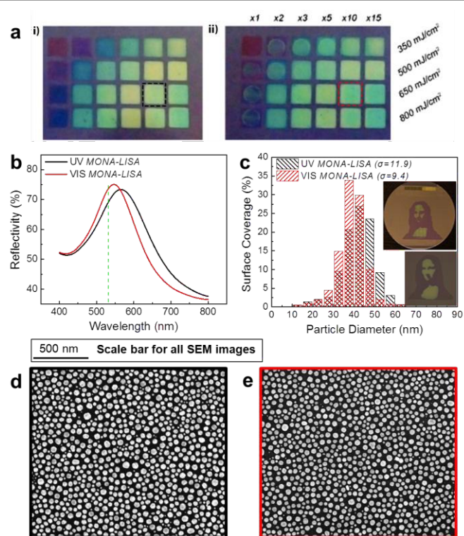
Fig. 5. (a) A digital photo of a grid of LA spots of varying fluence (y-axis) and number of pulses (x-axis) produced on a 10 nm Ag thin film: i) produced via the LISA / UV MONA-LISA process and ii) replica of i) with subsequent VIS MONA-LISA treatment (combined UV and VIS laser annealing). (b) Optical response of a Ag/Si sample (initial effective thickness of 10 nm) after UV MONA-LISA (10 pulses, 248 nm at 650 mJ/cm 2 - black line) and UV + VIS MONA-LISA (10 pulses, 248 nm at 650 mJ/cm 2 and 500 pulses, 532 nm at 125 mJ/cm 2 - red line). (c) Surface coverage of the nanoparticles in relation to the particle diameter for the two spots indicated with red and black dashed boxes in (a) and with optical response shown in (b). Inset depicts two portraits of Da Vinci's Mona Lisa validating the potential and scalability of the MONA-LISA process. (d) SEM image of the UV MONA-LISA sample. (e) SEM image of the UV + VIS MONA-LISA sample.
