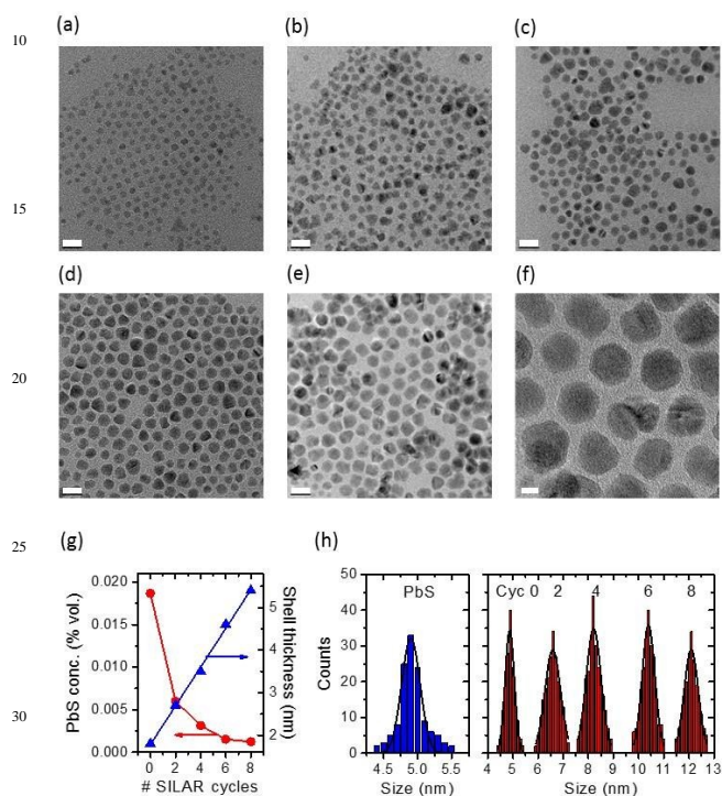
Figure 1. Size and size distribution of giant QDs. (a)-(f): TEM. (a) Representative TEM images of parent PbS/CdS QDs after cation exchange, before SILAR. (b)-(f): PbS/CdS QDs after coating with 2 (b), 4 (c), 6 (d) and 8 (e) SILAR cycles. (f) HR-TEM image of sample (e). Scale bar is 20 nm in (a)-(e) and 5 nm in (f). (g) Overall shell thickness and Pb volume concentration as a function of the number of SILAR cycles. (h) Size distribution of parent PbS QDs before cation exchange (blue) and of the core/shell QDs after different SILAR cycles. The solid lines are Gaussian fits of the experimental data.
