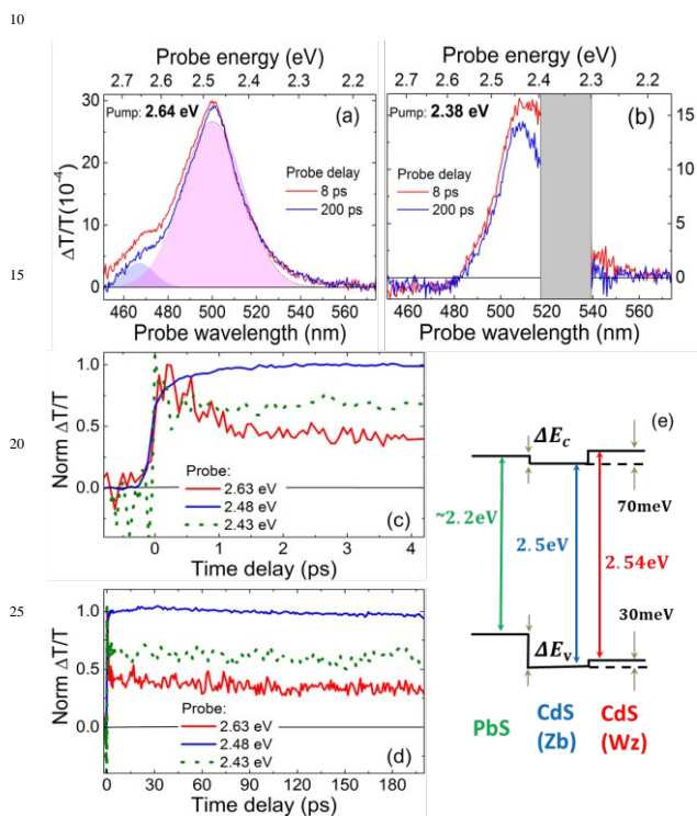
Figure 5. \Delta T/T for the Cyc 8 sample. (a,b) \Delta T/T spectra at different pump-probe delays: (a) pump at 2.64 eV (470 nm), absorbed fluence of 1.3 \mu\text{J}\cdot\text{cm}^{-2} , dashed line is the fit of the blue spectrum with the two Gaussian components (violet and pink areas); (b) pump at 2.38 eV (520 nm), absorbed fluence of 1.8 \mu\text{J}\cdot\text{cm}^{-2} (the gray region is due to scattering of the pump beam). (c,d) Corresponding normalized \Delta T/T dynamics at different pump and probe wavelength; red and blue solid line: pump at 2.64 eV (470 nm), probe at 2.63 eV (472 nm) and 2.48 eV (500 nm) respectively; green dotted line: pump at 2.38 eV (520 nm), probe at 2.43 eV (510 nm). (e) Scheme of the energy level diagram using bulk parameters for CdS Zb and Wz and for PbS data discussed in the text with inversely enlarged energy bands according to the effective masses (in m_0 units m_n^* = m_e^* = 0.085 ).
