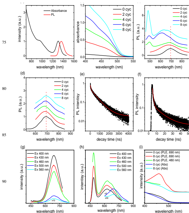
Figure 4. Optical properties of the giant QDs. (a) Absorption and PL spectra of the pure PbS QDs before cation exchange. Absorption (b) and PL (c and d) spectra of the PbS/CdS/CdS core/shell/shell QDs after different cycles of CdS shell growth. The excitation position is set at 430 nm in (c) and 520 nm in (d). (e) and (f): Fluorescence decays of QDs in toluene for sample Cyc 8, when the emission position was fixed at (690\pm 15) nm (e) and at (480\pm 7) nm (f), respectively. The excitation wavelength is \lambda_{ex}=444 nm. The red curves are the fitting of the experimental data using a three-component exponential decay. The measurements were carried out at room temperature. All the samples have the same concentration for fair comparison of the relative absorption and emission intensity. PL spectra of the QDs with (g) cycle 0 and (h) cycle 8 with tunable excitation wavelength. (i) Absorption and PLE are shown for the cycle 0 and cycle 8 samples.
