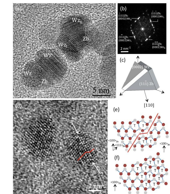
Figure 3. HREM investigation of the modifications of the PbS/CdS/CdS QDs structure after different SILAR cycles. (a) and (d) HREM micrographs of QDs after 8 and 0 SILAR cycles, respectively; (b) diffraction pattern acquired from the upper particle visible in (a); (c) schematic representation of the shape of the particles observed in (a); (e) and (f) schemes of the atomic structure of a stacking fault (SF) in the Zb structure and of the interface between Zb and Wz phases, respectively.
