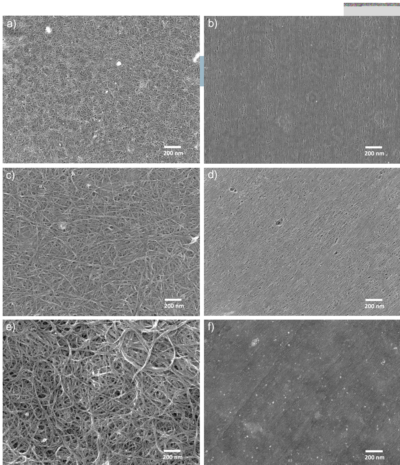
Figure 2 SEM images of (a, c, e) as-prepared nanotube films and (b, d, f) the same films after dry shear aligning, where the film in (a) and (b) was produced by slide casting of HiPco nanotubes (SuperPureTubes, NanoIntegris) dissolved in sodium polyelectrolyte solution and had an order parameter after DSA of S_{2D} = 0.41 , the film in (c) and (d) was produced by slide casting of gel sorted, small diameter metallic nanotubes made from raw HiPco material (NanoIntegris) and dissolved in sodium polyelectrolyte solution and had an order parameter after DSA of S_{2D} = 0.28 and the film in (e) and (f) was produced by vacuum filtration onto a mixed cellulose ester membrane (HAWP, Merck Millipore) of raw HiPco material suspended in 1 wt% SDS solution and had an order parameter after DSA of S_{2D} = 0.22 . In all cases DSA was conducted on the films mounted on glass slides. Absorption spectra of the three kinds of nanotube film are shown in Figure S1.
