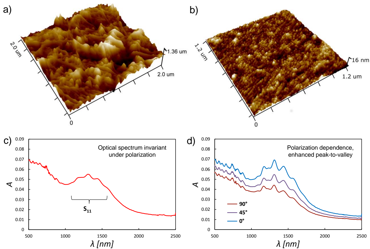
Figure 3 (a) and (b) show 3D AFM images of a vacuum filtered nanotube film before and after DSA, respectively, while (c) and (d) show the corresponding polarised optical spectra.
