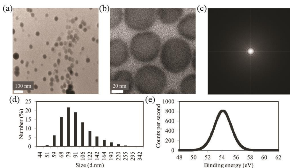
Figure 1: Characterization of Se nanoparticles via (a) TEM and (b) high resolution TEM, showing relatively mono-dispersed particles with sizes of approximately 50 nm. (c) SAED result showing the amorphous nature of Se NPs. (d) Dynamic light scattering measurement presenting size distribution of the NPs in suspension with mean diameter of approximately 80 nm. (e) XPS analysis revealing the binding energy of 54.16 eV for Se 3d peak indicating zero oxidation state of Se after coating with PVA.
