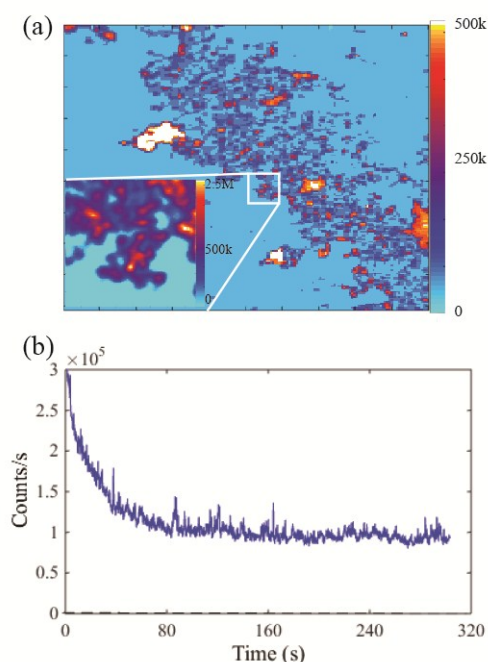
Figure 8: (a) A 50 \times 50 \mu\text{m}^2 confocal fluorescence scan (coarse) of PVA coated Se NPs on Si substrate. An excitation wavelength of 532 nm at an input power of 100 \mu\text{W} is used and the intensity scale bar is shown to the right of the figure. The inset shows a fine scan 10 \times 10 \mu\text{m}^2 fluorescence scan for PVA coated Se NPs. (b) Background subtracted emission for the characteristic PVA coated Se NP shown in the inset of (a). Black line at the base represents the low background counts.
