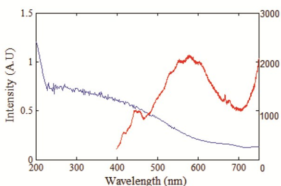
Figure 2: Measured absorption band (blue), and emission spectrum (red) indicating peak intensities at 416 nm and 580 nm. For the emission spectrum, the NPs have been excited with a UV pump at 325 nm. The intensity scale shown is in arbitrary units (A.U.).
