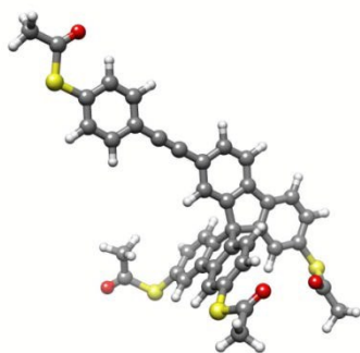
Figure 6. Ground state geometry of the SBF molecule ( \text{C}_{41}\text{H}_{28}\text{S}_4\text{O}_4 ). The acetylene end-groups are removed with one droplet of ammoniumhydroxide ( \text{NH}_4\text{OH} ) or triethylamine ( \text{Et}_3\text{N} ).
