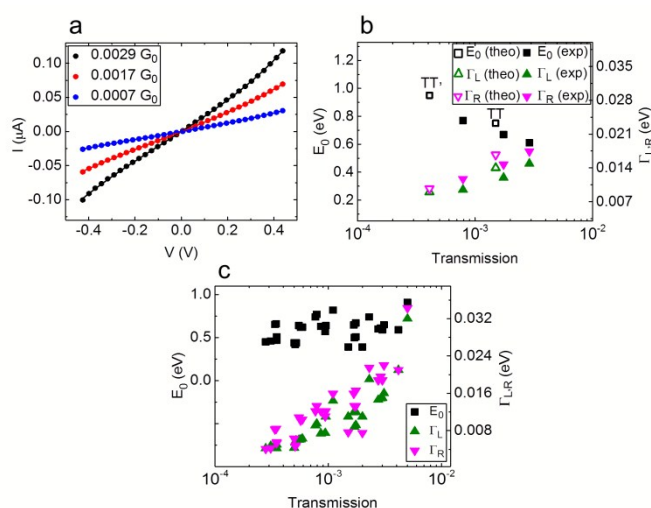
Figure 3. (a) I - V curves (symbols) of Au-SBF-Au junctions in different transmission regimes. They are fitted using the single-level model (lines) in the voltage range from -0.45 V to 0.45 V. (b) Experimental and theoretical fit parameters for a stretched contact. The best-fit parameters for the experiment are \Gamma_R = 17 meV, \Gamma_L = 14 meV, E_0 = 610 meV for G = 2.9 \cdot 10^{-3} G_0 , \Gamma_R = 15 meV, \Gamma_L = 12 meV, E_0 = 670 meV for G = 1.7 \cdot 10^{-3} G_0 , \Gamma_R = 12 meV, \Gamma_L = 9.5 meV, E_0 = 770 meV for G = 7 \cdot 10^{-4} G_0 , while the Lorentzian fit for the TT and TT' configurations from Fig. 2(d,e) yields \Gamma_R = 17 meV, \Gamma_L = 14 meV, E_0 = 760 meV for TT and \Gamma_R = 10 meV, \Gamma_L = 9 meV, E_0 = 950 meV for TT'. (c) The position of the molecular level E_0 , left axis, black squares) and the level broadenings ( \Gamma_R and \Gamma_L , right axis, green and magenta triangles) are obtained by fitting the I - V curves in the transmission range of the inclined conductance step.
