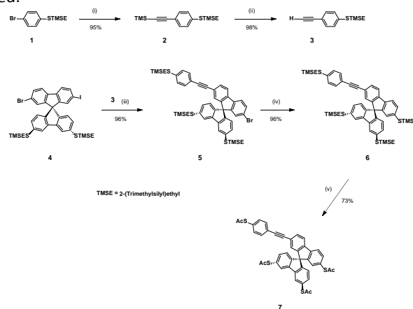
Scheme 1. Synthesis of spirobifluorene derivative 7 . Reagents and conditions: (i) Trimethylsilylacetylene, PdCl 2 (PPh 3 ) 2 , CuI, Et 3 N; (ii) K 2 CO 3 , MeOH, THF; (iii) 3 , PdCl 2 (PPh 3 ) 2 , CuI, Et 3 N; (iv) TMS(CH 2 ) 2 SH, Pd 2 (dba) 3 , XPhos, iso -Pr 2 EtNH, dioxane, Δ; (v) AgBF 4 , AcCl, CH 2 Cl 2 .
