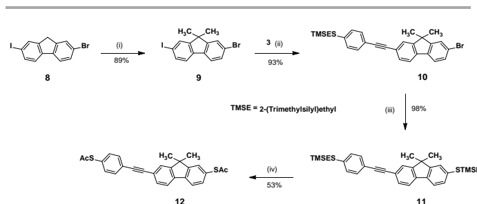
Scheme 2. Synthesis of fluorene derivative 12 . Reagents and conditions: (i) a) tert -BuOK, THF, b) CH 3 I; (ii) 3 , PdCl 2 (PPh 3 ) 2 , CuI, Et 3 N; (iii) TMS(CH 2 ) 2 SH, Pd 2 (dba) 3 , XPhos, iso -Pr 2 EtNH, dioxane, Δ; (iv) a) TBAF, THF, b) AcCl.
