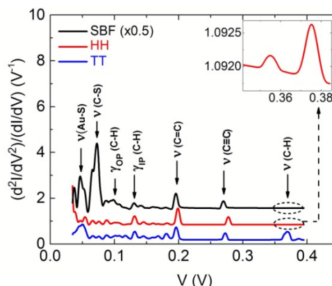
Figure 5. Calculated IET spectra for SBF, HH, and TT configurations. The spectra are offset for better visibility. The inset shows the magnified part of the IET spectrum for HH in the voltage range of 0.34 to 0.39 V, where the peaks have a lower intensity compared to the rest of the peaks and compared to the TT configuration.
