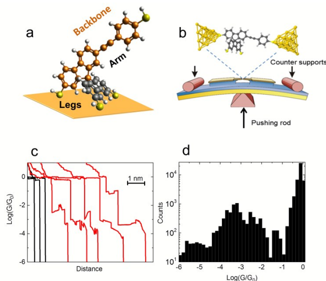
Figure 1. (a) Geometry of the studied SBF molecule introducing the terms “legs”, “arm”, and “backbone”. The hydrogen atoms at the outer ends of the legs and the arm are removed when establishing contact to the metal electrodes. (b) Sketch of the MCBJ setup. The upper part shows a possible junction geometry, where the sulphur atoms at both ends bind to a hollow site of the pyramidal Au electrodes. (c) Conductance-distance traces measured without molecules (black) and with SBF molecules (red). (d) Conductance histogram of Au-SBF-Au molecular junctions.
