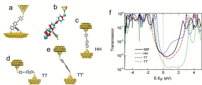
Figure 2. (a) The SBF molecular junction on an Au(111) surface contacted by an Au tip. (b) Dominant transmission eigenchannel incoming from the bottom electrode, evaluated at the Fermi energy for the SBF molecule in junction (a). The backbone of the molecule connected to pyramid-shaped electrodes in (c) HH and (d) TT positions. (e) Stretched TT junction, TT'. (f) Computed transmission curves for the SBF molecule and its backbone in HH, TT, and TT' configurations in the DFT+ \Sigma framework. The vertical dashed black line indicates the Fermi energy E_F .
