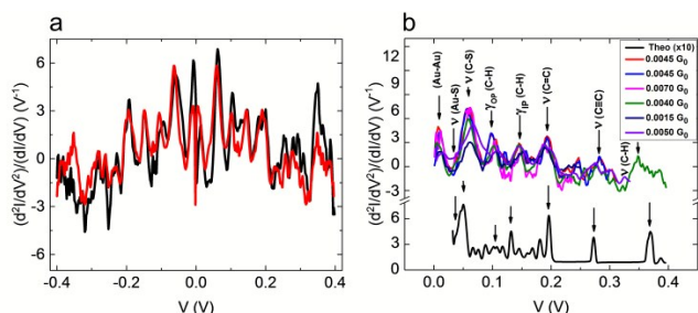
Figure 4. (a) Experimental IET spectrum of a Au-SBF-Au junction (black) with a conductance of 4 \cdot 10^{-3} G_0 (corresponding to the green curve in panel (b)) shown together with a symmetrized curve (red) with respect to the bias polarity. (For negative bias polarity the sign of d^2I/dV^2 has been inverted for better illustrating the symmetry.) (b) Comparison of experimental (coloured lines) and theoretical (black line, TT position) IET spectra. The arrows show the peak positions in the experimentally and theoretically obtained spectra.
