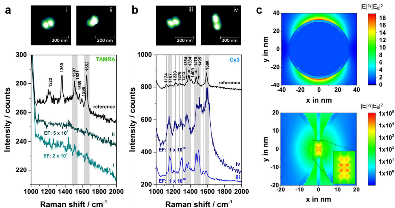
Figure 5. Experiments at the single-molecule level. (a) Correlated AFM and Raman study for structure 4a with two (dimer i) or only one (dimer ii) TAMRA molecule incorporated. In both cases peaks arising from TAMRA have been detected (highlighted in grey). (b) Analogue experiment to a) by using a single Cy3 as analyte molecule (structure 4b ). Several Cy3 bands are visible in the SERS spectra of both dimers iii and iv (highlighted in grey). Additionally, the dotted lines mark spectral positions of Cy3 which can either be detected for dimer iii or dimer iv. SERS experiments were performed with laser excitation at 532 nm, laser power of 400 – 500 \mu\text{W} and 10 s integration time. (c) FDTD calculations showing the distribution of the electromagnetic field enhancement that can be expected for a single 60 nm AuNP (top) as well as for a dimer consisting of two 60 nm AuNPs with a 2.5 nm silver shell (below). The dimer is separated by the 2 nm thick DNA origami template that is arranged concentrically in the simulation. For excitation a 532 nm laser line is assumed.
