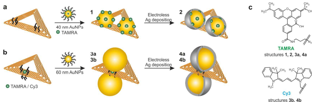
Figure 1. Formation of AuNP dimers using DNA origami substrates. The attachment process is realized by DNA hybridization between ssDNA capture strands protruding from the substrate and the complementary ssDNA coating of the AuNPs. (a) Two 40 nm AuNPs coated with the dye-modified sequence 5'-(TTT) 4 TX-SH-3' (X = TAMRA) are attached to one side of the DNA origami template resulting in structure 1 with an estimated gap size of 14 nm. Subsequent silver enhancement leads to Au-Ag-core-shell NPs with a decreased gap size (structure 2 ). (b) For single-molecule measurements one dye molecule (either TAMRA or Cy3) is incorporated in the DNA origami template. The attachment of two 60 nm AuNPs to different sides of the DNA origami ensures the position of the dye to be exactly in the hot spot (structures 3a , 3b ). Subsequent addition of a silver layer results in structures 4a or 4b . (c) Raman reporter molecules used in the present study with the covalent connection between dye and ssDNA marked in both molecular structures. Structures 1 , 2 , 3a and 4a are functionalized with TAMRA whereas structures 3b and 4b contain a Cy3 modification.
