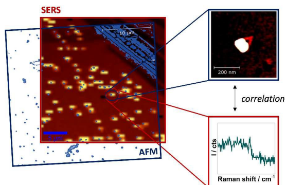
Figure 2. Illustration of correlated AFM and SERS imaging. AFM and SERS images are superimposed using a scratch on the Si as a marker in order to correlate structural and chemical information. In this way SERS signals can clearly be assigned to defined structures (the laser spot diameter is approximately 1.3 \mu\text{m} ). For better visualization the large scan-size AFM image is shown in transparent colors.
