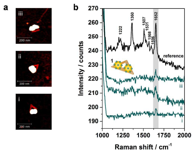
Figure 3. Single nanostructure correlations of 40 nm AuNP dimers covered with TAMRA-modified ssDNA (structure 1). (a) AFM images of three individual DNA-AuNP hybrids. (b) SERS spectra of the nanostructures i–iii showing the most prominent TAMRA peak at 1652\text{ cm}^{-1} (cyan spectra). For comparison a reference spectrum containing characteristic TAMRA bands at 1222, 1360, 1507, 1531, 1568, 1596 and 1652\text{ cm}^{-1} is shown (black spectrum). The number of TAMRA molecules contributing to each of the spectra i–iii is estimated to be approximately 40. SERS experiments were performed with laser excitation at 532 nm, laser power of 900 – 1000 \mu\text{W} and 2 s integration time.
