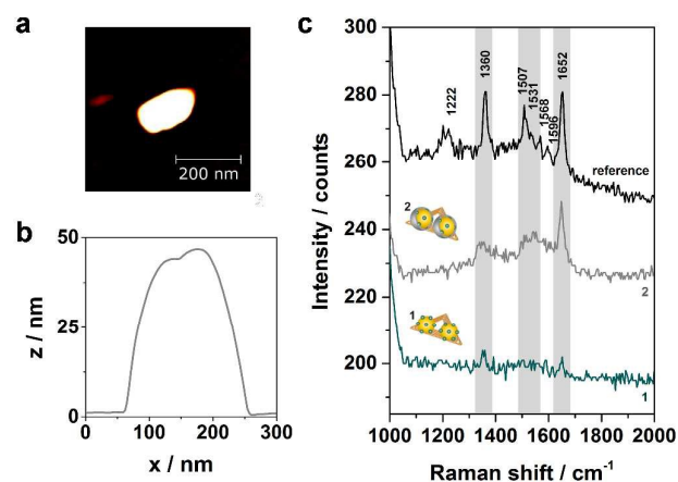
Figure 4. Comparison of correlated AFM images and SERS spectra before and after the silver enhancement process. (a) AFM image of one selected DNA-AuNP hybrid with silver shell (structure 2 ) after 3 min of incubation (LI silver). (b) The height profile of the dimer shown in a) indicates the growth of the silver shell. (c)
