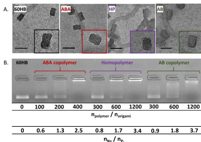
Figure 4. A) TEM micrographs showing (left to right) native origami (60HB), PDMAEMA-PEG-PDMAEMA-coated origami (ABA) with n_{\text{polymer}}/n_{\text{origami}}=200 , PDMAEMA-coated origami (HP) with n_{\text{polymer}}/n_{\text{origami}}=600 and PEG-PDMAEMA-coated origami (AB) with n_{\text{polymer}}/n_{\text{origami}}=600 . B) Native 60HB origami (leftmost lane) was run in an agarose gel along with 60HB-polymer complexes. Amine to phosphate ratio is denoted as ( n_{N^+}/n_{P^-} ).
