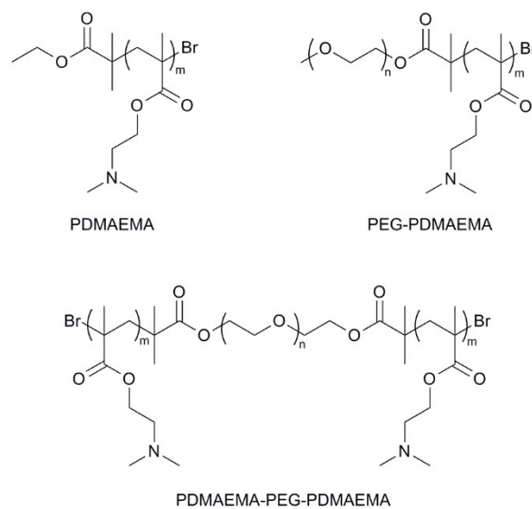
Figure 2. Three polymers were prepared utilizing Atom Transfer Radical Polymerization (ATRP) technique. Homopolymer PDMAEMA was prepared using commercial ATRP initiator ethyl \alpha -bromoisobutyrate. The copolymers were synthesized using the PEG-macroinitiators. Two separate copolymer structures were synthesized, PDMAEMA-PEG (AB-type) and PDMAEMA-PEG-PDMAEMA (ABA-type).
