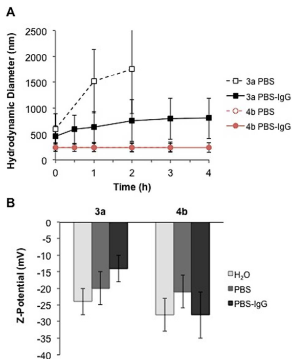
Fig. 7. (A) Temporal evolution of the hydrodynamic diameter of particles 3a and 4b , dispersed in phosphate buffer (open symbols) and phosphate buffer plus IgG (solid symbols). (B) Z-potential values of the particles before and after incubation with IgG.
