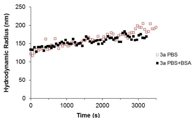
Fig. 6. Time resolved dynamic light scattering of dilute 3a nanoparticle suspensions in the presence (solid black symbols) and absence (open red symbols) of BSA. The intensity-weighted R_h of the nanoparticle aggregates was calculated by non-linear least squares fitting of the second order cumulants (ALV software).
