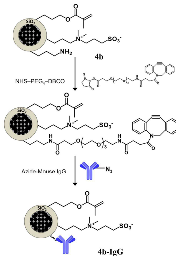
Fig. 8. Modification of the multifunctional zwitterion-bearing particles 4b with a strained alkyne (DBCO) that allows the covalent immobilization of an antibody (mouse IgG) by means of alkyne-azide click chemistry, along with a reduced nonspecific adsorption over the particles surface.
