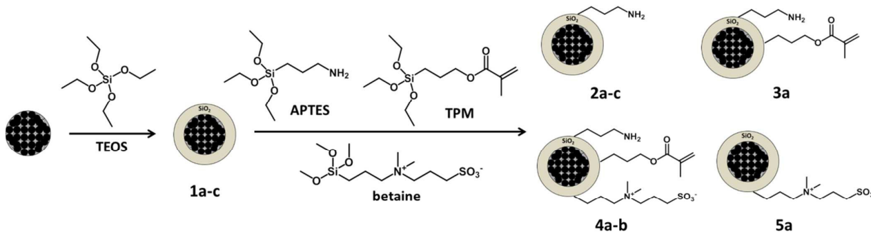
Fig. 2. An initial silica shell is formed from TEOS around the hybrid particles. Afterwards, the amino, alkene and zwitterion functional groups are introduced into the silica surface using the APTES, TPM, and betaine organosilanes, respectively. Monofunctional (amino 2a-c , zwitterion 5a ), bifunctional (amino/alkene 3a ) and trifunctional (amino/alkene/zwitterion 4a-b ) nanoparticles were synthesized.
