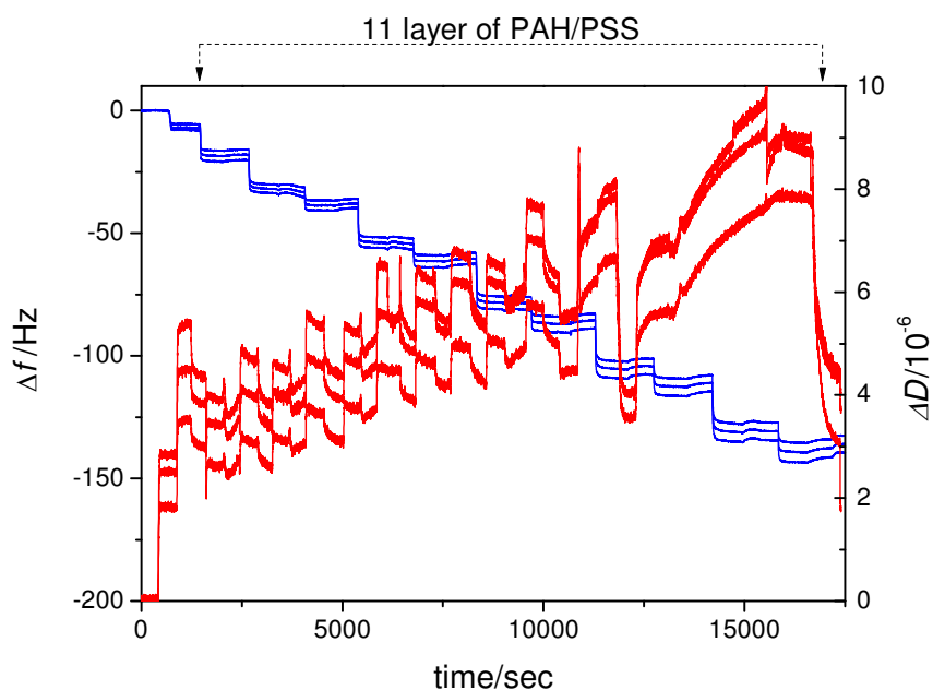
Figure S2. Frequency (blue curves) and dissipation (red curves) changes monitored during the PEM deposition of the assembly of 11 layer of PAH/PSS.
