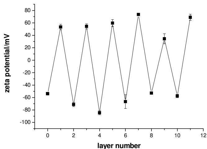
Figure S1. Zeta potential changes during the layer-by-layer coating of silica particles. 3 \mu\text{m} sized silica particles were coated with a multilayer of polyelectrolytes (PAH/PSS) 5,5 . The coating with positively charged PAH and negatively charged PSS was detected by the change of the zeta potential. The zeta potential was measured in 1 mM Tris buffer (pH 7).
