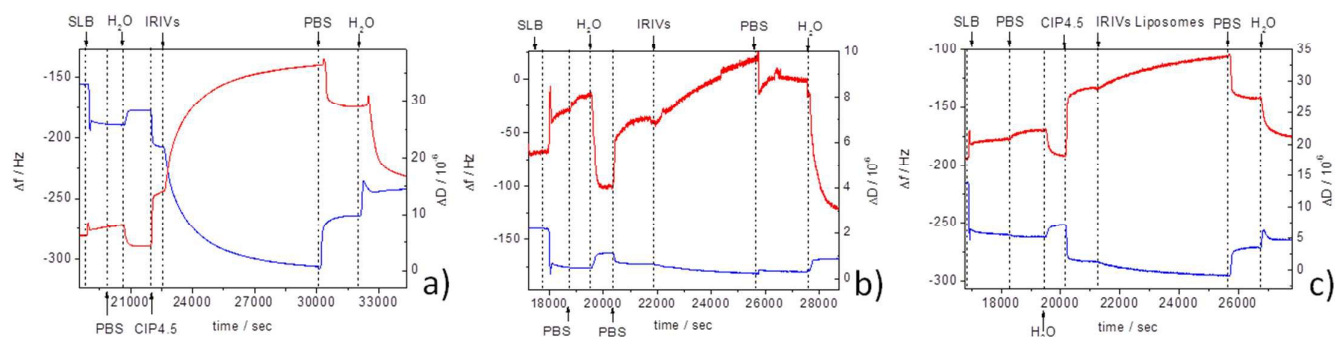
Figure 6. Frequency (blue) and dissipation (red) curves measured by QCMD for the formation of phospholipid bilayer deposited on a PEM of 11 layer of PAH/PSS and later exposed to a) IRIVs in acidic pH (CIP 4.5), b) IRIVs in neutral pH (PBS 7.4) and c) protein free liposomes with the same lipid composition and content as IRIVs in acidic pH (CIP 4.5).
