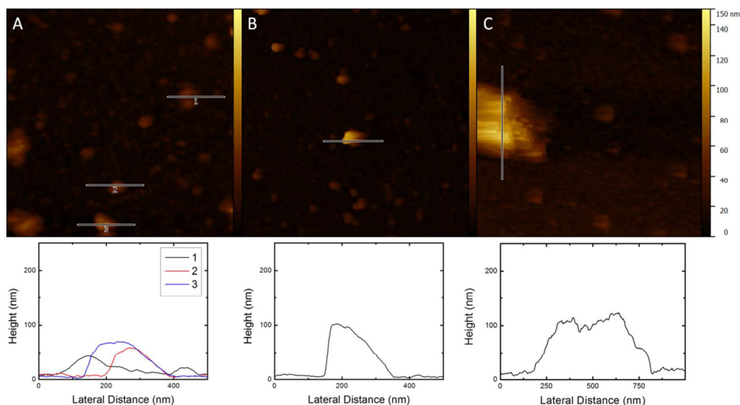
Figure 7. AFM images ( 2 \times 2 \mu\text{m} ) acquired in 1.5 mM NaCl (liquid mode) of (PAH/PSS) 5.5 PC:PS lipid bilayer membrane after addition of a) IRIVs in pH 4.5 or b) IRIVs in pH 7.4 and c) protein free liposomes in pH 4.5. Bottom panels display roughness profiles taken as cross sections of above images.
