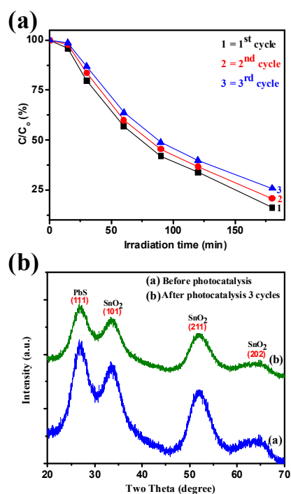
Figure 11 (a) Reproducibility of the photocatalytic decomposition of RhB using fresh (cycle 1) and recycled (cycles 2 and 3) \text{SnO}_2\text{-PbS} under visible light and (b) XRD patterns of \text{SnO}_2\text{-PbS} nanocomposite before and after these tests.
