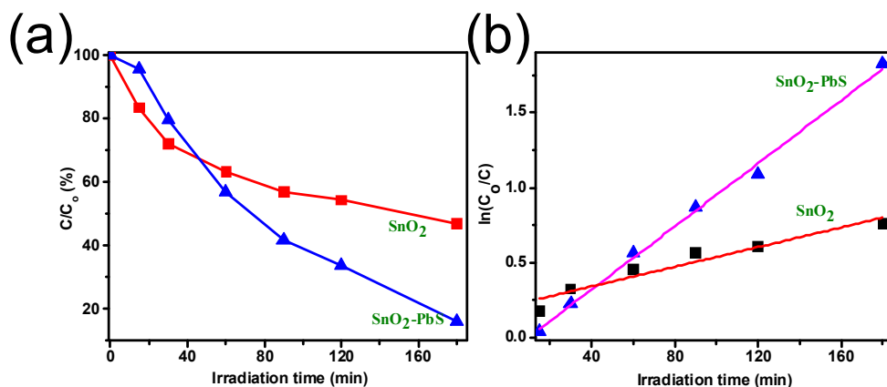
Figure 10 (a) Plot of C/C_0 (%) (where C_0 and C are the concentrations of dye before and after irradiation, respectively) for RhB as a function of visible light irradiation time in the presence of \text{SnO}_2 NPs and \text{SnO}_2\text{-PbS} nanocomposites. (b) Plot of \ln(C_0/C) as a function of visible light irradiation time.
