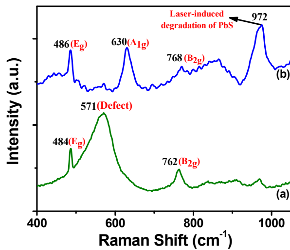
Figure 6 Raman spectra of (a) SnO 2 NPs and (b) SnO 2 -PbS nanocomposites.
