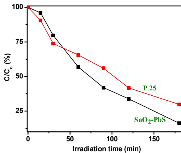
Figure 14 A comparison of C/C_0 (%) as a function of irradiation time for RhB solutions treated with SnO 2 -PbS nanocomposite and P25 (5.0 mg in either sample).
