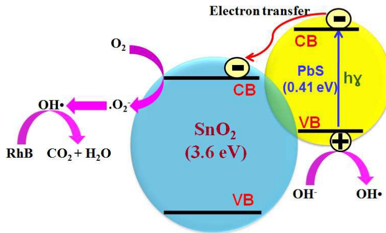
Figure 12 Model for the high photocatalytic activity and stability of SnO 2 -PbS nanocomposites.
