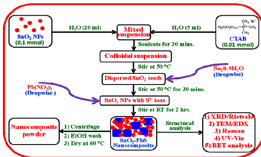
Figure 1 Synthetic scheme for the preparation of SnO 2 -PbS nanocomposites.
