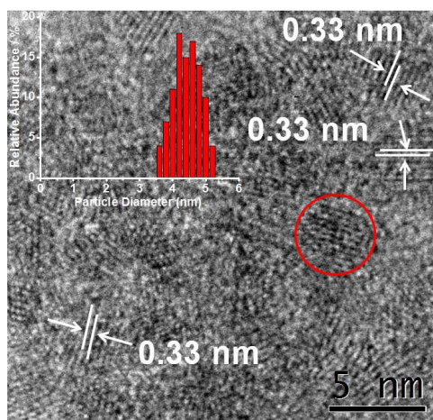
Figure 4 A representative HRTEM image of SnO 2 NPs indicating measured distances between the lattice planes and the particle size distribution for the sample (top left). The area in the red circle was subjected to FFT (see ESI Figure S6b).
