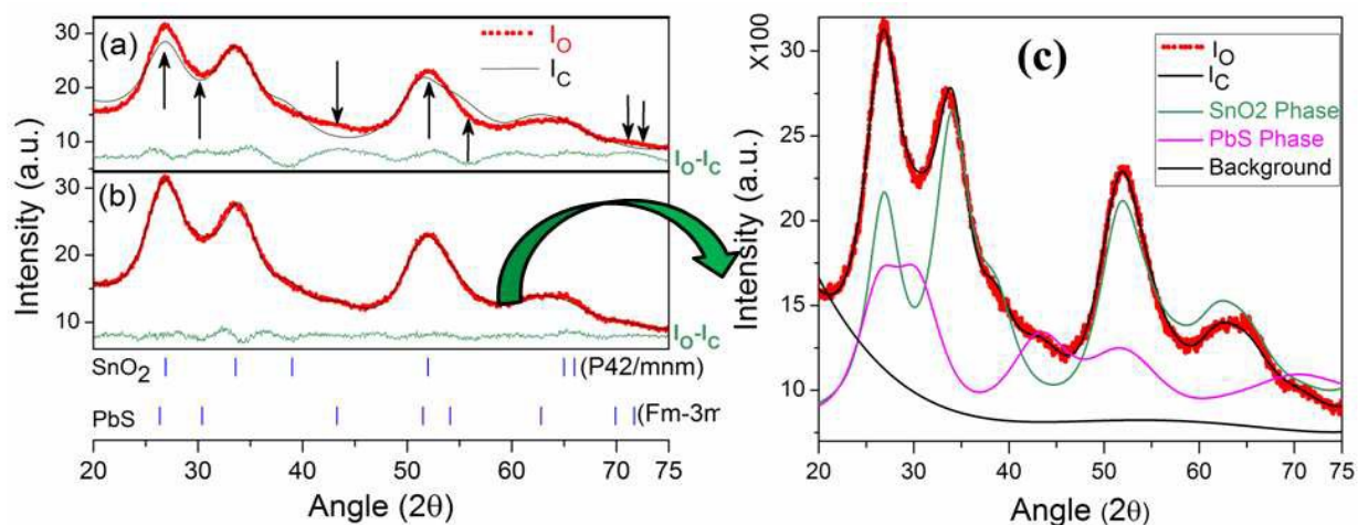
Figure 3 Typical Rietveld refinement output pattern for SnO 2 -PbS nanocomposites employing (a) tetragonal SnO 2 phase only and (b) both tetragonal SnO 2 and cubic PbS phase. (c) The contribution of tetragonal SnO 2 , cubic PbS and background to the XRD pattern for SnO 2 -PbS nanocomposites.
