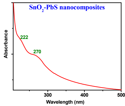
Figure 8 UV-Vis absorption spectrum of SnO 2 -PbS nanocomposites in aqueous solution.
