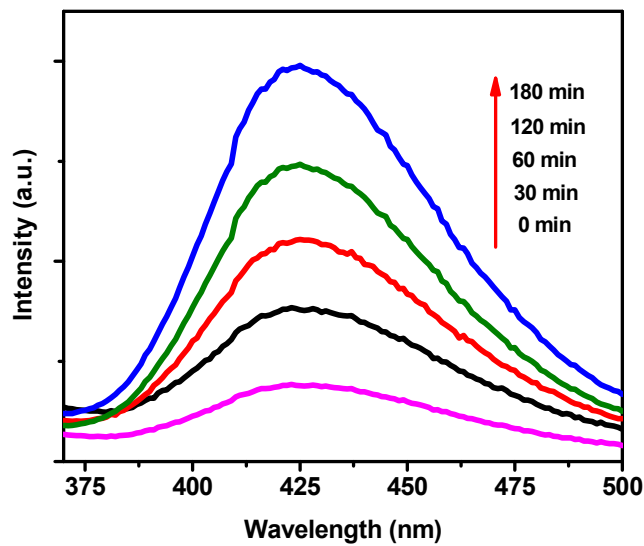
Figure 13 Fluorescence spectral changes measured during illumination of SnO 2 -PbS nanocomposite in a basic solution of TA (excitation at 315 nm).
