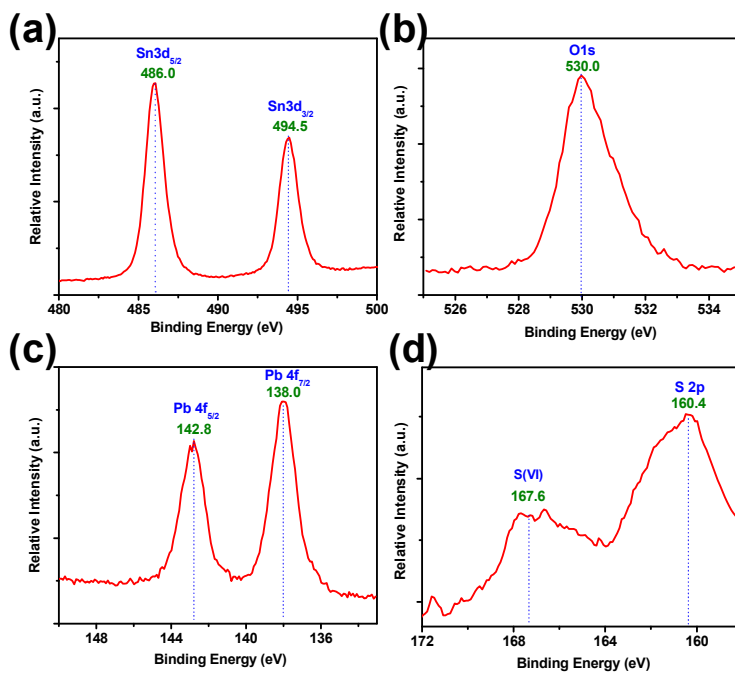
Figure 7 XPS data for SnO 2 -PbS nanocomposites: binding energy spectra for Sn3d (a), O1s (b), Pb4f (c), and S2p (d).
