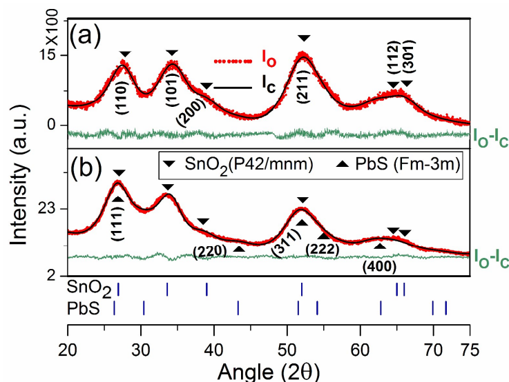
Figure 2 Observed ( I_0 ) and simulated ( I_c ) XRD patterns (indexed) of (a) SnO 2 NPs and (b) SnO 2 -PbS nanocomposites. The green lines represent I_0 - I_c . Vertical markers corresponding to reflections from individual phases are shown in blue.
