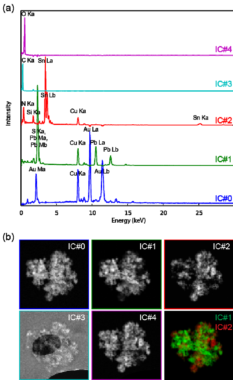
Figure 5 ICA results obtained from an EDX spectrum image of a SnO 2 -PbS nanocomposite structure. (a) independent component spectra containing the X-ray lines for the elements present (Au and Cu attributable to grid and sample holder). Independent component maps (b) IC#0-#4 are interspersed throughout the region. IC#1 represents a Pb rich phase, IC#2 a Sn rich phase, and IC#3 the carbon supporting film. Bottom right is an artificially coloured overlay of the IC#1 (green) and IC#2 (red) maps.
