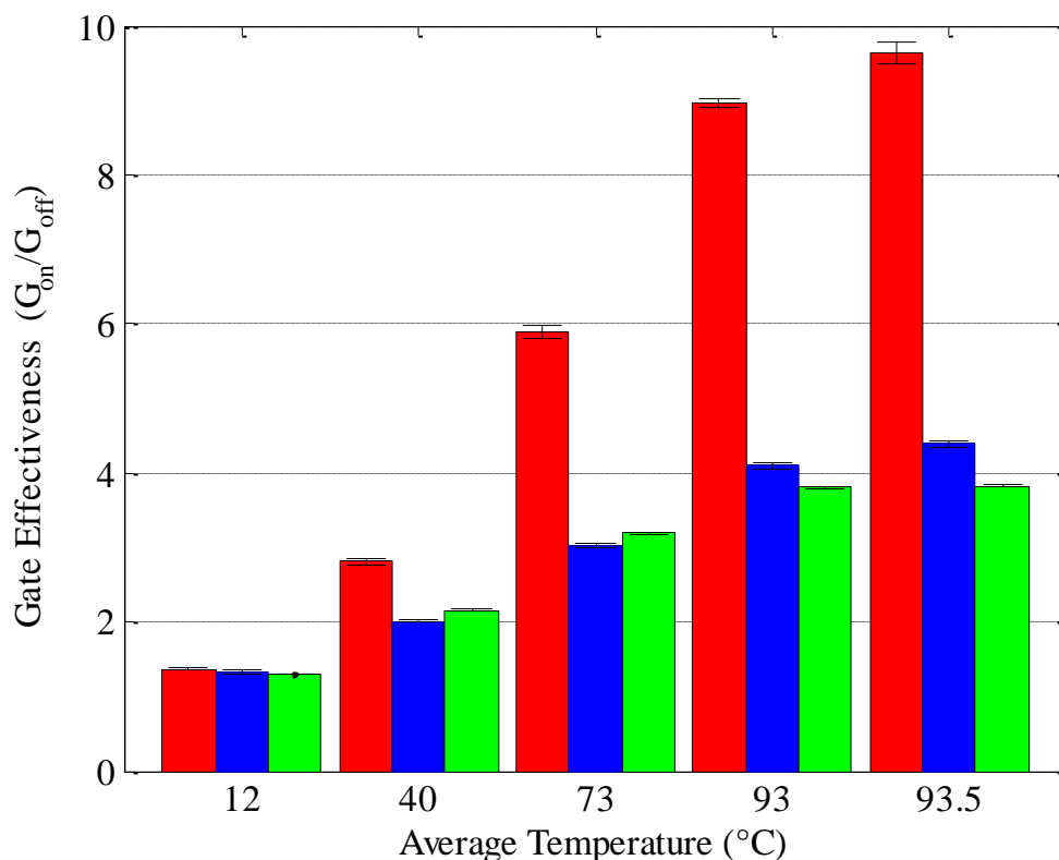
Figure 4. Effect of wall surface charge on the gate effectiveness. The figure compares the gate effectiveness for a 1 mM potassium chloride solution at pH=7 (red) to a solution of the same concentration and pH=4 (blue) while the solution at 1 M (green) shows the bulk behavior. At pH=4, the wall surface charge is low and consequently the sensitivity of the conductance of the nanochannel to the temperature is lower. At this condition, the increase of the nanochannel conductance is close to the one of the bulk. The nanochannel length is 110 \mu\text{m} while the width of the gate is only 72 \mu\text{m} . The error bars show the 95% confidence interval for 5 measurements.
