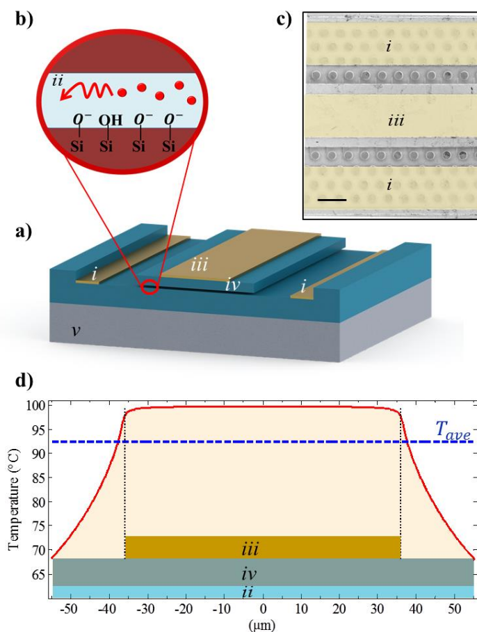
Figure 1. a) Schematic of a thermally gated device mounted on a cool plate. The cool plate keeps the temperature at the bottom of the device at 3 \pm 1 °C. The impedance of the nanochannel is screened using the integrated platinum electrodes close to the entrance of the nanochannel. i : Impedance measurement electrodes ii : Nanochannel. iii : Thermal gate. iv : Dielectric layer. v : Temperature controlled cool plate. b) Schematic of the ionic transport inside a nanochannel (110 μm in length, 3 μm in width and 40 nm in height). Heating up the nanochannel enhances the ionic transport by increasing the wall surface charge. c) Scanning electron micrograph (SEM) of the fabricated device shows the relative position of a thermal gate electrode 72 μm in width and the measurement electrodes. The scale bar is 50 μm. d) Temperature distribution (red solid line) inside the nanochannel while the gate electrode is at 100 °C. the average temperature (blue dashed line) is about 92 °C.
