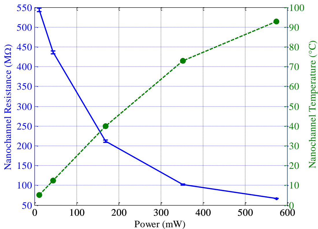
Figure 2. Evolution of resistance and average temperature of the nanochannel at different applied powers for a 1 mM potassium chloride solution. Increasing the power decreases the nanochannel resistance by heating up the nanochannel. The average temperature is estimated by calibrating the resistance of the nanochannel at 1M where change of conductivity is dominant by ion mobilities. 10 The nanochannel length is 110 \mu\text{m} while the width of the gate is only 72 \mu\text{m} .
