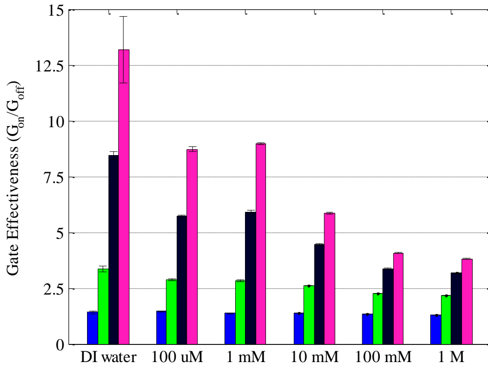
Figure 3. The gate effectiveness for \Delta T=90^\circ\text{C} (pink), \Delta T=70^\circ\text{C} (black), \Delta T=37^\circ\text{C} (green), \Delta T=10^\circ\text{C} (blue) of maximum applied power at different ionic concentrations. The power applied to a 2.5 mm in length gate electrode is 570 mW at \Delta T=90^\circ\text{C} . The gate effectiveness is higher at low ionic concentrations. The nanochannel length is 110 \mu\text{m} while the width of the gate is only 72 \mu\text{m} . The error bars show the 95% confidence interval for 5 measurements.
