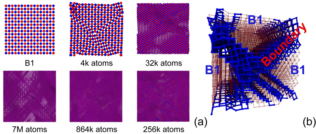
FIG. 3. (a) Morphologies of B1 grain boundaries obtained from supercell magnification of the B33 intermediate of Fig. 1 (original cell (4k, 3960 atoms), 2x2x2 (32k, 31680 atoms), 4x4x4 (256k, 253444 atoms), 6x6x6 (864k, 855360 atoms) and 12x12x12 (7M, 6842880 atoms)), after NpT-MD calculations. (b) Detailed representation of the smallest grain obtained (4k): regions of coherent B1 structure are separated by B1 grain boundaries. A strong anisotropy can be noticed, as B1 percolates in one direction only (red framework), normal to the plane. The structural motif of the boundaries resembles the NiAs type structure (blue regions). Pb and Se are not differentiated to emphasise structural features.
