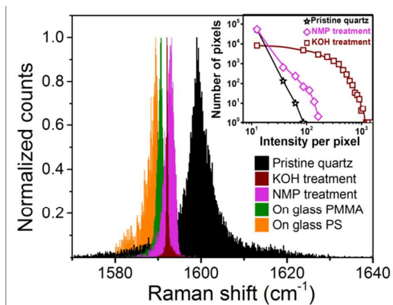
Figure 6. Histogram of G 1 -mode Raman shifts for pristine SWNT arrays, after etching with KOH (with PMMA), after transfer onto glass with PMMA or PS, and after solvent treatment with NMP only. Inset: Number of pixels versus PL intensity for pristine SWNT arrays, after etching with KOH (with PMMA) and after solvent treatment with NMP.
