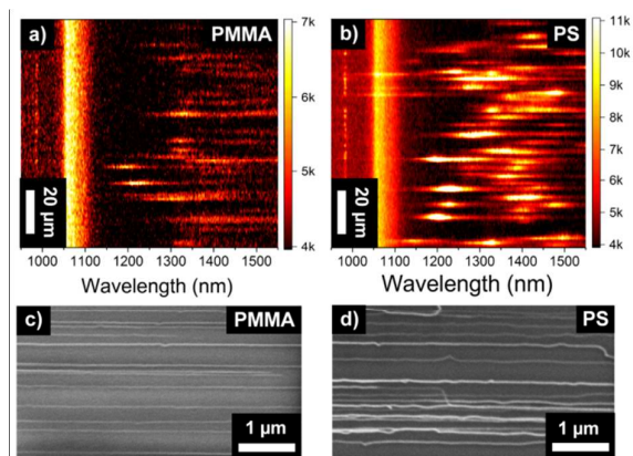
Figure 5. Comparison of hyperspectral images of multiple SWNTs transferred to a glass substrate using a) PMMA or b) PS as a transfer polymer (the signal at 1060 nm is due to the glass substrate). Corresponding SEM images of SWNT arrays transferred with c) PMMA and d) PS as polymer matrix.
