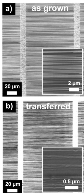
Figure 1. SEM images of SWNT arrays a) as-grown on quartz and b) transferred to annealed quartz substrates. Alignment of the SWNTs is almost completely preserved.
