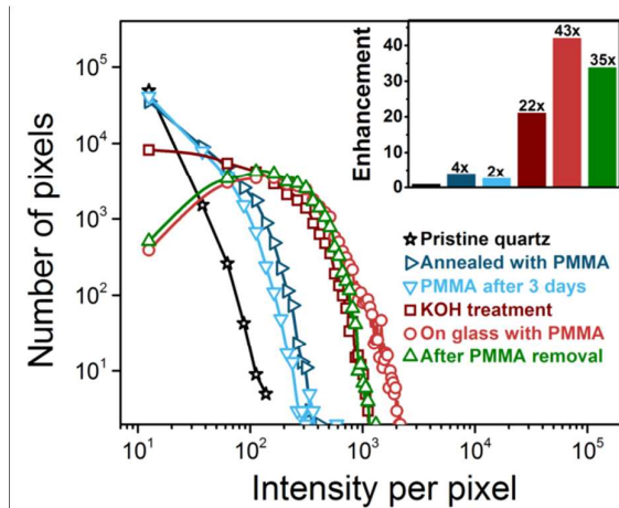
Figure 3. Influence of transfer process steps on PL characteristics: Number of pixels versus their PL intensity for SWNT arrays after every transfer process step compared to pristine SWNTs on quartz determined from analysis in the area between the catalyst lines. Inset: corresponding overall intensity enhancement versus pristine SWNTs.
