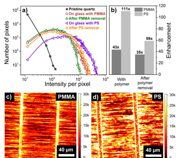
Figure 4. Impact of transfer polymer on the optical response of SWNTs: a) Number of pixels versus PL intensity for SWNT arrays transferred onto glass using PS and PMMA as a transfer polymer, with polymer and after removal of the polymer compared to pristine SWNTs on quartz. b) Corresponding overall intensity enhancement versus pristine SWNTs. PL intensity maps of SWNT arrays transferred to glass substrate using c) PMMA or d) PS as the transfer polymer.
