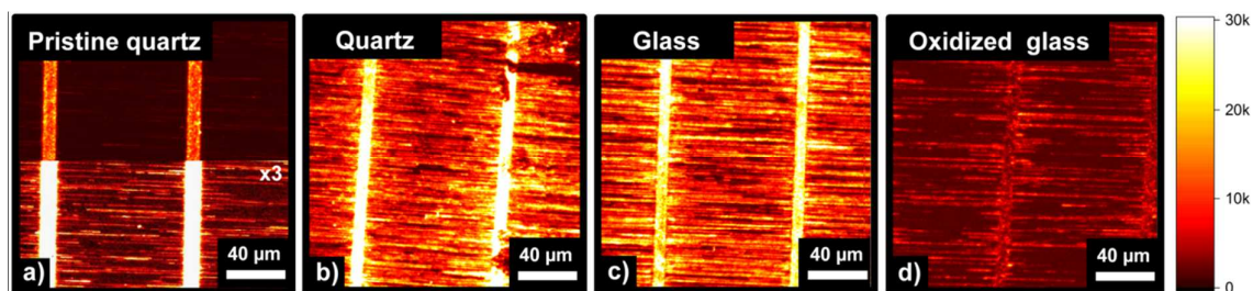
Figure 2. Comparison of PL intensity maps for different substrates: a) pristine SWNT array as-grown on quartz (intensity at the bottom part was increased three times to visualize presence of SWNTs), b) transferred to annealed quartz, c) transferred to cleaned glass and d) transferred to oxidized glass. Integrated intensity for wavelengths 0.9 - 1.6 \mu\text{m} . Excitation wavelength \lambda_{\text{ex}} = 785 \text{ nm} , excitation power P_{\text{ex}} = 35 \mu\text{W} (b-d) or 180 \mu\text{W} (a).
