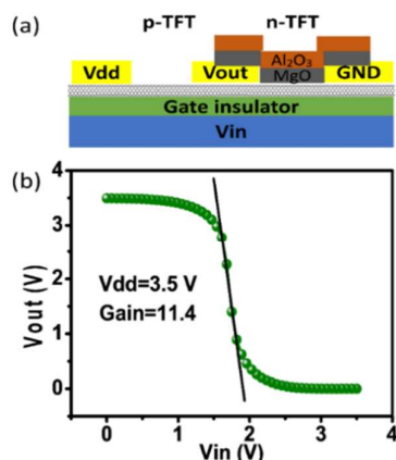
Fig. 4 (a) Schematics of a complementary inverter. (b) Transfer characteristics of the inverter. Both the channel length and channel width are 40\ \mu\text{m} for both the n-type and p-type device. The gate insulator is 40\ \text{nm}\ \text{HfO}_2 . The thickness of \text{MgO} and \text{Al}_2\text{O}_3 are 10\ \text{nm} and 30\ \text{nm} respectively.
