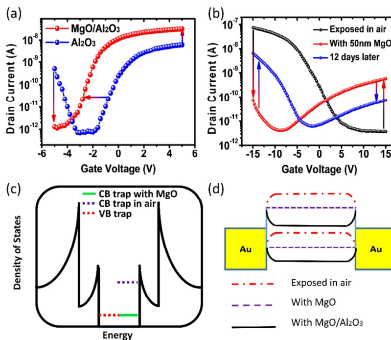
Figure 3. Mechanism of n-type CNT-TFT with MgO/Al 2 O 3 bilayer as top-gate dielectrics. (a) Transfer characteristics of CNT-TFT with single-layer ALD Al 2 O 3 (blue) and MgO/Al 2 O 3 (red) bilayer as top gate dielectrics. (b) Transfer characteristics of CNT-TFT with the channel exposed in air (black), just after deposition of 50 nm MgO (red) and 12 days after MgO deposition (blue). (c) Schematic illustration of the density of trap states near the band edge of CB and VB affected by MgO deposition. (d) Schematic of energy band diagram for the device exposed (red), with only MgO deposition (violet), and with MgO/Al 2 O 3 (black) bilayer as dielectrics.
