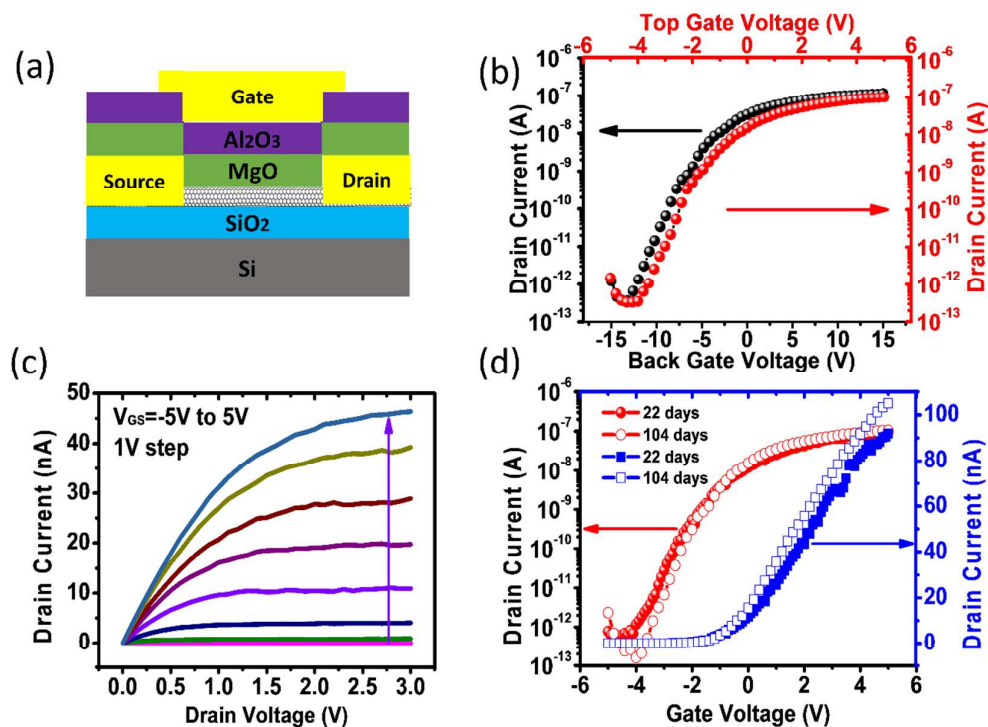
Fig. 2 Properties of the n-type TFT on silicon substrate. (a) Cross-sectional schematic of the device on silicon substrate. The thickness of MgO and Al_2O_3 are 10 nm and 30 nm respectively. The channel area is 40 \mu m \times 40 \mu m . (b) Transfer characteristics of the TFT measured at V_{DS}=2 V with the top gate (red) and back gate (black). (c) Output characteristics and (d) air stability of the device.
