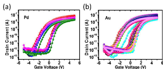
Fig. 5 Transfer characteristics of n-type CNT-TFTs with Pd (a) and Au (b) as drain/source metal contact materials measured at V_{DS}=2\ \text{V} in air. The channel dimensions are 40\ \mu\text{m} \times 40\ \mu\text{m} for all the devices.
