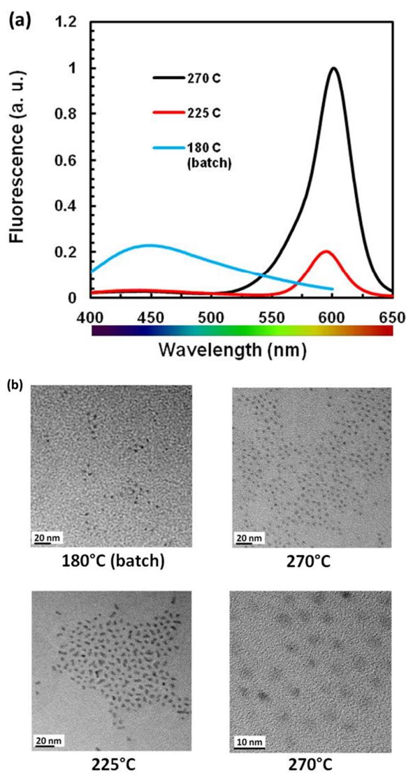
Figure 1a and 1b: (a) Fluorescence spectra of CdSe particles synthesized at varying temperatures and (b) corresponding TEM images showing wide particle size
