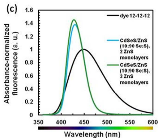
Figure 8a-c. (a) Absorbance at 1/40 dilution, (b) absorbance in arbitrary units, and (c) absorbance-normalized fluorescence in arbitrary units for CdSeS/ZnS particles with varying ZnS monolayers.
