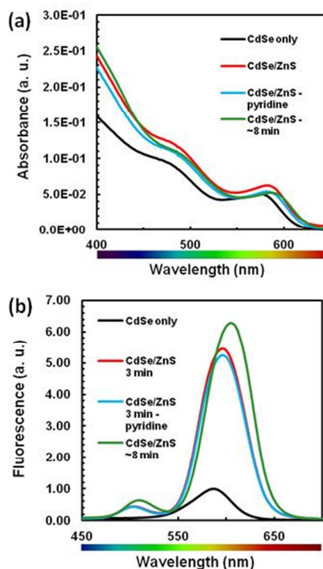
Figure 2a-b: (a) Absorbance and (b) fluorescence spectra of CdSe/ZnS quantum dots in arbitrary units with varying residence time and pyridine treatment. The pyridine-treated sample was diluted 1:1 with pyridine and then diluted to the same concentration as the standard CdSe/ZnS dots.
