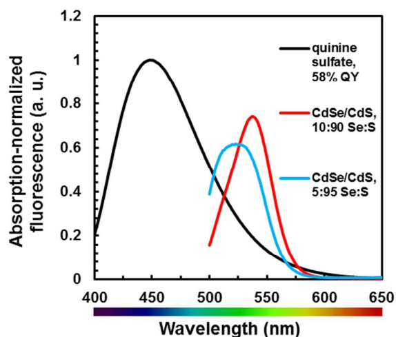
Figure 3: Absorption-normalized fluorescence for CdSe/CdS particles as a function of Se:S ratio. Excitation: 490 nm. Fluorescence below 500 nm is not shown due to proximity to the excitation signal.
