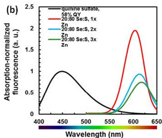
Figure 5: (a) Absorbance and (b) fluorescence spectra of CdSe/CdS/ZnS quantum dots in arbitrary units with varying ZnS shell growth amount. 1, 2, or 3 additions corresponds to ~2, 4, or 6 monolayers. Excitation: 490 nm.
