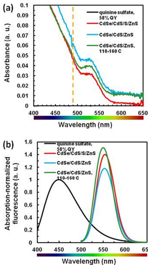
Figure 4: (a) Absorbance and (b) fluorescence spectra of CdSe/CdS/ZnS quantum dots in arbitrary units with varying shell growth procedure. Excitation: 490 nm.
