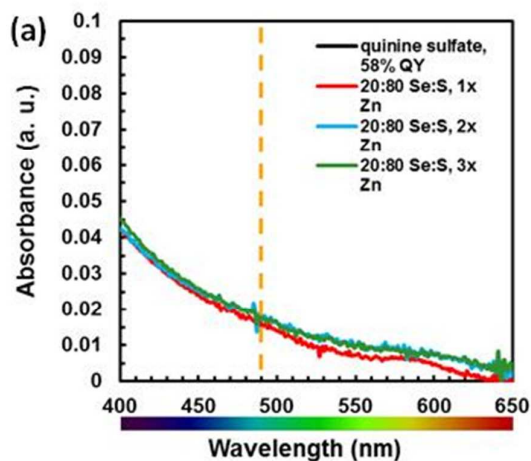
Figure 4: (a) Absorbance and (b) fluorescence spectra of CdSe/CdS/ZnS quantum dots in arbitrary units with varying shell growth procedure. Excitation: 490 nm.
