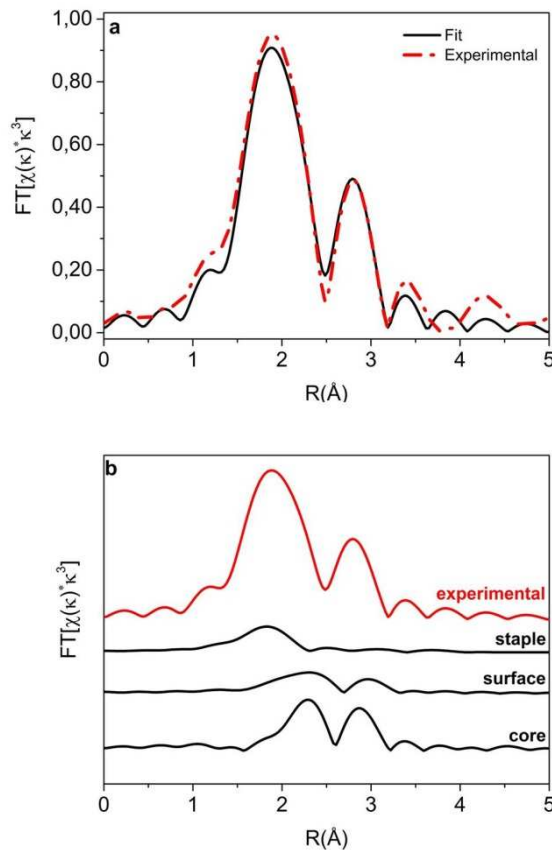
Figure 5. EXAFS spectra of \text{Pd}_2\text{Au}_{36}(\text{SC}_2\text{H}_4\text{Ph})_{24} in R space: (a) experimental and fitted spectra for a mixture of staple and core doped models. (b) Experimental and simulated EXAFS spectra for the staple, surface and core doped models
