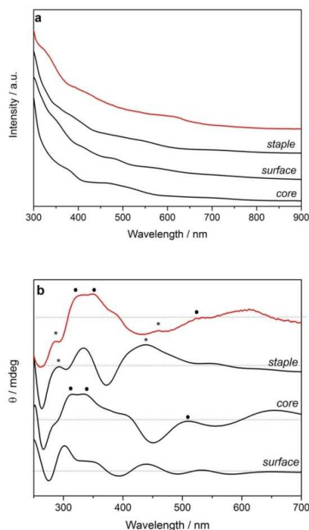
Figure 4. Comparison between experimental (red) and calculated (black) (a) absorption and (b) CD spectra of \text{Pd}_2\text{Au}_{36}(\text{SC}_2\text{H}_4\text{Ph})_{24} nanocluster. Coincident peaks between experimental and theoretical spectra are shown by asterisks (* staple model; • core model). Calculations were done for three different models (see text for more details)
