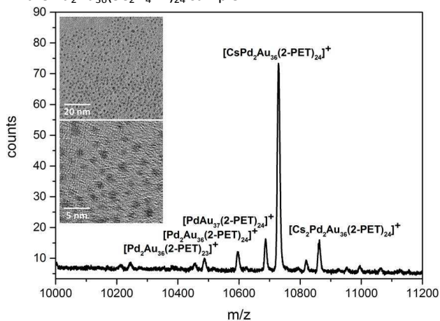
Figure 1. Positive polarization ESI-MS spectrum of \text{Pd}_2\text{Au}_{36}(\text{SC}_2\text{H}_4\text{Ph})_{24} . inset: HRTEM image from \text{Pd}_2\text{Au}_{36}(\text{SC}_2\text{H}_4\text{Ph})_{24} sample.
