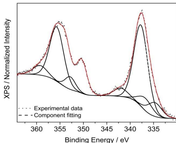
Figure 2. Au 4d and Pd 3d XP spectra of \text{Pd}_2\text{Au}_{36}(\text{SC}_2\text{H}_4\text{Ph})_{24} , experimental data are denoted in grey dots, envelop and Shirley background, and component fitting are denoted in black
