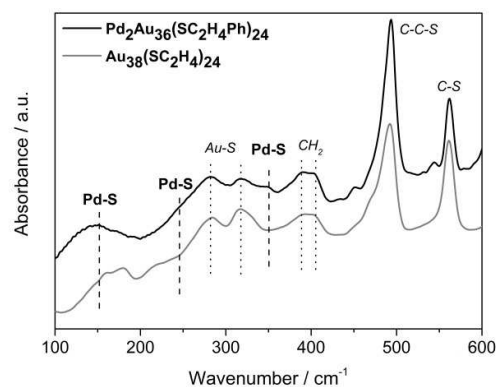
Figure 3. FIR spectroscopy of \text{Au}_{38}(\text{SC}_2\text{H}_4\text{Ph})_{24} and \text{Pd}_2\text{Au}_{36}(\text{SC}_2\text{H}_4\text{Ph})_{24} nanoclusters
