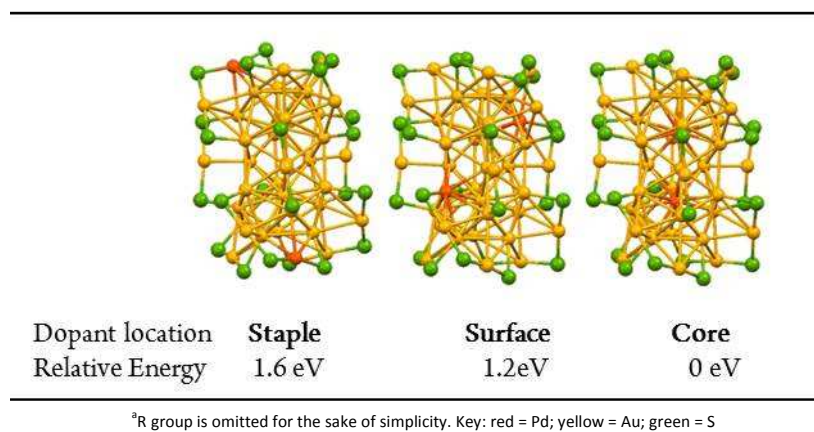
Scheme 1. Optimized structures for \text{Pd}_2\text{Au}_{36}(\text{SCH}_2\text{CH}_2\text{Ph})_{24} a
