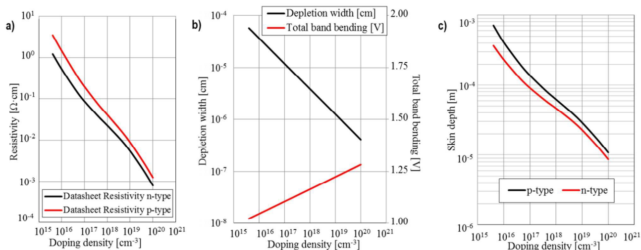
Figure 4. Physical parameters of the doping sample used in the analytical model of the tip/sample resistivity. (a) Datasheet resistivity of the doped Si sample with respect to the different n- and p-implant doping concentrations (Infineon Technologies, Germany). (b) Depletion width [cm; left scale] and total band bending [V; right scale] at different doping concentrations. (c) Skin depth [m] of p-doped and n-doped regions for different doping concentrations.
