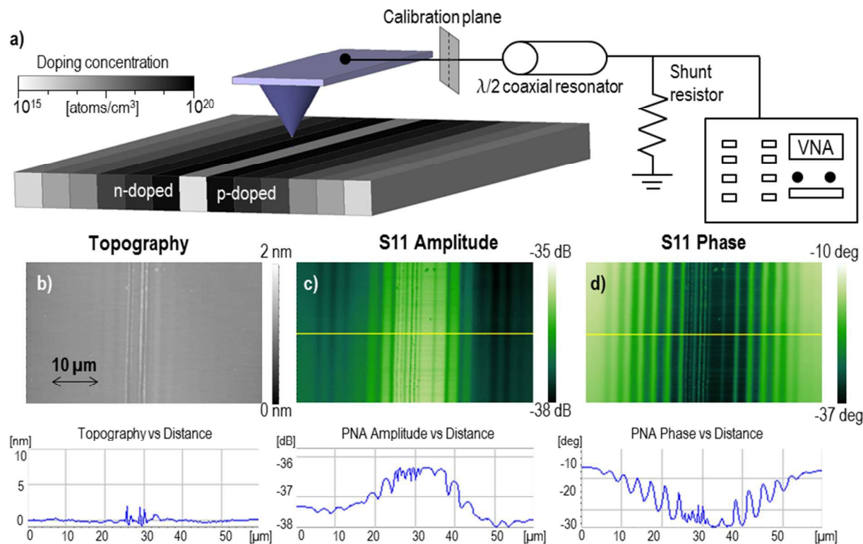
Figure 1. a) Sketch of the SMM experimental setup and of the doped Si sample with flat topography. The sample consists of 10 different n-implant areas (left region) and 10 different p-implant areas (right region), each area with a width of 2\ \mu\text{m} , with doping concentrations ranging from 4 \times 10^{15} to 1 \times 10^{20} atoms/cm 3 . The SMM raw images of this sample are shown including flat topography (b), S_{11} amplitude (c) and S_{11} phase (d). The horizontal cross-sections are given below the images.
