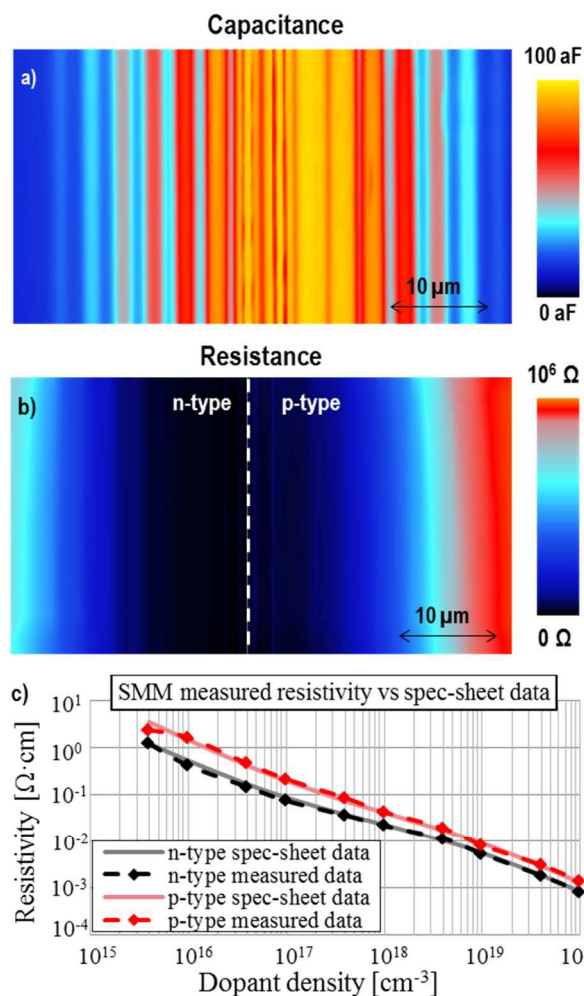
Figure 2. Calibrated SMM data including capacitance (a) and resistance (b) images. Based on the raw S_{II} amplitude and phase data (see Fig. 1) the three error parameter model was used to calibrate the complex impedance images. The doped Si sample has 10 different n- and 10 different p-implant areas (each 2 \mu\text{m} wide) with doping concentrations ranging from 4 \times 10^{15} to 1 \times 10^{20} atoms/ \text{cm}^3 . The resistivity in (c) is calculated from the calibrated resistance using a tip/sample analytical model including skin depth \delta and depletion width W_{DL} . The tip radius r was determined from the EFM dC/dz approach curve. The SMM resistivity is compared to the datasheet resistivity.
