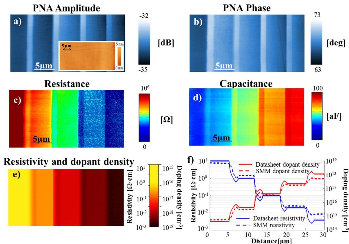
Figure 3. SMM raw data (a,b) and calibrated impedance (c,d) of the IMEC n-type Si dopant sample. The sample has a flat topography (inset in a) and different n-doped areas with doping concentrations ranging from 10^{14} to 10^{19} atoms/cm 3 . The 5 \mu\text{m} wide doping areas are separated by 1 \mu\text{m} wide bulk interface layers as observed also in the capacitance and resistance images. The resistivity and doping concentration (e) are calculated from the SMM resistance based on the tip/sample analytical model. (f) Comparison of SMM resistivity and doping concentration values to the datasheet values (provided by IMEC) determined with Secondary Ion Mass Spectroscopy (SIMS).
