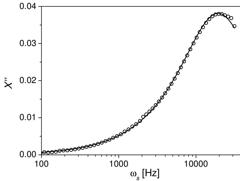
FIG. 5. Imaginary part X'' of the response function of the nanorods as a function of frequency, determined by OT (open black circles). The black line is the fit with Eq. 2 assuming a lognormal-distribution (Eq. 3) of the characteristic relaxation frequency \omega_c with \omega_c^0 = 21460 Hz and \sigma = 0.58 .
