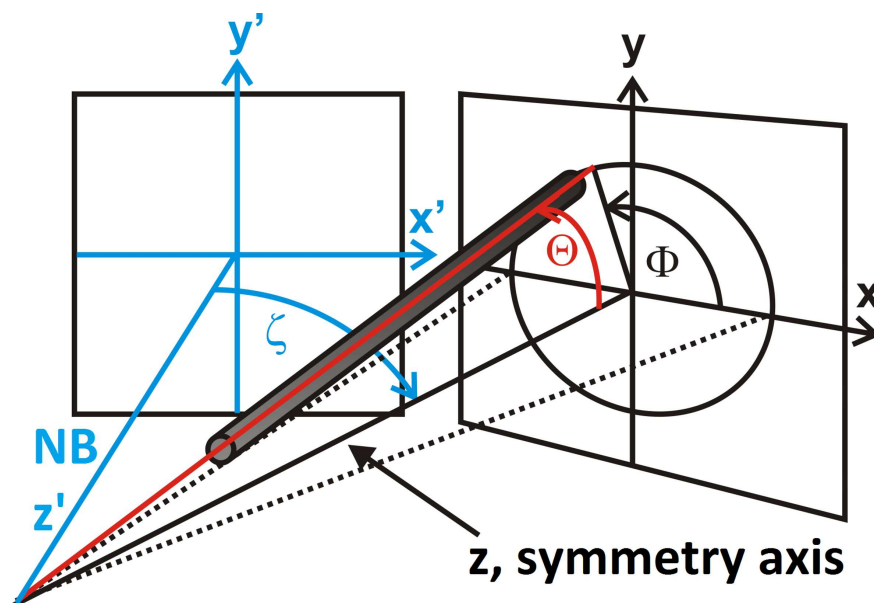
FIG. 8. Schematical illustration of the orientation of an individual nanorod with respect to the detector and definition of the relevant angles. When the ensemble is quasistatically rotated by the angle \zeta out of the neutron beam (NB, z' -direction) the z -direction is the symmetry axis of the ensemble.
