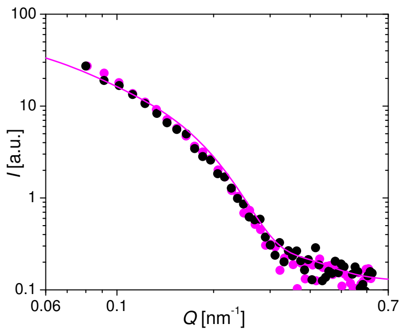
FIG. 12. Intensity after radially averaging in the horizontal sector of the time channel with minimal integrated intensity at \omega_s = 11309.7 Hz (magenta) and of the time channel with identical integrated intensity at \omega_s = 157.1 Hz (black, see Fig. 9). Full line is the simulated intensity of the ensemble when the symmetry axis is rotated by 7.8^\circ out of the neutron beam.
