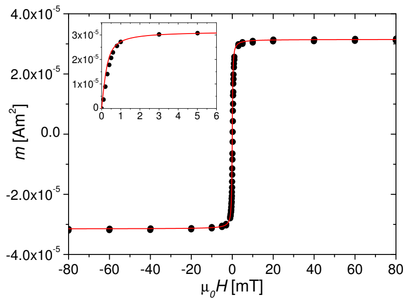
FIG. 2. Magnetization curve of the nanorod dispersion in D_2O and corresponding fit with a single Langevin function (red line) with the magnetic moment m_r = 3 \cdot 10^{-17} \text{ Am}^2 of the nanorods and the saturation moment m_S = 3.2 \cdot 10^{-5} \text{ Am}^2 of the colloidal dispersion; inset shows the upper right quadrant from 0 mT to 6 mT.
