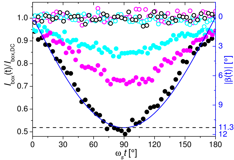
FIG. 9. Integrated intensities for sample frequencies of \omega_s = 157.1 Hz (black), \omega_s = 11309.7 Hz (magenta) and \omega_s = 18849.6 Hz (cyan) in the horizontal sector (full symbols) as well as in the vertical sector (open symbols) as a function of time. The integrated intensities were normalized to the sector area and divided by the normalized integrated intensity I_{box,DC} of the static scattering pattern in the circular area indicated in Fig. 6. Phase shifts between the signal and the magnetic field were omitted by shifting the intensity on the time-scale, so that \omega_s t = 90^\circ corresponds to the minimum and hence maximal rotation of the nanorod ensemble out of the neutron beam. The blue line is the orientation of the magnetic field vector with respect to the neutron beam as a function of time.
