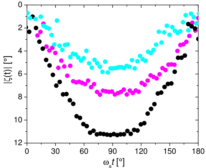
FIG. 11. Orientation of the symmetry axis of the nanorod ensemble with respect to the neutron beam for \omega_s = 157.1 Hz (black), \omega_s = 11309.7 Hz (magenta) and \omega_s = 18849.6 Hz (cyan) as a function of time.
