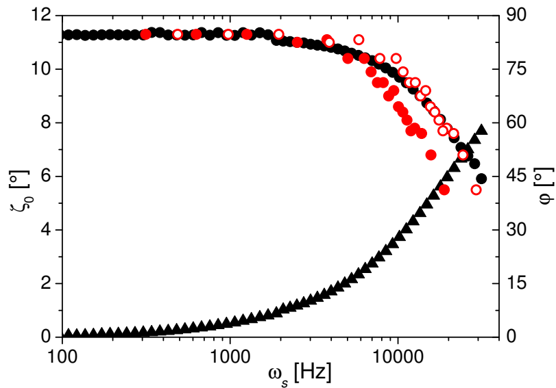
FIG. 4. Magnitude of the oscillation amplitude of the nanorods \zeta_0 (black circles) and the phase shift \varphi (black triangles) between their axes and the oscillating field vector as a function of frequency, determined by OT. The red circles are the magnitudes of the oscillation amplitudes determined by SANS. Good agreement with the results from OT is obtained, when the values are shifted by a factor of 1.5 on the frequency-axis (open red circles).
