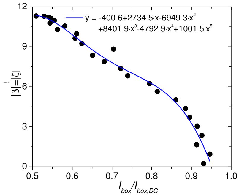
FIG. 10. Magnitude |\beta| of the orientation angle of the field vector and hence the symmetry axis of the ensemble |\zeta| as a function of the integrated intensity at \omega_s = 157.1 Hz (black). The fitting function enables to translate measured intensities into |\zeta| .
