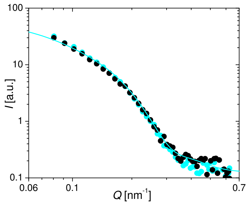
FIG. 13. Intensity after radially averaging in the horizontal sector of the time channel with minimal integrated intensity at \omega_s = 18849.6 Hz (cyan) and of the time channel with identical integrated intensity at \omega_s = 157.1 Hz (black, see Fig. 9). Full line is the simulated intensity of the ensemble when the symmetry axis is rotated by 5.5^\circ out of the neutron beam.
