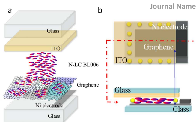
Figure 1 A schematic of Gr-ITO 10\ \mu\text{m} cell filled with nematic liquid crystal, (a) overall device operation (b) cell structure of the Gr-ITO cell.
