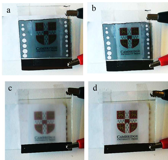
Figure 8 Test cell Gr-ITO electrodes with 10 μm spacer beads, filled with a mixture of (a,b) BL006 nematic LC with 4% black dye S428, and (c,d) BL006 with 1% RM257. (a,c) No electric field applied and (b,d) under applied electric field, 3 V μm -1 , 1 kHz.
