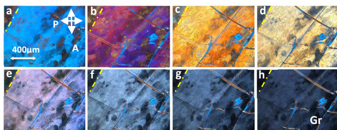
Figure 2 POM images of the 10 \mu\text{m} thick Gr-ITO switching cell under crossed polarisers. LC homeotropic alignment under applied electric field a) No field applied, (b) 0.6 \text{V}/\mu\text{m} , c) 0.75 \text{V}/\mu\text{m} , d) 0.9 \text{V}/\mu\text{m} , e) 1.5 \text{V}/\mu\text{m} , f) 1.8 \text{V}/\mu\text{m} , g) 2.1 \text{V}/\mu\text{m} and h) 3 \text{V}/\mu\text{m} field (yellow dotted line is the edge of the graphene sheet (Gr) and scale bars: 400 \mu\text{m} ).
