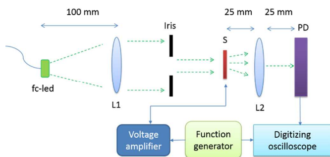
Figure 3 Experimental setup used to measure light scattering characteristics of the test cells. L1: 100 mm focal length lens, L2: 25 mm focal length lens, S: mounted sample cell, LED: 532 nm cantered, fibre coupled led light source, the iris aperture was set to 4 mm, and a collimated beam of light was incident on the sample.
