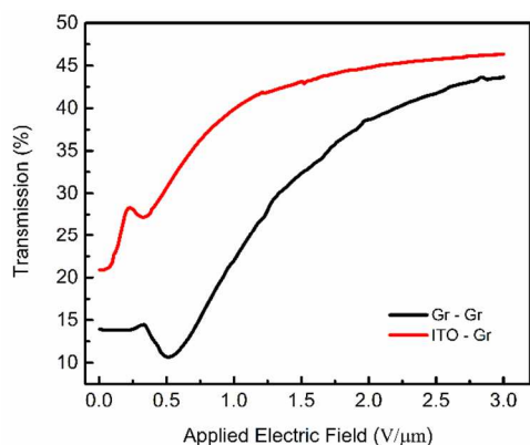
Figure 7 Transmission vs. applied electric field traces for 10 μm Gr-Gr and ITO-Gr devices filled with BL006 N-LC+4% black dye.
