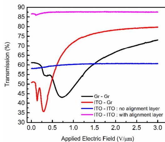
Figure 4 Transmission vs. applied electric field traces for the various cell configurations. 10 \mu\text{m} LC BL006 filled cells.
