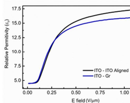
Figure 5 Relative permittivity vs applied E-field permittivity in BL006 LC filled ITO-ITO and ITO-Gr cells. E-field induced LC reorientation shows different alignment layer induced bulk response.
