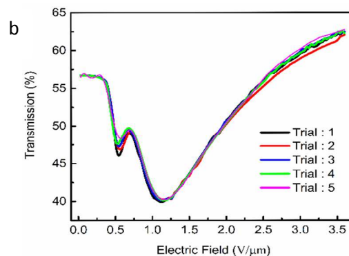
Figure 6 Transmission curves of a Gr-Gr cell filled with 10\mu\text{m} BL006 nematic LC, (a) the effect of applied electric field and frequency on the scattering characteristic of the test cell (b) repeated switching runs.
