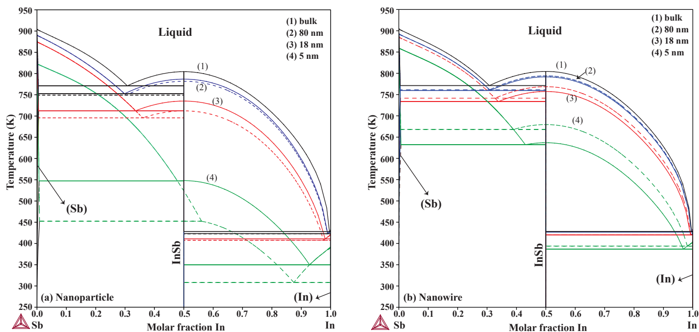
Fig. 4 The calculated phase diagram of bulk and of (a) nanoparticles and (b) nanowires for radius = 5, 18 and 80 nm. The solid lines are the calculated digram with the assumed relevant surface energy for InSb nanoparticles and nanowires, {111} and {110} surface energies, respectively. For comparison, phase diagrams for nanoparticles with {110} surface energy of InSb and for nanowires with {111} surface energy of InSb are also calculated and shown with dashed lines.
