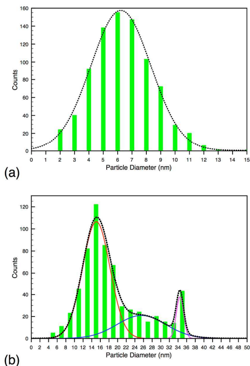
Figure 4. Particle size distributions in (a) Ag/PVA nanocomposite showing simple Gaussian distribution of silver nanoparticles and (b) Au/PVA showing a more complex distribution reflecting the different families of Au nanoparticles formed within the PVA host matrix.
