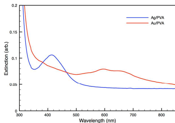
Figure 8. Extinction spectra for the Ag/PVA and Au/PVA nanocomposite materials. The silver doped nanocomposite shows a well-defined peak at \sim 415 nm whereas the gold doped material shows a broader, multi-modal peak centred around \sim 620 nm.
