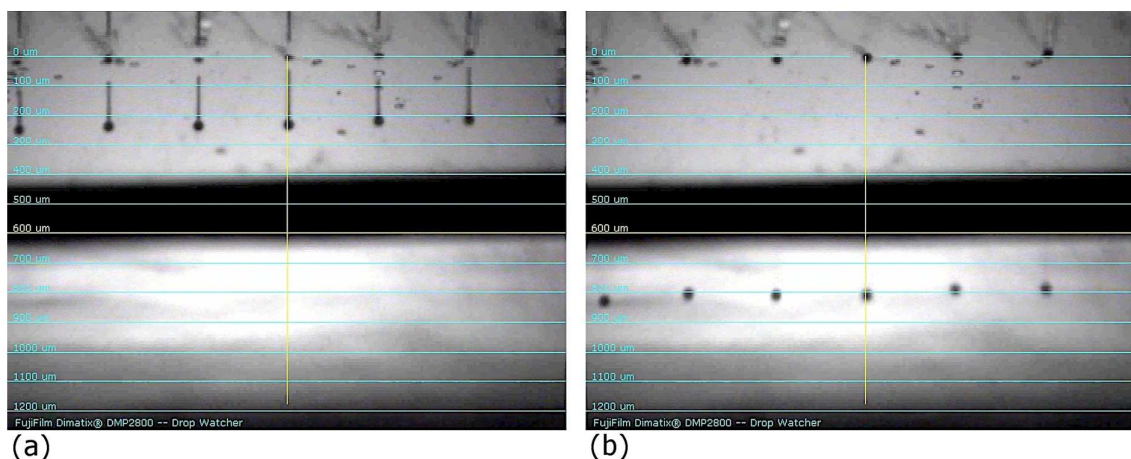
Figure 1. Droplet formation for printable PVA nanocomposite fluid. (a) Immediately after ejection from printer nozzles showing the short droplet “tails” with no satellite droplet structure for the optimised driver waveform. (b) Formation of well-behaved droplets after absorption of the “tail” into the main droplet body, well before impact with the substrate.
