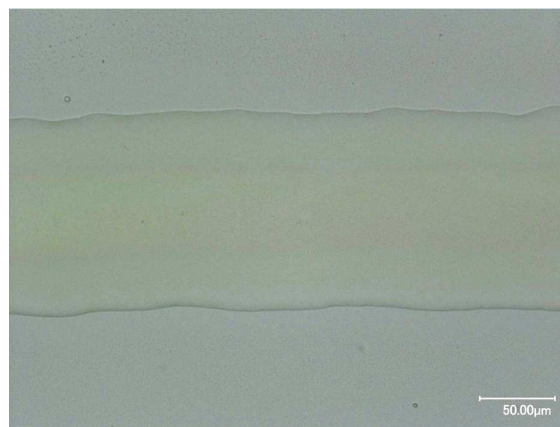
Figure 2. Optical micrograph of a printed Ag/PVA feature following thermal treatment to generate Ag nanoparticles. The yellow tint to the printed feature arises from the surface plasmon resonance behaviour of the embedded Ag nanoparticles. Good edge quality is achieved using optimised printing conditions.
