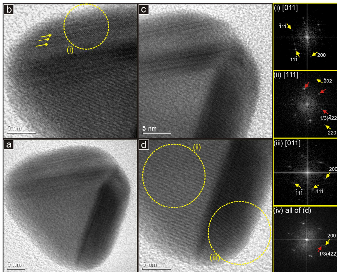
Figure 6. TEM images of a doubly-twinned Au particle showing: (a) the whole particle and (b,c,d) the three corners. Circles indicate regions from which DDPs (i) to (iv) have been obtained. Zone axes and Miller indices of the spots are given in the DDPs. The arrows in (b) indicate a series of plane defects. See text for further details.
