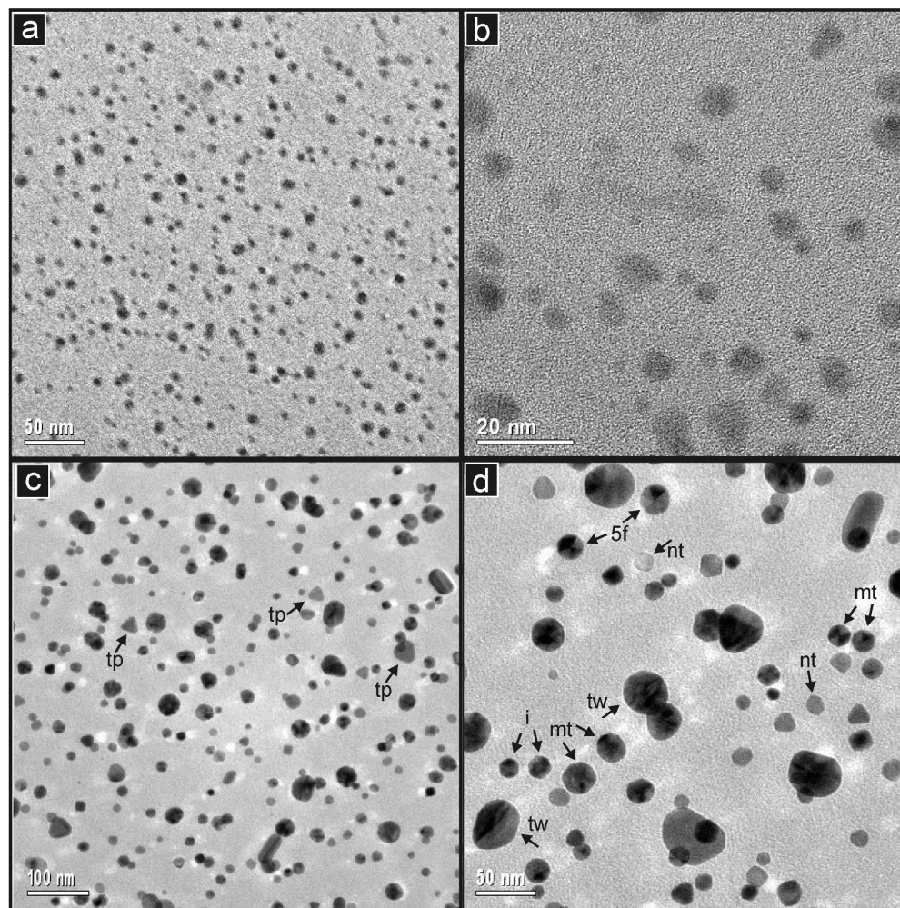
Figure 3. Low and intermediate magnification TEM images of the (a,b) Ag/PVA and (c,d) Au/PVA samples. See text for meanings of labels in (c) and (d).
