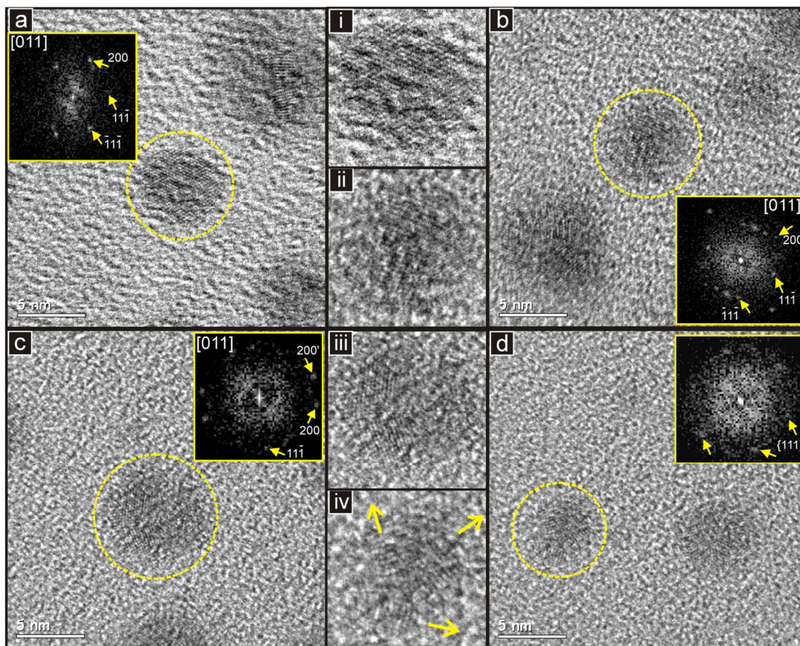
Figure 5. TEM images of four individual Ag particles with accompanying DDPs inset. Magnified views of the images in (a)-(d) are given in (i)-(iv), respectively. See text for details.
