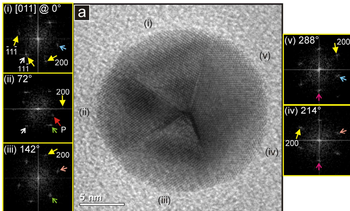
Figure 7. (a) TEM image of a multiply-twinned Au particle showing five-fold symmetry viewed down its major (C5) axis of symmetry. DDPS of each of the five visible crystal domains are presented as indicated on the image. These can all be indexed to the Au structure viewed along the [011] zone axis. All Miller planes are indicated in (i). In (ii)-(v) only the 200 planes are labelled. In the DDPS, the angles of rotation relating the patterns are given and small coloured arrows indicate {111} planes which are shared (i.e. continuous) between neighbouring domains. The extra spots marked P in (ii) are from an ordered region of the polymer near the edge of the particle.
