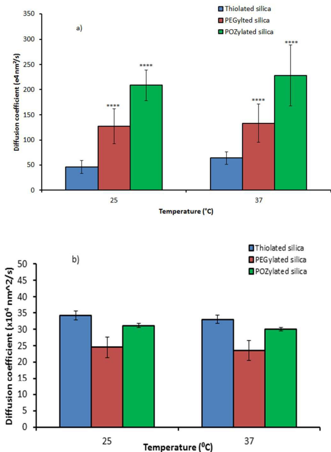
Figure 4. Experimentally determined diffusion coefficients (a), and calculated diffusion coefficients (b) of functionalised and unfunctionalised silica nanoparticles through 1% w/v gastric mucus. Data show the mean \pm standard deviation, where n=9 .
