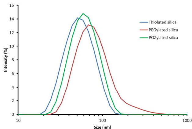
Figure 1. Dynamic Light Scattering size distributions of thiolated (blue), PEGylated (red) and POZylated (green) silica nanoparticles.
