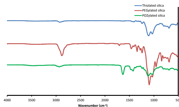
Figure 2. FTIR spectra for thiolated (blue), PEGylated (red), and POZylated (green) silica nanoparticles.
