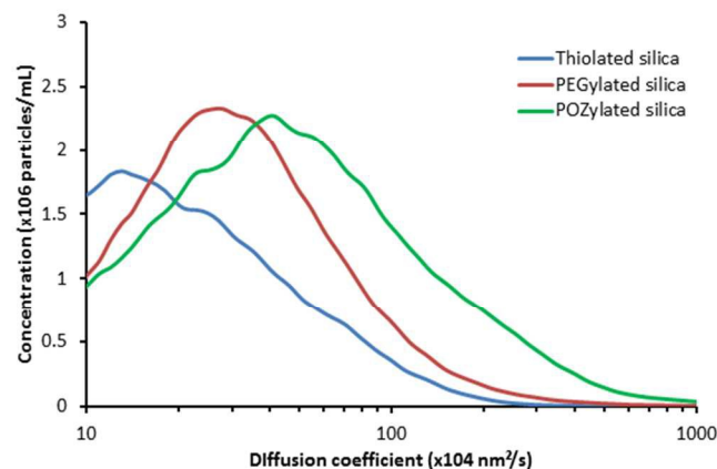
Figure 3. Distribution of diffusion coefficients for thiolated (blue), PEGylated (red) and POZylated (green) silica nanoparticles in 1% w/v gastric mucus at 37\text{ }^\circ\text{C} . Data represents the mean distributions, where n=9 .
