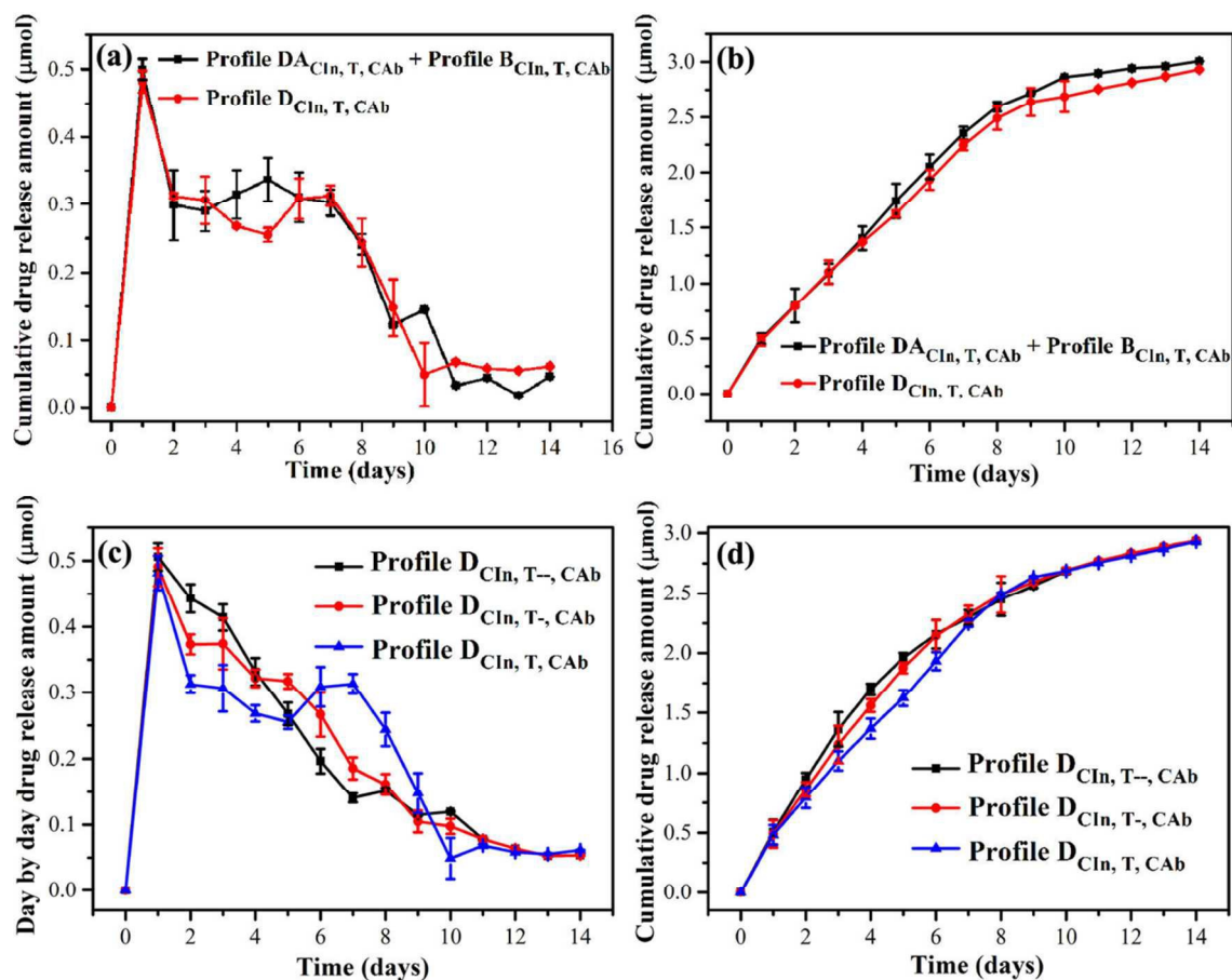
Fig. 5 (a) Day-by-day and (b) cumulative release profile of D_{\text{Cln}, T, \text{CAb}} profile compared to the summation of Profile DA_{\text{Cln}, T, \text{CAb}} + Profile B_{\text{Cln}, T, \text{CAb}} ( \text{Cln} \approx 2.2 \mu\text{mol} , \text{CAb} \approx 0.8 \mu\text{mol} , and T = 0.23 \text{ mL} ). (c) Day-by-day and (d) cumulative release profiles of BLM taken from three BLM-SiO 2 -BLM NP samples at the same BLM load amount ( \text{Cln} \approx 2.2 \mu\text{mol} , \text{CAb} \approx 0.8 \mu\text{mol} ) but different TEOS amount ( T = 0.15 \text{ mL} , T = 0.2 \text{ mL} , and T = 0.23 \text{ mL} ).
