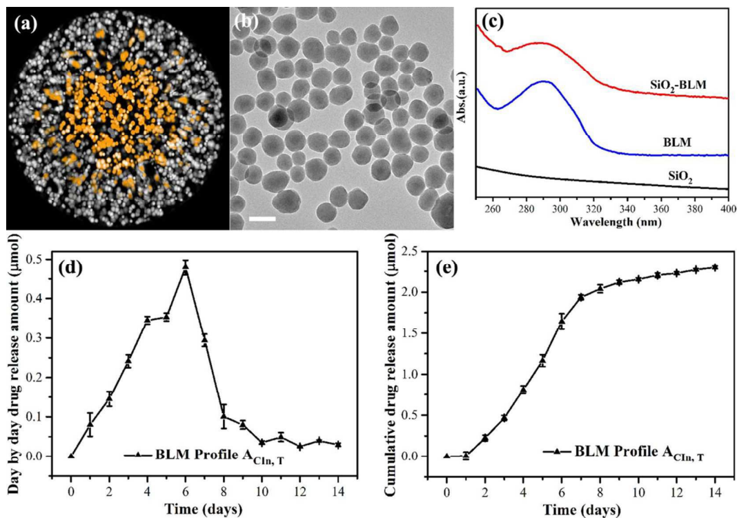
Fig. 3 (a) Illustration of the SiO 2 -BLM self-decomposable NP (A Model); (b) Low magnification TEM image of the as-synthesized SiO 2 -BLM NP (sample A Cl n , T ). The scale bar is 100 nm; (c) Optical absorption spectra taken from pure SiO 2 , pure BLM, and SiO 2 -BLM NPs; (d, e) Day-by-day and cumulative release profiles of BLM in deionized water from A Model NPs at 37 °C. The experimental data shown in this figure were obtained from the SiO 2 -BLM NP (sample A Cl n , T ) synthesized at TEOS amount of T= 0.23 mL, first-loaded (grown-in) BLM amount ~ 2.2 μmol.
