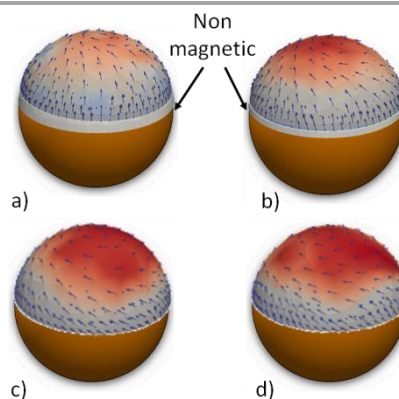
Figure 10 The magnetic moment configuration calculated by micromagnetic simulation for a) 28 Å, b) 38 Å, c) 42 Å and d) 72 Å evaporated iron thickness on 400 nm diameter spheres. The bluish color represents the magnitude of the Z component while the red stands for the X-Y in-plane component. The non magnetic part of the iron layer is shown with gray.
