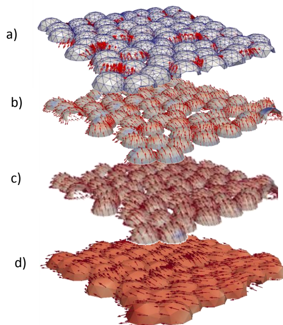
Figure 8 Magnetic moment configuration calculated by micromagnetic simulation for a) 26 Å, b) 34.5 Å, c) 48.5 Å and d) 70.5 Å evaporated iron thickness on 25 nm diameter spheres. The bluish color represents the magnitude of the Z component while the red stands for the X-Y in-plane component.
