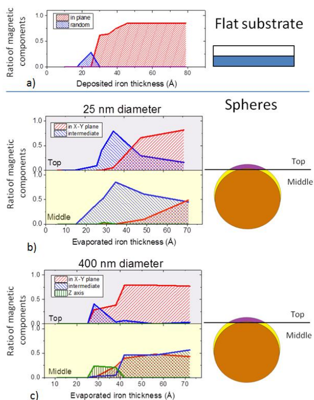
Figure 8 Evolution of the magnetic components orientation with increasing iron thickness of a) Flat substrate, b) 25 nm and c) 400 nm diameter silica spheres. The green line corresponds to the magnetic orientation parallel to the z direction, the red line corresponds to the magnetization lying in the x-y plane and the blue line corresponds to the intermediate magnetization direction. For the 25 nm and 400 nm particles the frame is divided into two parts representing the ratio of the magnetic components on the top of the sphere and on the middle of the sphere as it is indicated in the picture next to the frame
