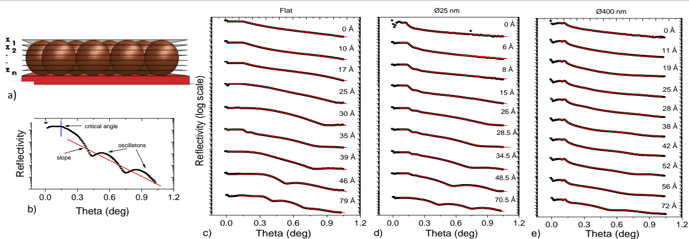
Figure 3 a) Division of the spherical particle template into sublayers b) A selected reflectivity curve and the definition of the key features such as critical angle, oscillations and the slope of the decay are marked. X-ray reflectivity curves of increasing iron layer thickness on flat silicon substrate (c) and on 25 nm (d) and 400 nm (e) diameter silica spheres (black points). The red line corresponds to the fitted data.
