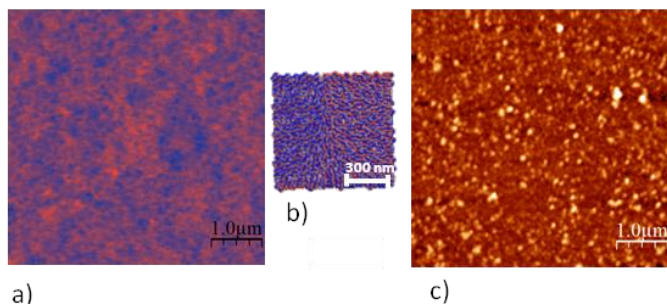
Figure 9 a) MFM image taken on 25 nm diameter nanospheres covered with \sim 70 Å iron and a 50 Å Nb capping layer. The magnetic tip was magnetized along the tip axis; hence the measurement was sensitive to the perpendicular component of the magnetization. b) The simulated magnetic orientation distribution in the Fe layer and c) the acquired topography image are shown.
