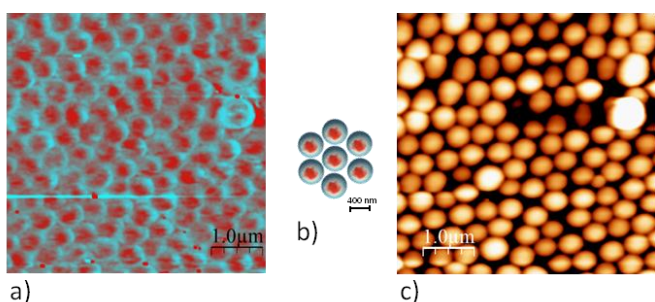
Figure 11 a) MFM image taken on ~70 Å thick iron layer evaporated on 400 nm spheres. The magnetic tip was magnetized along the tip axis, implying the measurement is sensitive to the perpendicular component of the magnetization. b) The simulated hexagonal structure and c) the AFM topography image
