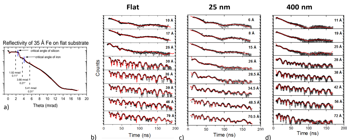
Figure 6 (a) X-ray reflectivity curve measured on 35 Å iron on flat substrate. Dashed lines represent the angles where timespectra were recorded and blue lines indicate the critical angle of silicon and iron. The red line corresponds to the simulated spectra Time resolved NFS spectra (black circles) measured at incident angle of 0.11^\circ after each iron deposition phase (b) on flat Si substrate (c) on 25 nm and (d) on 400 nm diameter spheres.
