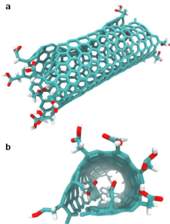
Figure 3. Self-assembly of a single, functionalised graphene nano-sheet to form a rolled tube with capped ends in vacuum (mimicking a non-polar solvent). The tube formation is facilitated by opposite electrostatic charges on the opposing edges. (a) View from the side. (b) View from one of the end showing two carboxylic acid chains partially blocking the tube.
