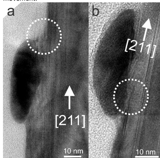
Figure 5. HRTEM image. (a) The highlights indicate missing regions along the nanowire sidewall. (b) The image shows a discontinued stacking fault, as indicated by the highlights.
