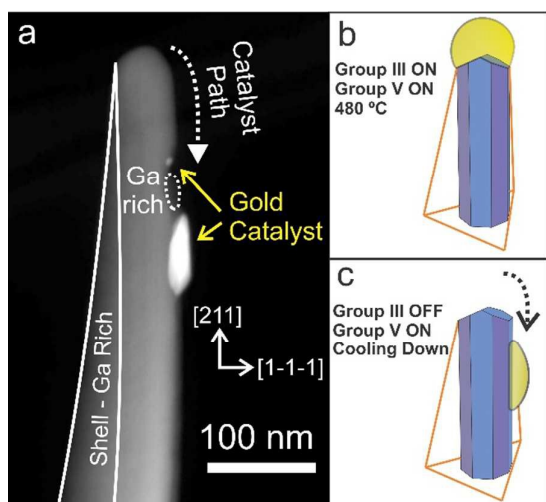
Figure 4. (a) HAADF image of a nanowire apex. (b) Schematics of the catalyst position during growth. (c) Schematics of the catalyst movement and final position during cool down.
