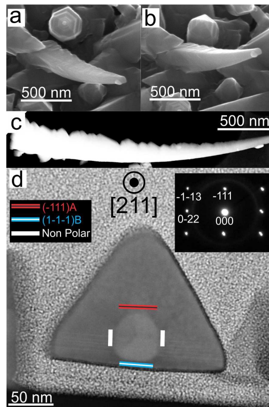
Figure 1.(a,b)SEM image of as-grown nanowires; the sample was tilted by 30° between images. (c) ADF-STEM lateral view of a triangular NW. (d) TEM image of the cross section of a nanowire grown in the [211] direction (see electron diffraction pattern in the inset).
