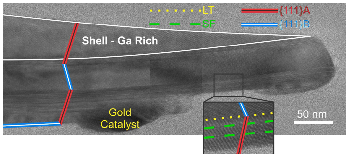
Figure 3. Mosaic of nanowire HRTEM images. \{111\} facets with different polarities are enabled by lamellar twins, as indicated in the figure inset. Most of the stacking faults cross the \{111\} A facet.
