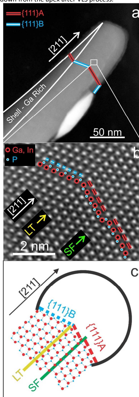
Figure 2. (a) High angle annular dark field (HAADF) image of a nanowire; the polarity of the {111} facets have been determined by direct measurement of the dumbbells. (b) FFT filtered image of a HAADF image of the region indicated in (a), which show the presence of LTs and SFs. (c) Schematics of the interface between the catalyst and the nanowire during growth.
