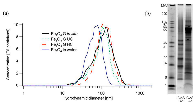
Fig. 7 Fe 3 O 4 NPs in simulated gastric fluid. a) Size distributions obtained from NTA analysis for Fe 3 O 4 NPs incubated with gastric fluids and relative hard coronas isolated by ultracentrifugation (UC) and centrifugation (HC). b) SDS-PAGE of the hard corona samples isolated by ultracentrifugation (UC) and conventional centrifugation (HC) methods, respectively, as indicated by the labels below the tracks of the gel.
