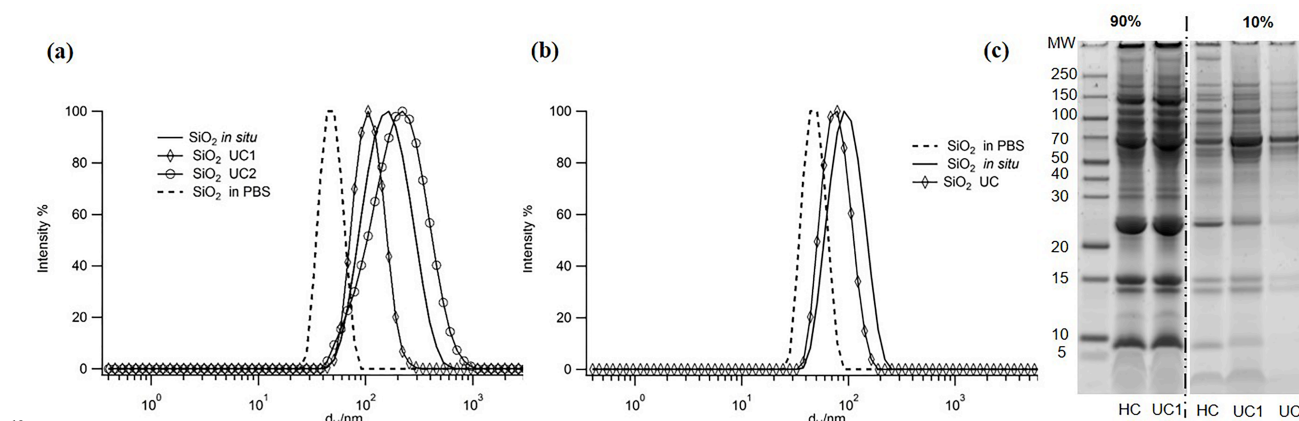
Fig. 4 Characterization of SiO 2 NPs. In graph a) and b) are reported size distributions by intensity percentage of SiO 2 NPs in 10% and 90% FBS respectively, compared to NPs in PBS (dashed line). c) SDS-PAGE gel of the hard corona complexes of SiO 2 NPs in 10% and 90% FBS isolated by ultracentrifugation (UC) and conventional centrifugation methods (HC), respectively, as indicated by the labels below the tracks of the gel.
