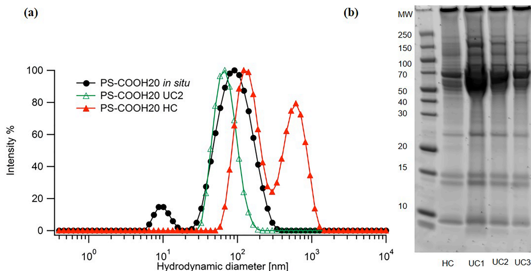
Fig. 2 HC complexes of PS-COOH20 in 90% FBS. a) Size distribution by intensity percentage of NPs in situ (black dots), HC complexes isolated by centrifugation (HC, red triangles) and ultracentrifugation (UC2, green empty triangles). b) SDS-PAGE gel of the complexes in 90% FBS isolated by conventional centrifugation methods (hard corona, HC) and ultracentrifuge (UC1-2), respectively, as indicated by the label below the tracks of the gel.
