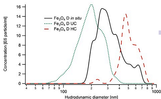
Fig. 8 Fe 3 O 4 NPs in simulated intestinal fluid. Size distributions obtained from NTA analysis for Fe 3 O 4 NPs incubated with intestinal fluids for one hour and relative hard coronas isolated by ultracentrifugation (UC) and centrifugation (HC).
