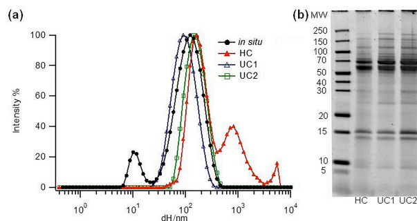
Fig. 5 Fe 3 O 4 in 55% FBS. a) Size distributions from DLS measures of Fe 3 O 4 NPS in situ and HC complexes recovered by ultracentrifugation (UC1-2) and by centrifugal washings (HC) b) SDS-PAGE of hard corona complexes isolated by conventional centrifugation (HC) and by density gradient ultracentrifugation (UC1-2).
