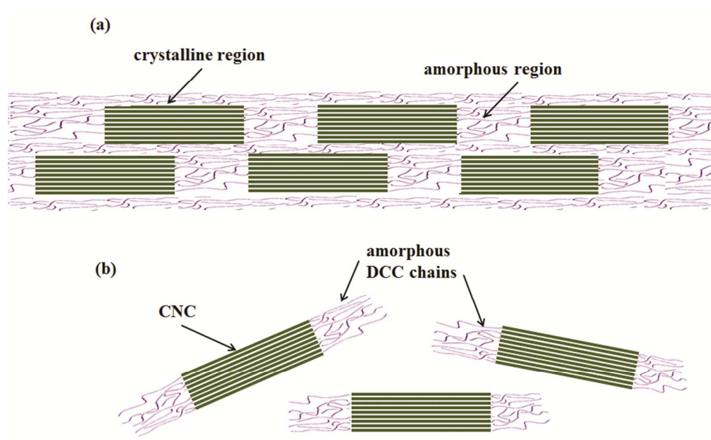
Scheme S1. Schematic presentation of (a) CNC packed inside a cellulose micro-fibril, and (b) CNCs separated via the double oxidation process.
