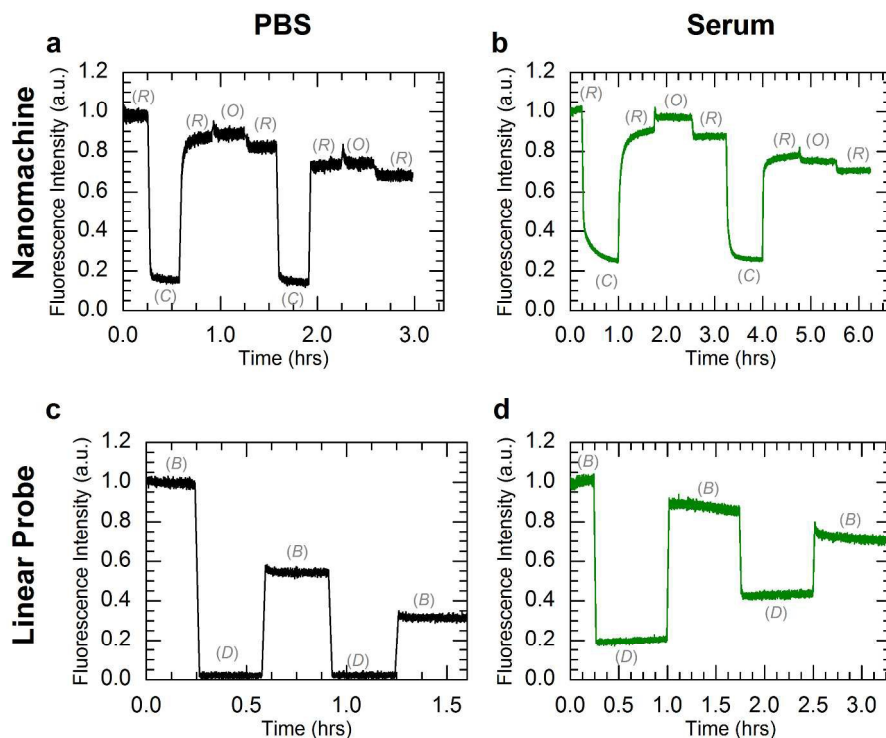
Fig. 4. Kinetics data for operation of the three-state nanomachine and two-state linear probe at 37 °C. Both systems were operated in PBS (a,c) and human serum (b,d) through two complete cycles. The fluorescence data were normalized to the initial state intensities. The mechanical states of the nanomachine are Relaxed (R), Closed (C), and Open (O). The mechanical states of the linear probe are Bright (B) and Dark (D). Nanomachine data (a,b) include ~10% fluorescence offsets from excess A in solution. The observed overall decreases in fluorescence for the Relaxed state of the nanomachine and the Bright state of the linear probe are attributed to dilutions from fuel injections. (a) Operation of the nanomachine in PBS shows state transitions similar to 25 °C, but with unstable fluorescence in the Open state. (b) In serum, clear state transitions were observed for the first complete cycle, yet the Open state transition failed during the second cycle. Operation was arbitrarily terminated after two complete cycles. (c) Operation of the linear probe in PBS is consistent with results seen at 25 °C. (d) In human serum, the linear probe displayed a continuous increase in Dark state fluorescence, which is attributed to enzymatic degradation.
