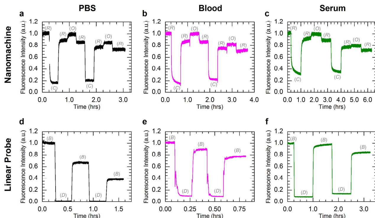
Fig. 3. Kinetics data for operation of the three-state nanomachine and two-state linear probe. Both systems were operated in PBS (a,d), heparinized whole human blood (b,e), and human serum (c,f) through two complete cycles at 25 °C. The fluorescence data were normalized to the initial state intensities. The mechanical states of the nanomachine are Relaxed (R), Closed (C), and Open (O). The mechanical states of the linear probe are Bright (B) and Dark (D). Nanomachine data (a-c) include ~10% fluorescence offsets from excess A in solution. Aside from the Cy5.5-IBRQ interaction in the linear probe in PBS (d, see main text), the observed overall decreases in fluorescence for the Relaxed state of the nanomachine and the Bright state of the linear probe are attributed to dilutions from fuel injections. Stable operation was observed for both systems in all three solutions.
