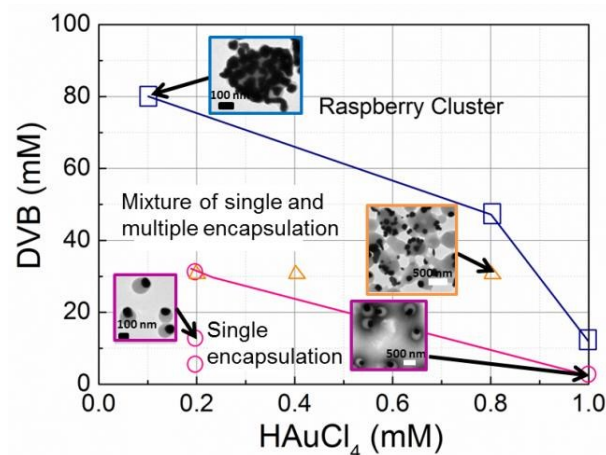
Fig. 2. The product diagram of hybrid nanoparticles under different concentrations of DVB and HAuCl 4 . □ Au raspberry clusters, △ mixture of Au-PDVB nanoparticles with single and multiple Au components, ○ Au-PDVB Janus particles. The reactions are taking place under 45 °C.
