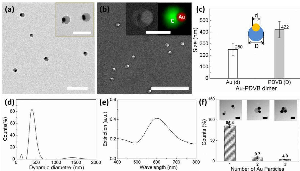
Fig. 1. Asymmetric hybrid nanoparticles synthesized under 0.2 mM HAuCl 4 and 32 mM DVB. (a) TEM image, scale bar is 2 μm and 1 μm in the inset, (b) SEM image with inset of EDX mapping. Scale bars are 5 μm and 500 nm in the inset, (c) is the statistic measurement of the sizes of the hybrid nanoparticles, (d) is the dynamic light scattering measurement of the hybrid nanoparticles in aqueous dispersion (number average), (e) is the UV-Vis spectra of the hybrid nanoparticles, (f) is the purity and the yield of the hybrid particles with different morphologies, all the scale bars in the insets are 100 nm.
