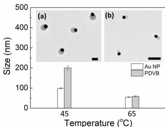
Fig. 3. Sizes of Au and PDVB components obtained at different temperatures. Insets are TEM images of asymmetric Au-PDVB hybrid nanoparticles synthesized at (a) 45 °C and (b) 65 °C. Scale bars are 200 nm.
