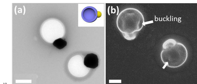
Fig. 5. (a) TEM and (b) SEM images of Au-PS Janus nanoparticles obtained using Styrene as the monomer. Inset is the scheme representing Au-PS hollow shell Janus hybrid nanoparticles. Scale bars are 200 nm.
