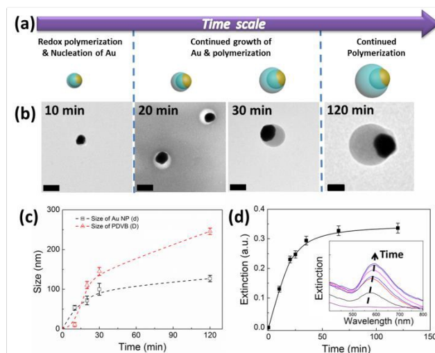
Fig. 4. Kinetics of growth of hybrid nanoparticles. (a) Scheme and (b) typical TEM images at different times, all scale bars are 100 nm. (c) Size changes of components of Au and PDVB with time. (d) Growth kinetics of Au component monitored with UV-Vis spectroscopy.
